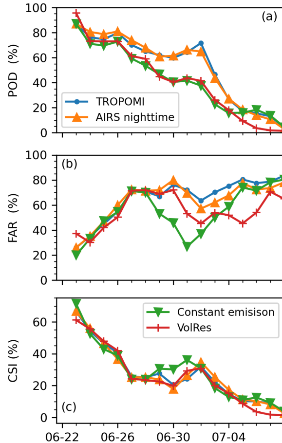
Figure 14. Time series of POD (a), FAR (b), and CSI (c) for forward simulations initialized by a constant injection rate (green) and the VolRes profile (red) as well as injection parameters reconstructed using TROPOMI (blue) and AIRS nighttime data (orange), respectively. The reference observations are TROPOMI observations retrievals. Color coding indicates the The column density threshold used to detect events (see plot key) is 5.0 DU.
