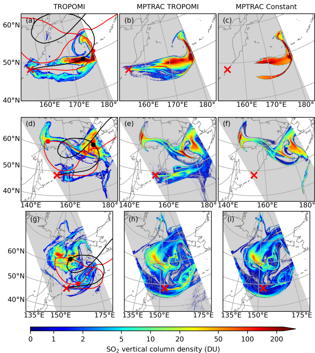
Figure 11. TROPOMI observations-retrievals and MPTRAC forward simulations of SO 2 transport. Top row (a-c): spatial distribution of SO 2 vertical column density (DU) from the TROPOMI orbit that starts at 23 June 2019, 01:05 UTC and ends at 23 June 2019, 02:47 UTC (a), and the corresponding distribution in forward simulations, which were initialized by TROPOMI observations-retrievals (b) and by a constant injection rate (c), respectively. Middle and bottom rows show the same as the top row but for the orbits of 25 June 2019, 00:27-02:09 UTC and 28 June 2019, 01:12-02:53 UTC, respectively. The mean trajectories for injections between 7-87-8 km (red curve) and 11-1511-15 km (black curves) are plotted on the maps on the left, and the mean locations at the corresponding time of each map are indicated by red and black dots.
