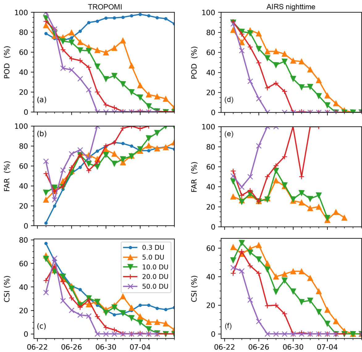
Figure 13. Time-Left panel (a–c): time series of the probability of detection (POD; a), false alarm rate (FAR; b), and critical success index (CSI; ac) for a forward simulation initialized by the reconstructed injection parameter based on TROPOMI data. The TROPOMI observations retrievals are used as reference observations. Subplots in the right panel (d–f) are the same as the left panel, but for AIRS nighttime data and the reference observations are also from the AIRS nighttime data. Color coding indicates the column density threshold used to detect events (see plot key).
