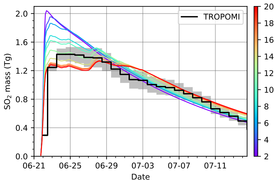
Figure 8. Temporal change of SO 2 total mass in MPTRAC forward simulations, which were initialized by considering different numbers of days of TROPOMI observations retrievals since the beginning of the Raikoke eruption (see color bar). Total mass of SO 2 injection in all simulation-simulations is 2.1 Tg. In the forward simulations, the mass is derived from the chemistry module. The mass changes measured by TROPOMI are shown by the black line and gray shading indicates the measurement errors.
