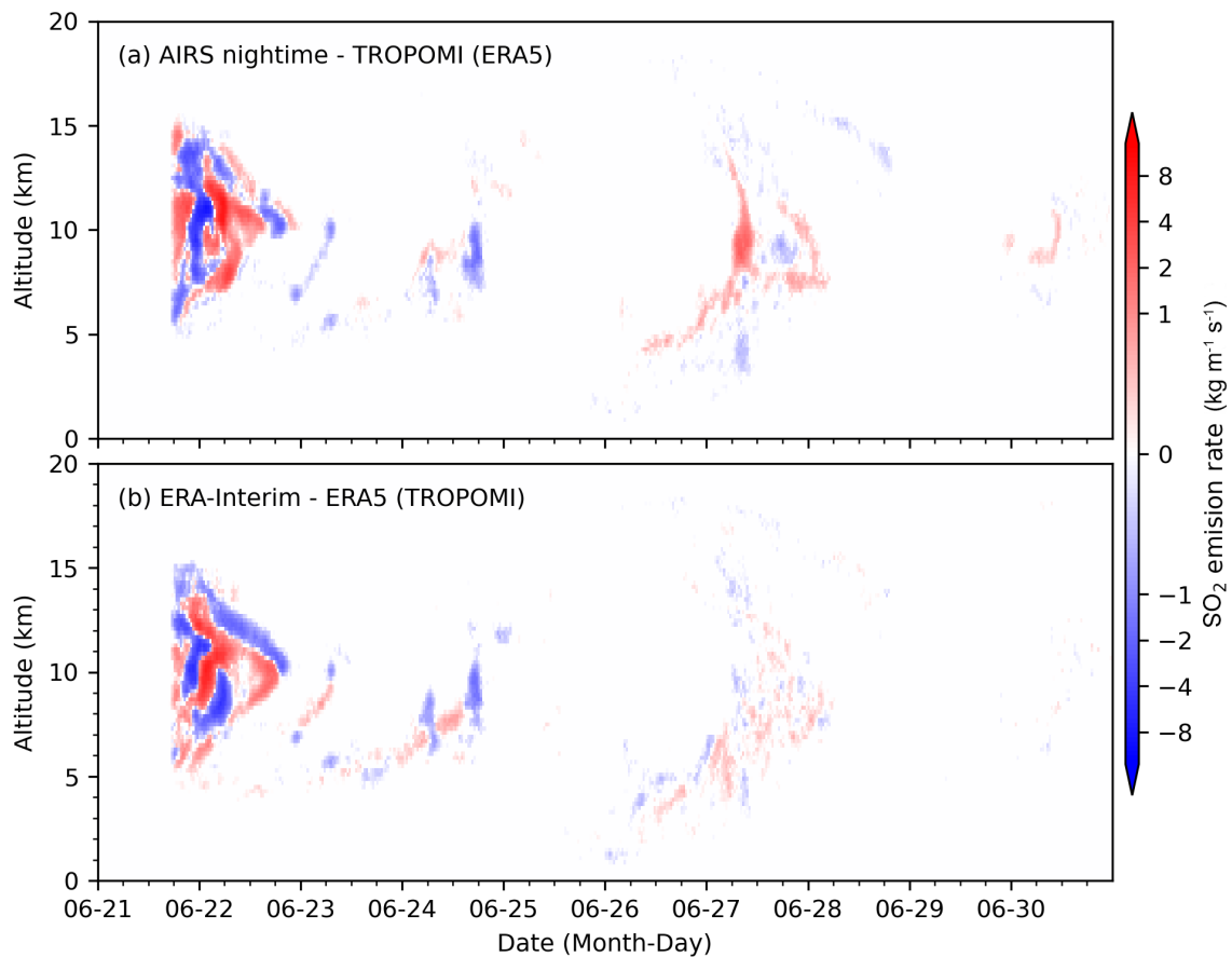
Figure 7. Differences of in reconstructed SO 2 injections of the 2019 Raikoke eruption derived from different combinations of satellite observations retrievals and reanalysis data compared with the TROPOMI-ERA5 combination: AIRS nighttime with ERA5 (a), and TROPOMI TROPOMI with ERA-Interim (b).
