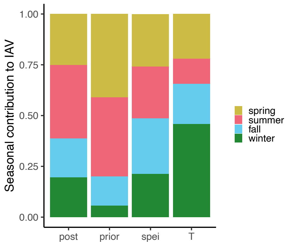
660 Figure 10: Seasonal contribution to IAV calculated relative to 14 years for posterior NEE fluxes (post), VPRM NEE fluxes (prior), SPEI, and T during the four seasons over the full domain.
