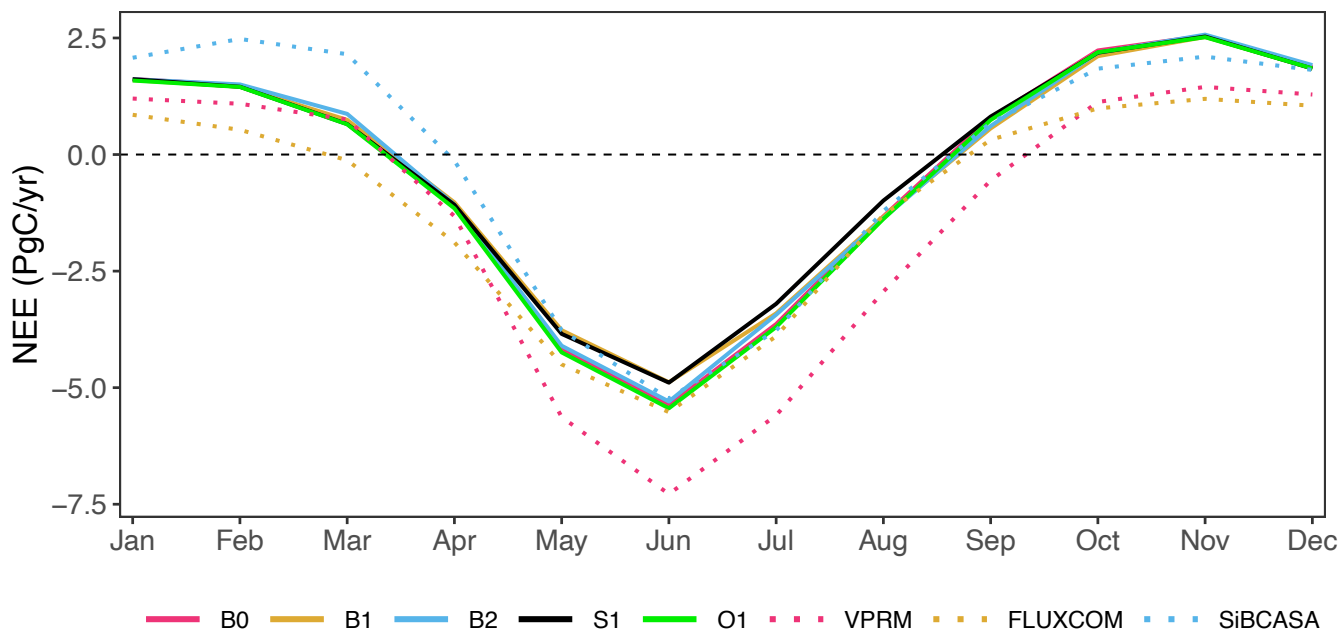
635 Figure 4: Seasonal cycle of NEE calculated as the average of monthly fluxes over 13-year estimated using the ensembles of inversions (solid lines) B0, B1, B2, S1, O1, as well as the biogenic prior fluxes (dotted lines) obtained from VPRM, FLUXCOM, and SiBCASA.
