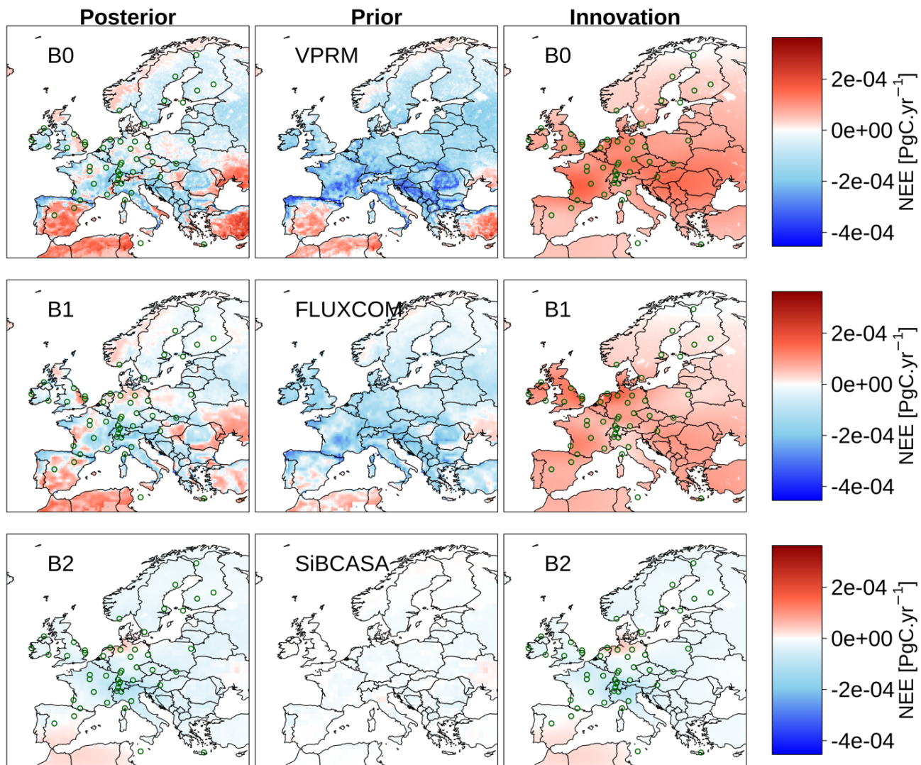
645 Figure 7: Posterior, prior, and innovation of fluxes (posterior - prior) averaged over the 2006-2018 period calculated from the biosphere ensemble of inversions (B0, B1 and B2). Green circles refer to observing sites.
