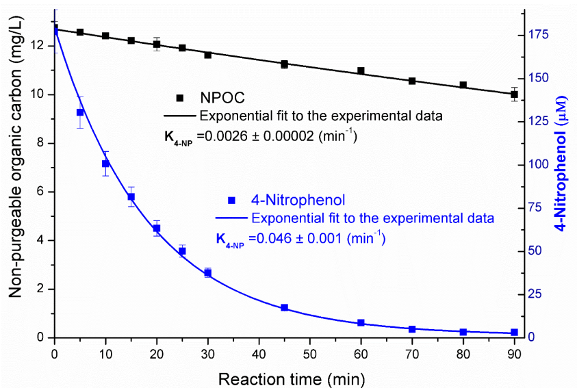
Figure 7: The concentrations of 4NP and non-purgeable organic carbon during the reaction in pure water (the results obtained for pH=2 and 9 reaction solutions were very similar – section S11, S12). The uncertainties for the first-order decay rates ( K , \text{min}^{-1} ) are standard errors from the regression analysis.
