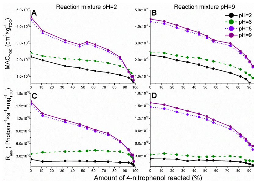
Figure 5: The pH-dependent organic carbon-normalized mass absorption coefficients (MAC TOC ) derived using the integrated absorbance peak for the reaction mixture absorption measured for the reaction of 4NP (A, pH=2) and 4NPT (B, pH=9) and the corresponding TOC-normalized rates of sunlight absorption (R abs ) for 4NP (C) and 4NPT (D). Only the data for pH =2, 6, 8, 9 are shown for clarity and the complete data are presented in Fig. S4S12. The colors refer to the pH at which the absorbance was measured (section 2.4). The experimental data are represented by points, with the lines provided to guide the eye.
