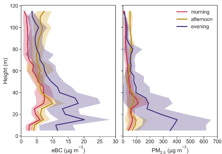
485 Figure 6: Mean vertical eBC and PM 2.5 profiles with standard deviation (shaded area) during morning (6:30–8:30 LT, red line), afternoon (12:00–14:00 LT, yellow line) and evening (17:00–19:00 LT, purple line) winter-time temperature inversions over the Retje hollow.
