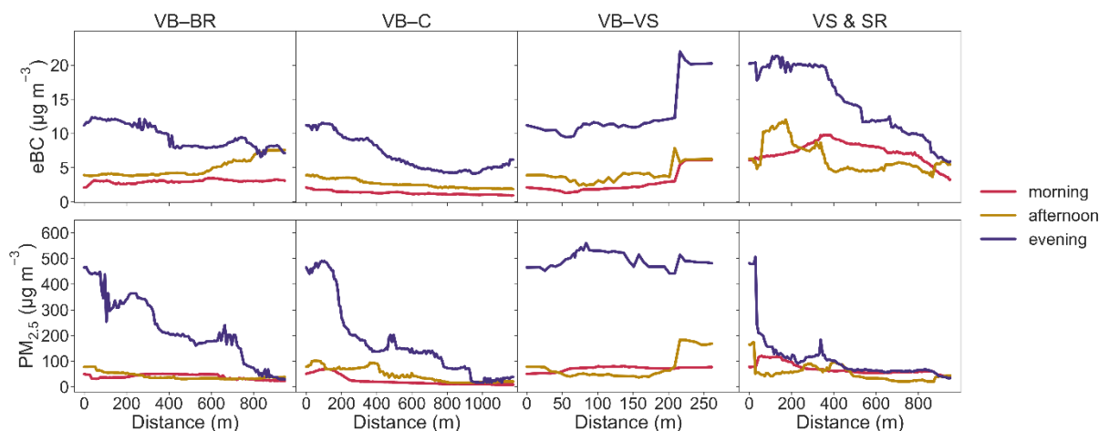
455 Figure 4: Variability of eBC (top panels) and PM 2.5 (bottom panels) mass concentrations during morning (6:30–8:30 LT, red line), afternoon (12.00:14.00 LT, yellow line) and evening (17:00–19:00 LT, purple line) winter-time temperature inversion along different parts of the fixed route in the Retje hollow.
