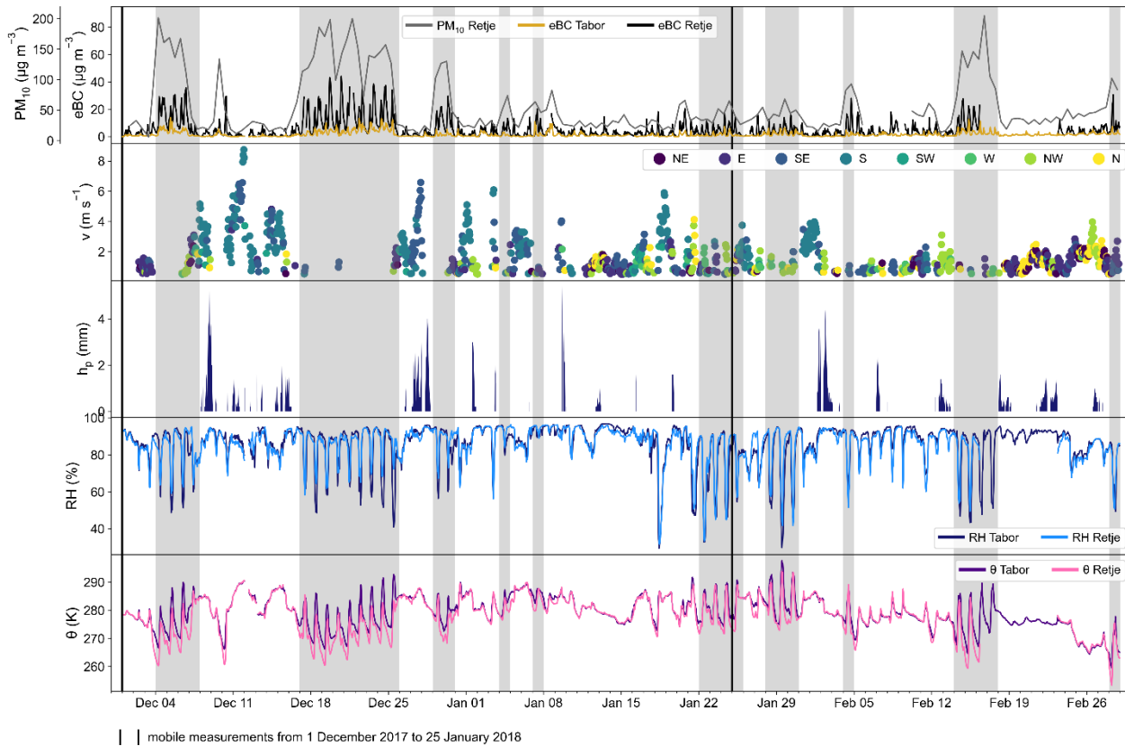
340 Figure 2: Time series of meteorological and air quality data for winter period (December 1, 2017–March 1, 2018): the 12-hour PM 10 mass concentrations at Retje, the hourly mean eBC mass concentrations at Retje and Tabor, wind speed (v) and direction at Hrib, precipitation (h p ) at Hrib, relative humidity (RH) and potential temperature (θ) at Retje and Tabor. The shaded areas represent temperature inversion periods.
