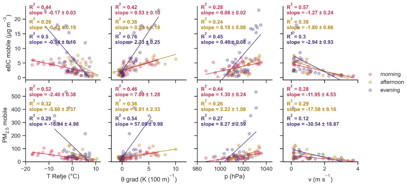
645 Figure 8: Linear correlations between the temperature measured at the Retje station (T Retje), potential temperature gradient ( \theta grad), atmospheric pressure (p) and wind speed measured at the Hrib (v) with mobile eBC and PM 2.5 mass concentrations inside the cold air pool (CAP).
