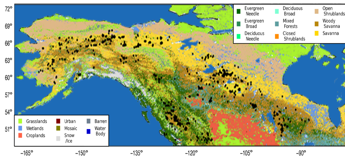
Figure 1. Map of all plumes used in this study (black dots) overlaid on the 2017 MODIS IGBP land cover types.
