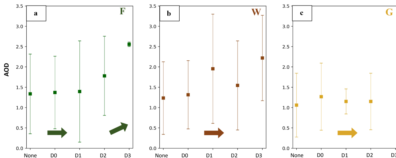
Figure 8. Median plume AOD according to plume type and drought level. Panels are color-coded by plume type and identified with the appropriate abbreviation in the top right-hand corner. Points represent the mean values, and whiskers are the standard deviations. Arrows highlight the general trends with increasing drought: up arrows signify that the trend is statistically significant, and flat arrows indicate that they are not. Note that AOD begins to increase with increasing drought level from D2 onward for forest plumes; for woody plumes, the differences in AOD are only significant when comparing the “None” category to the D3 category, with no clear trend in intermediate categories; for grassy plumes, there are no statistically significant relationships between AOD and drought severity.
