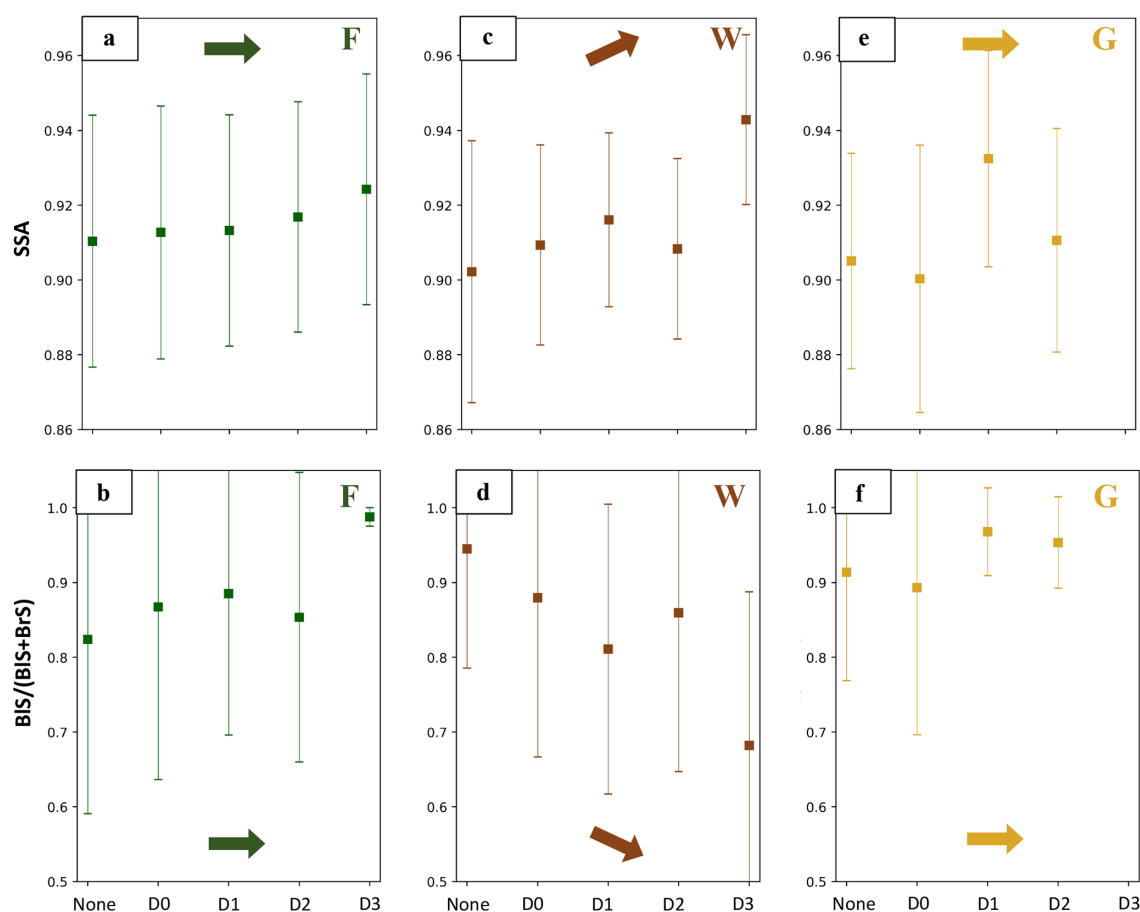
Figure 9. MISR mid-visible single-scattering albedo (a, c, e) and the fraction of AOD from BIS vs. the sum of both BIS and BrS (b, d, f) for different drought conditions. Decreasing values indicate lower amounts of BrS and higher amounts of BIS. Panels are color-coded by plume type and identified with the appropriate abbreviation in the top right-hand corner. Points represent the mean, and whiskers are the standard deviations. Arrows help highlight the general trends with increasing drought index: up or down arrows signify that the trends are statistically significant, and flat arrows indicate that they are not. Note that the D2 category presents an outlier for the otherwise clear trends in SSA and BIS / (BIS + BrS) for woody plumes; for F and G plumes, there is no statistically significant response to increasing drought severity for either variable.
