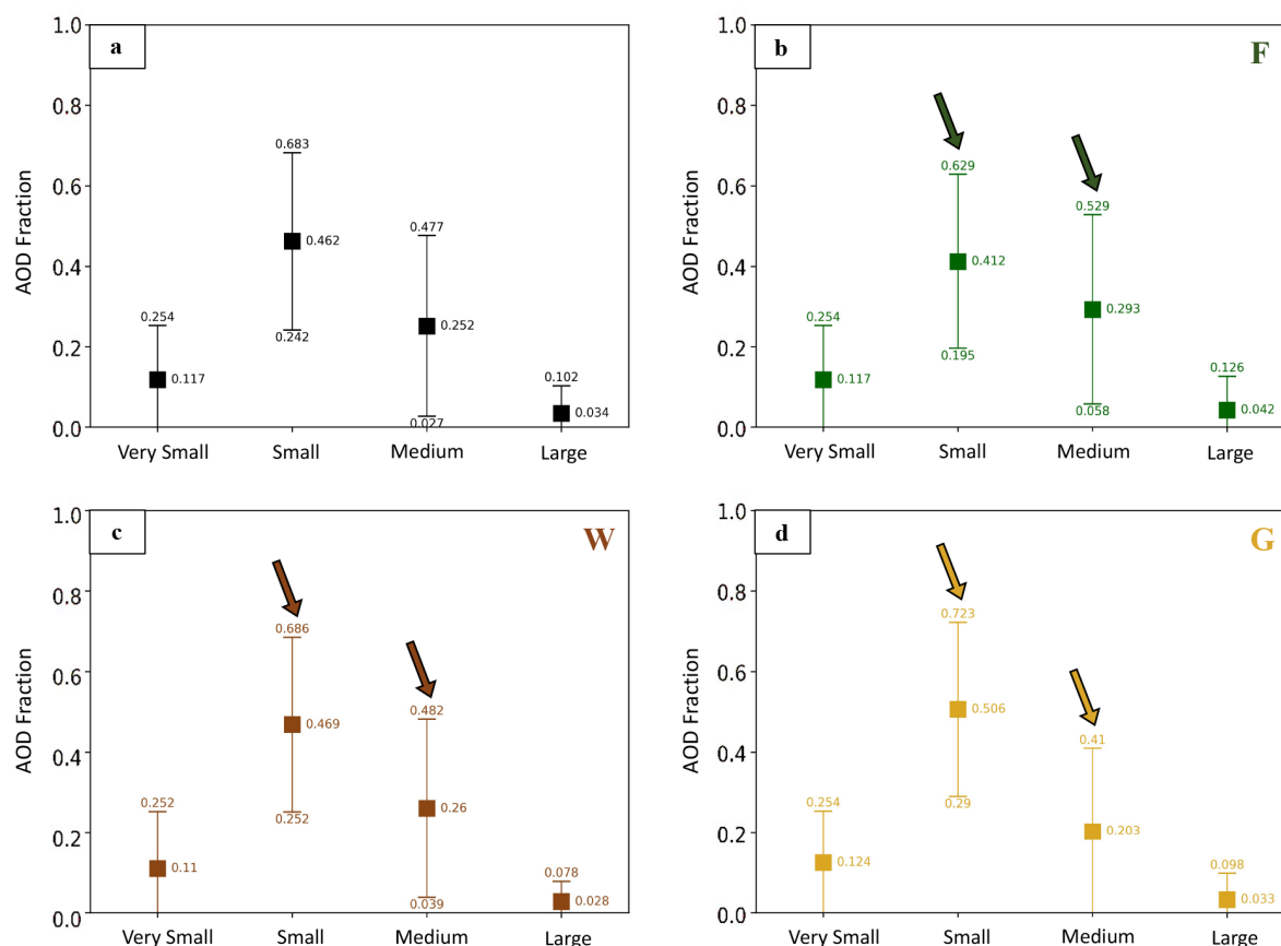
Figure 3. Particle size distributions in terms of each RA component's fractional contribution to the total AOD. All plume types are shown in panel (a), whereas panels (b)–(d) display color-coded results for individual plume types, denoted with the appropriate abbreviation in the upper right-hand corner. Points represent the mean values, and whiskers show the standard deviations. Arrows highlight the differences in the partitioning between the small and medium particle fractions for the different plume types.
