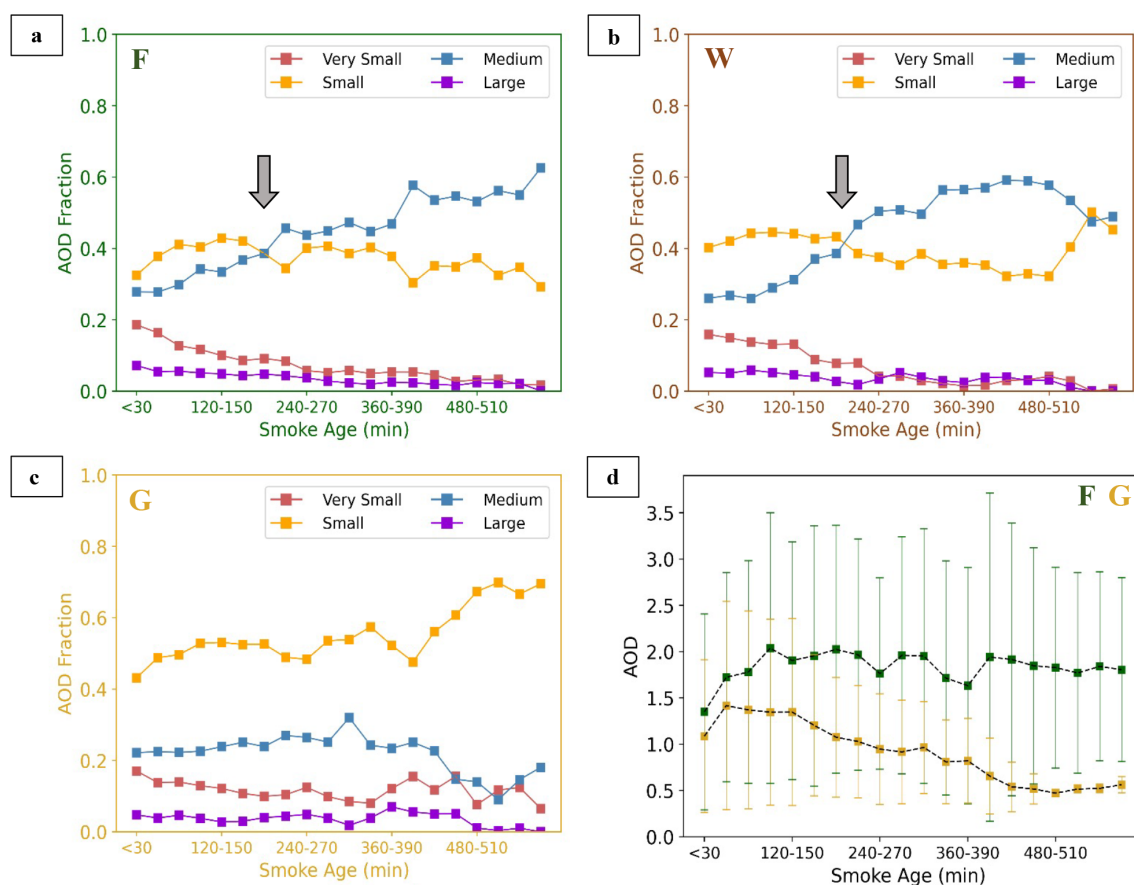
Figure 5. MISR particle-size component AOD fractions (in terms of the contribution to the total AOD, from 0 to 1) by smoke age for (a) forest plumes, (b) woody plumes, and (c) grassy plumes. In panel (d), the MISR mid-visible AOD is plotted by age for forest and grassy plumes, for reference. The points represent the mean values, and the whiskers are standard deviations. Arrows help highlight the points of important particle-size transitions.
