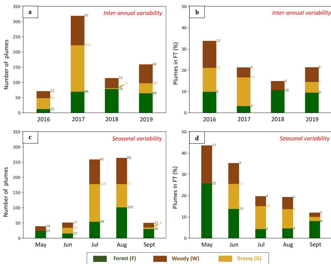
Figure 2. Seasonal and inter-annual variability in the plume number ( a , c ) and the percentage of those plumes in the free troposphere (FT) ( b , d ). Each bar is divided by color according to the relative contribution from each of the three fire types in the given month or year, with quantitative annotations. For example, 39 plumes were identified in the month of May ( c ), 16 of which were W fires and 23 of which were F fires. Of the 39 fires that month, ~42 % were in the FT (~17 % classified at W fires, and ~25 % classified as F fires) ( d ). Note that differences in rounding (for the sake of simpler visualization here) produce slightly different numbers compared with the percentage of plumes in the FT given in Table 2. A plume is considered to be in the FT if its median height is 100 m greater than the PBL height as defined in the MERRA-2 dataset.
