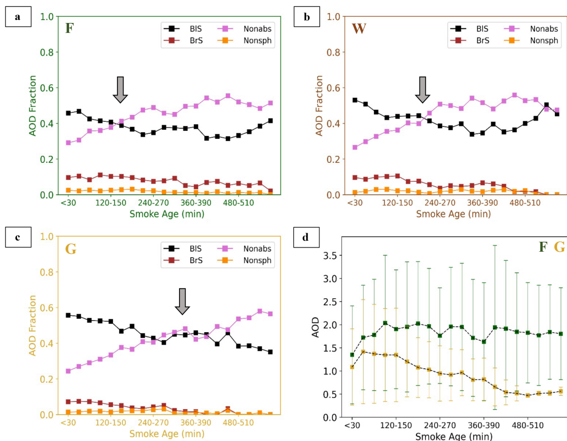
Figure 6. MISR particle-type component AOD fractions (in terms of the contribution to the total AOD, from 0 to 1) by smoke age for (a) forest plumes, (b) woody plumes, and (c) grassy plumes. In panel (d), the MISR mid-visible AOD is plotted by age for forest and grassy plumes, for reference. The points represent the mean values, and the whiskers are standard deviations. Arrows help highlight the points of important particle-size transitions. TS18
