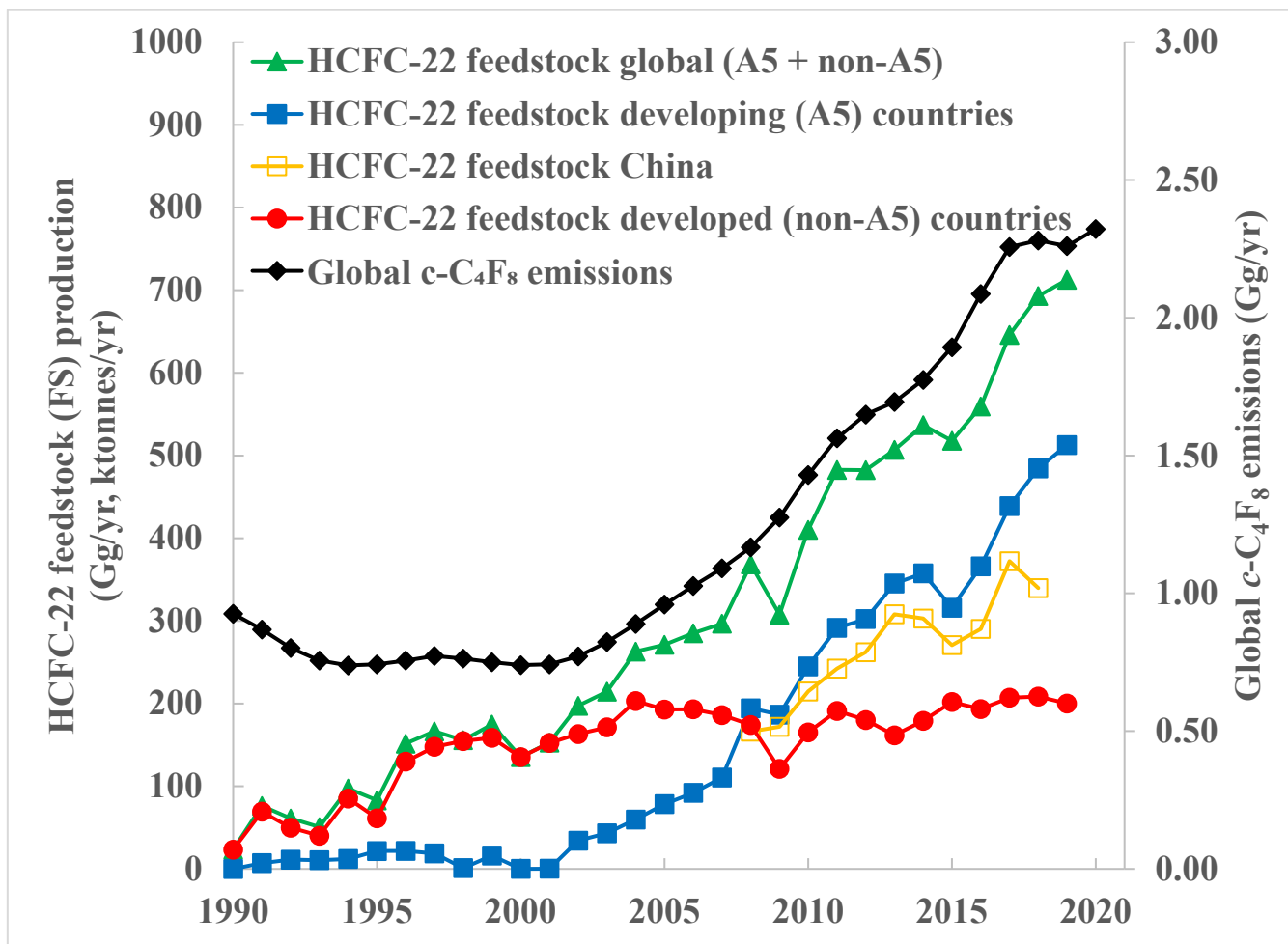
Figure 2 HCFC-22 feedstock (FS) production ( \text{Gg yr}^{-1} ). Global HCFC-22 FS production (green triangles) is the sum of HCFC-22 FS production in non-A5 (developed, red circles) and A5 (developing, blue squares) countries. Since about 2002, the increasing trend of global HCFC-22 FS production is dominated by growth in A5 countries, particularly China (orange open squares), while HCFC-22 FS production in non-A5 countries has been relatively stable.
