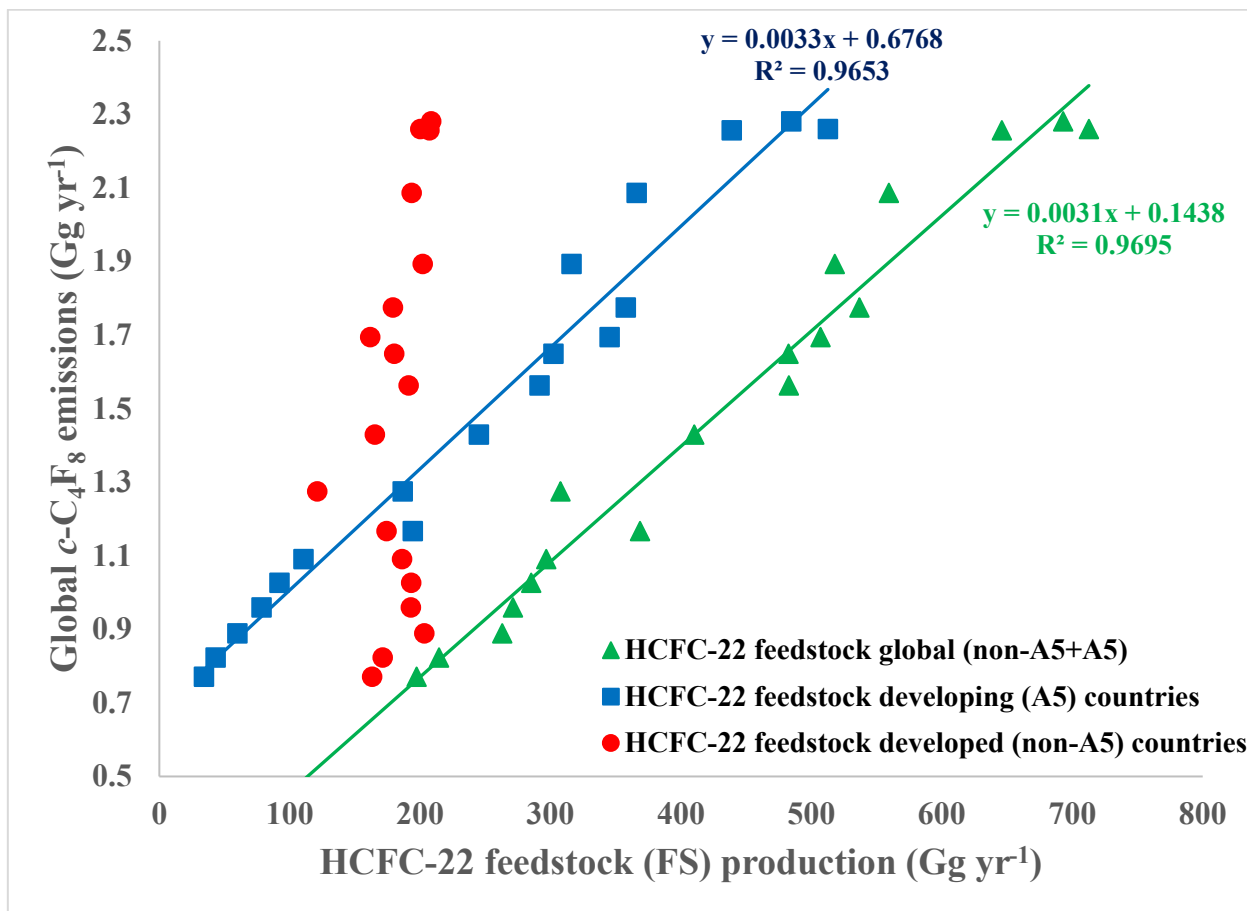
165 Figure 3 The relationship between A5 (developing, blue squares), non-A5 (developed, red circles) countries and total global HCFC-22 feedstock (FS, green triangles) production and global c -C 4 F 8 (PFC-318) emissions (2002-2019).
