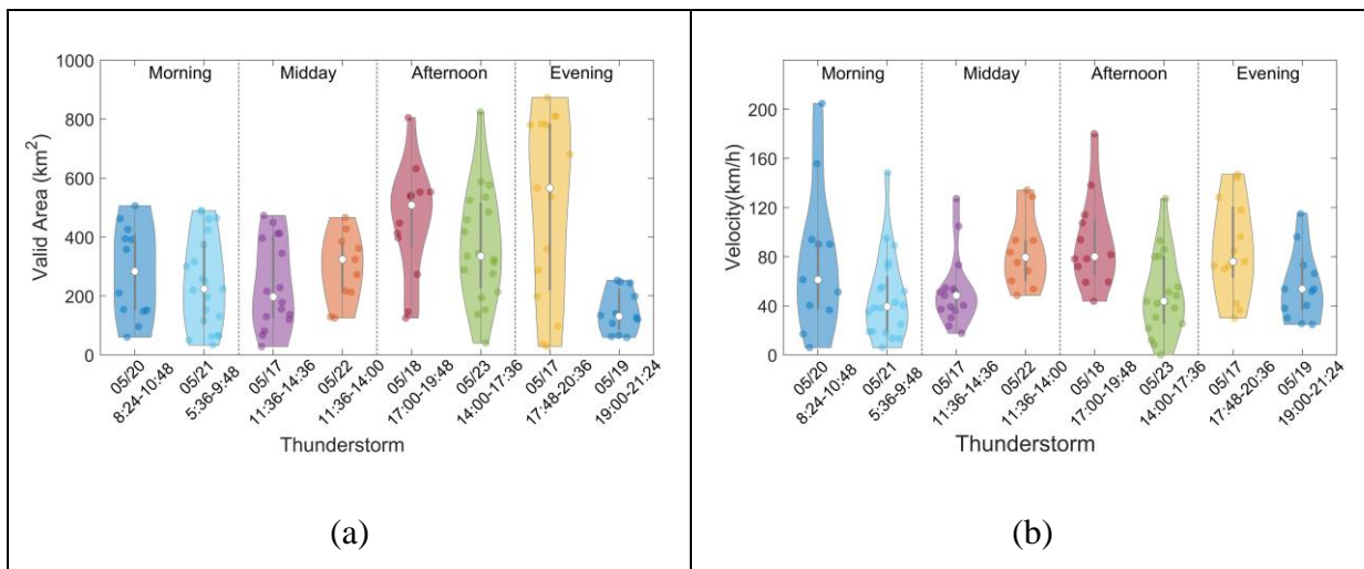
515 Figure 7. (a) Comparison of the valid area between eight cases. The upper and lower edges of boxes mean the maximum and minimum values. The white circle in each box represents the median of VA. The filled circles with a darker color than the box represent all VA values of thunderstorms. The grey vertical line in the box represents the interquartile range of VA. (b) Same as (a), but for the velocity.
