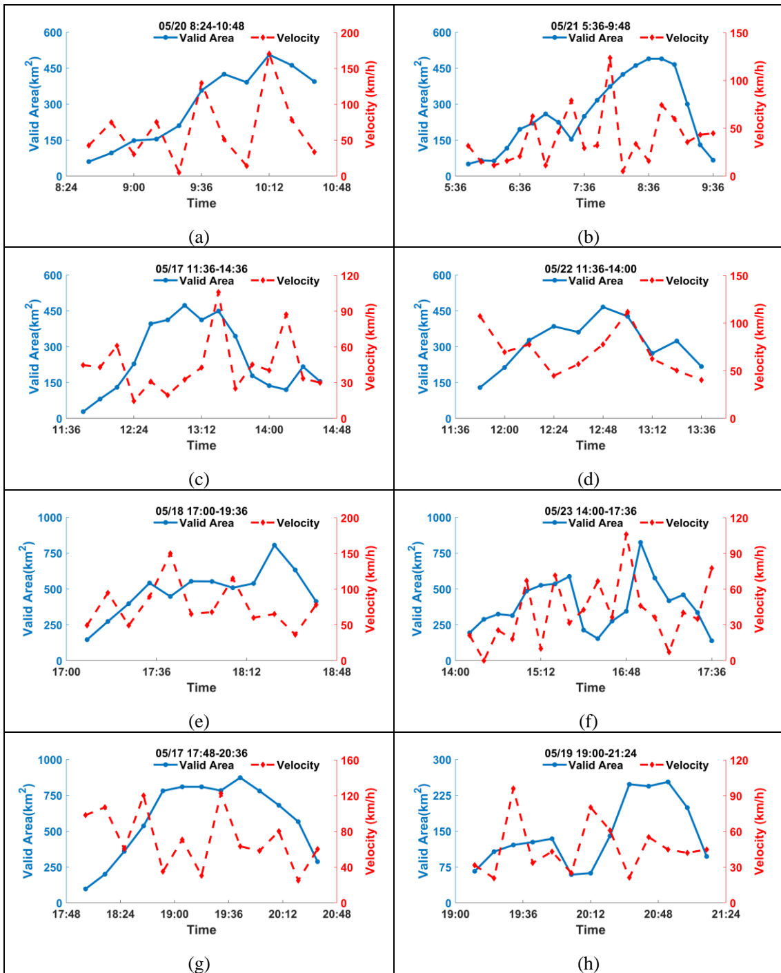
Figure 6. Valid area and velocity of eight cases, as a function of time. The blue solid line and the red dotted line represent the valid area and velocity within a time interval, respectively.
