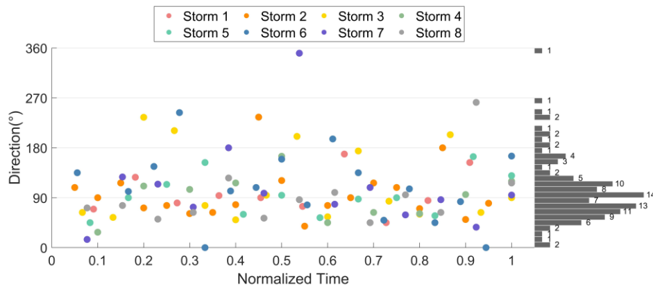
520 Figure 8. The cluster direction of motion in each interval. The colored dots denote different thunderstorms. As the duration of thunderstorms is different, the normalized time is used for the gathering of all directions of thunderstorm movements. The bar chart on the right represents the frequency of the 10° angle range.
