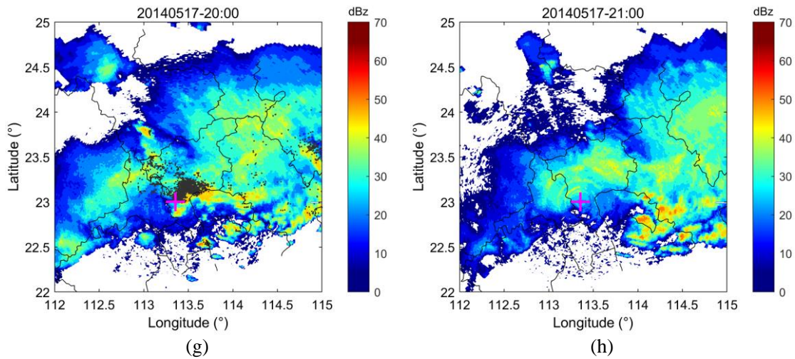
480 Figure 2. The stacking map of reflectivity scan by WSR-98D research radar and spatial distributions of total lightning data on 17 May 2014. Prominent areas of higher reflectivity are simultaneously covered by lightning events. The red plus represents the radar station which is situated on the east side of the FTLLS.
