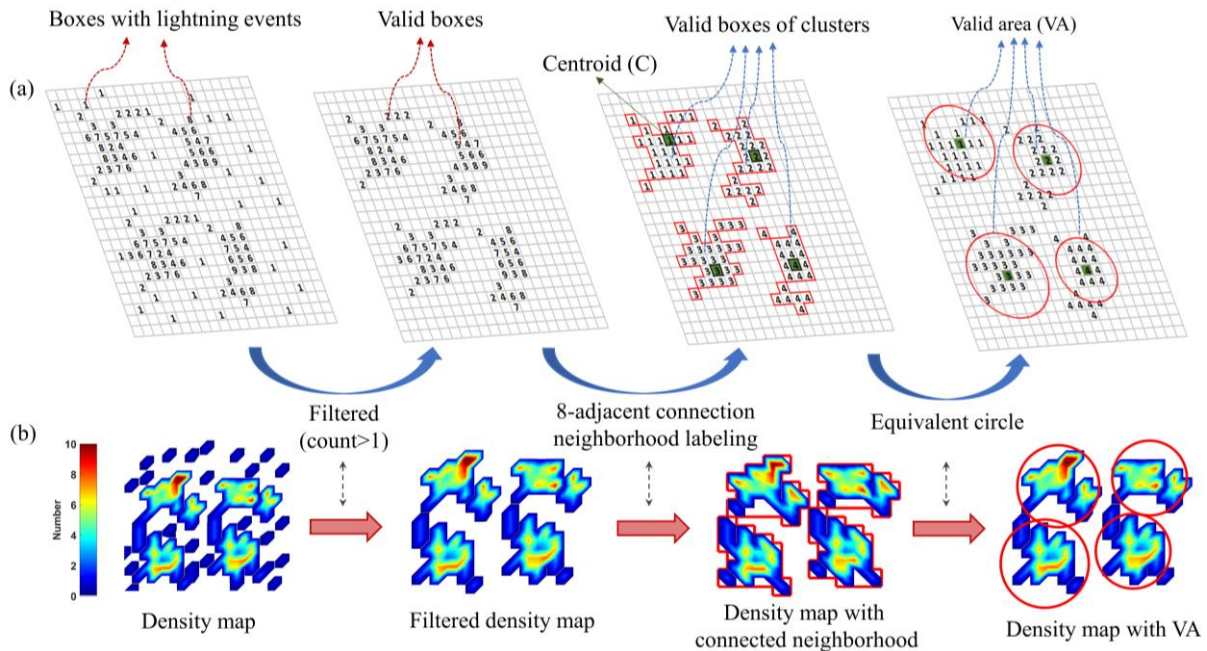
485 Figure 3. (a) Illustration of the 8-adjacent connected-neighbourhood labeling and the procedure of dealing with the lightning data to obtain the centroid and the valid area of clusters. (b) The workflow of cluster identification through density map.
