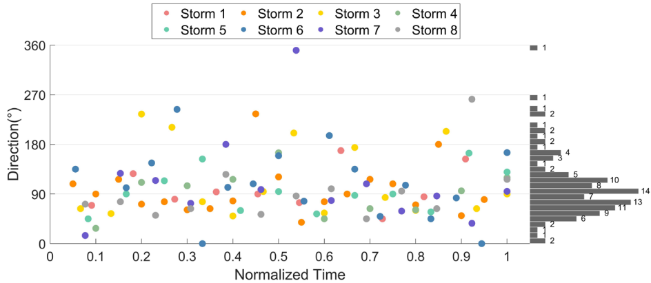
485 Figure 8. The cluster direction of motion in each interval. The colored dots denote different thunderstorms. As the duration of thunderstorms is different, the normalized time is used for the gathering of all directions of thunderstorm movements. The bar chart on the right represents the frequency of the 10° angle range.
