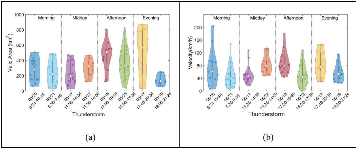
480 Figure 7. (a) Comparison of the valid area between eight cases. The upper and lower edges of boxes mean the maximum and minimum values. The white circle in each box represents the median of VA. The filled circles with a darker color than the box represent all VA values of thunderstorms. The grey vertical line in the box represent the interquartile range of VA. (b) Same as (a), but for the velocity.
