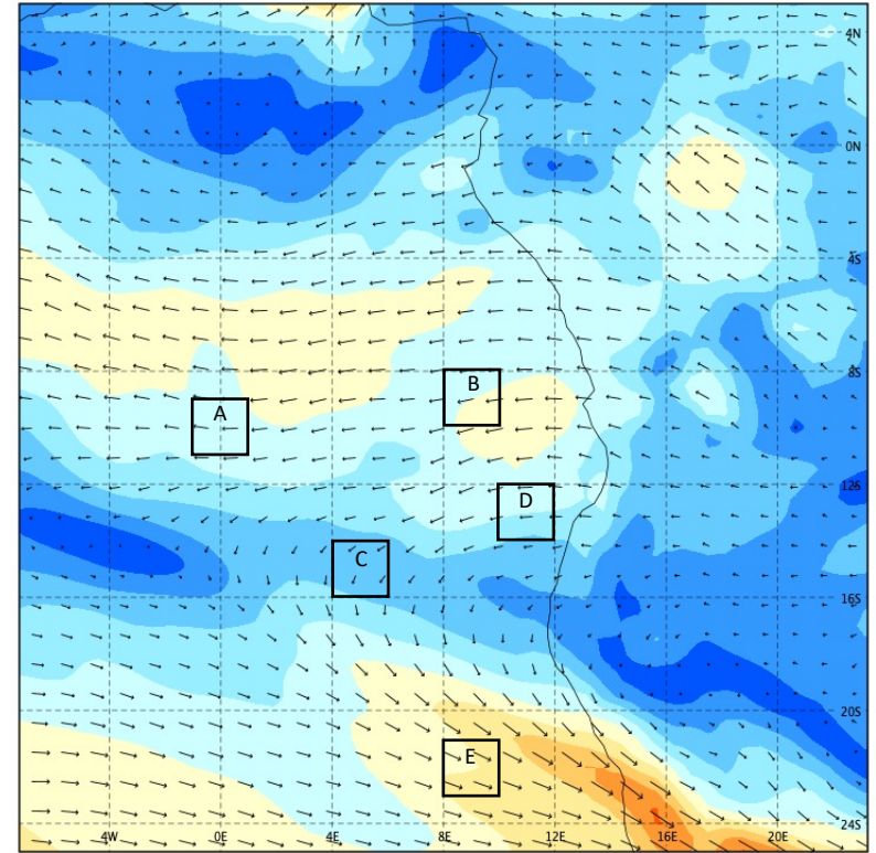
September 14 2016 1200 UTC 650 hPa Winds
