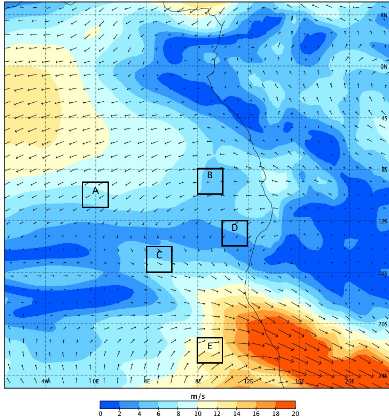
September 16 2016 1200 UTC 650 hPa Winds
