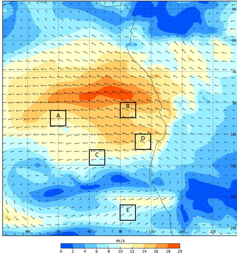
September 22 2016 1200 UTC 650 hPa Winds
