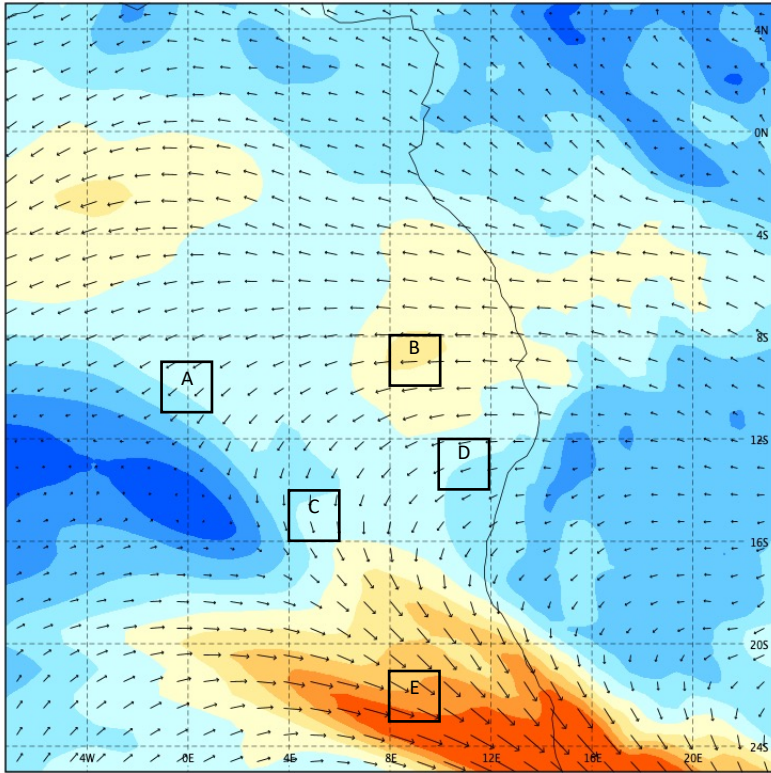
September 10 2016 1200 UTC 650 hPa Winds
