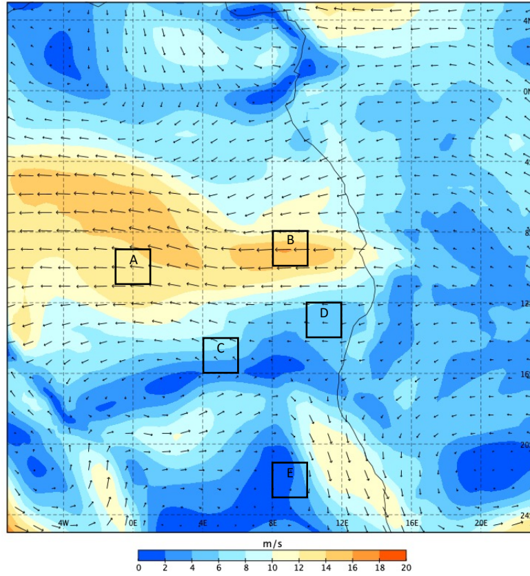
September 24 2016 1200 UTC 650 Pa
