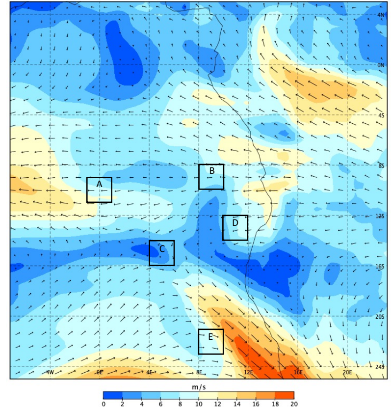
September 26 2016 1200 UTC 650 hPa Winds
