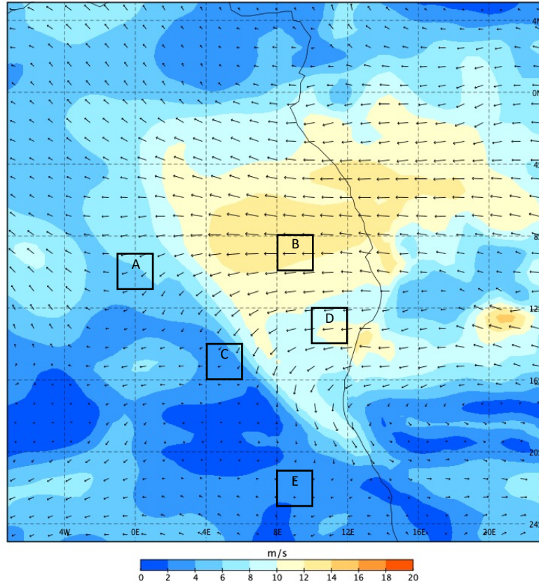
September 18 2016 1200 UTC 650 hPa Winds
