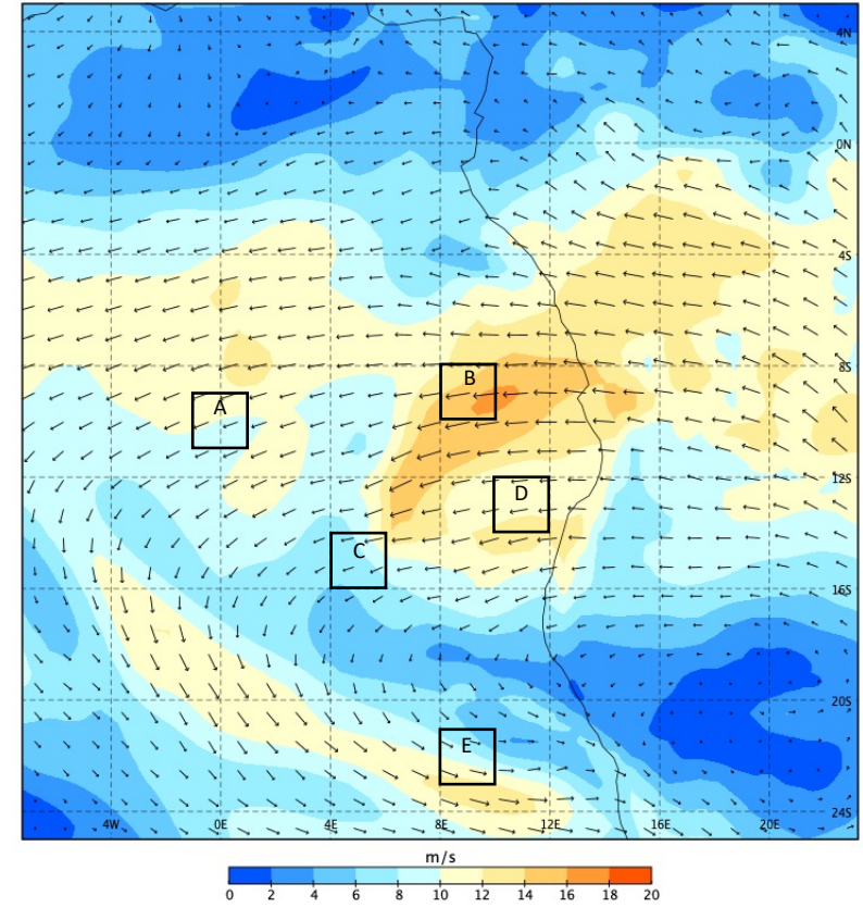
September 20 2016 1200 UTC 650 hPa
