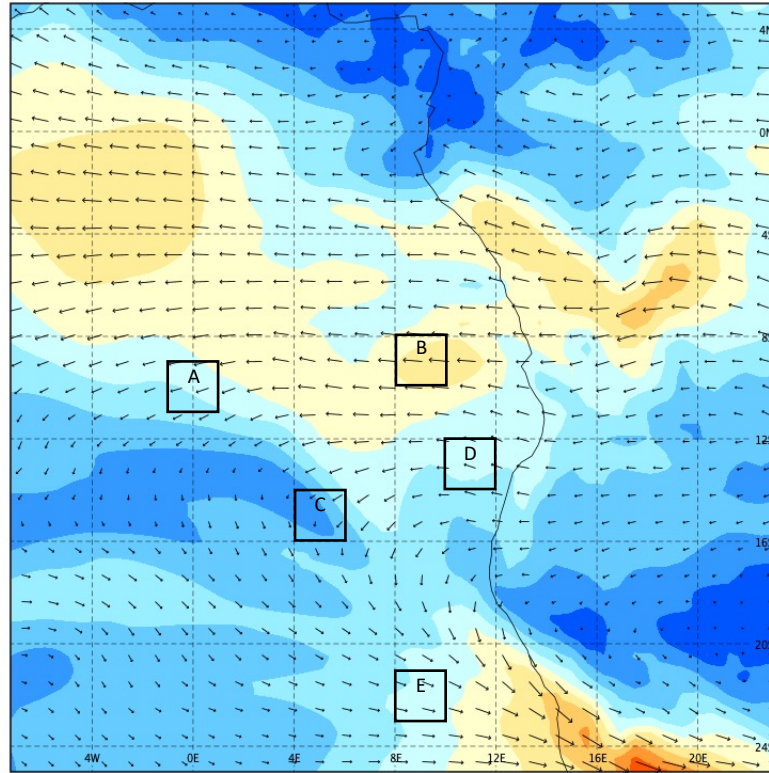
September 12 2016 1200 UTC 650 hPa Winds
