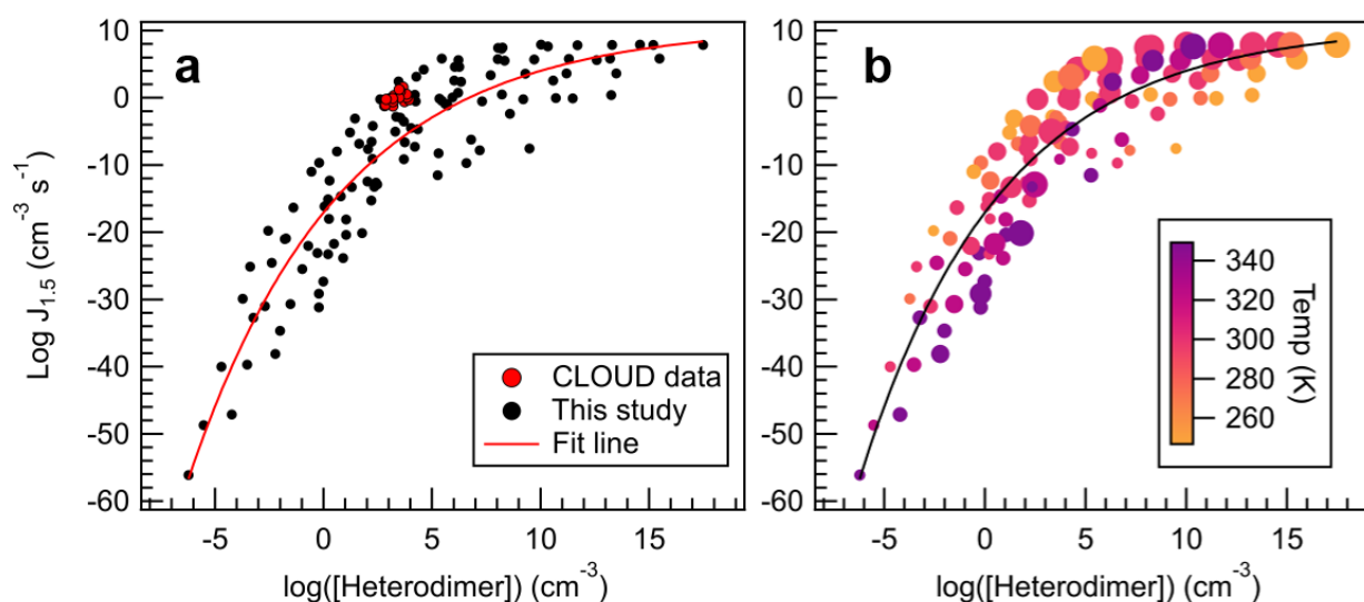
Figure 11. Heterodimer concentration plotted against J_{1.5} , wherein a) all data are represented with black dots, and b) data points are colored according to temperature and sized to reflect monomer concentrations ( 10^5 – 10^9 \text{ cm}^{-3} ). Data were fitted to an exponential function, which can be found in Equation 4.
