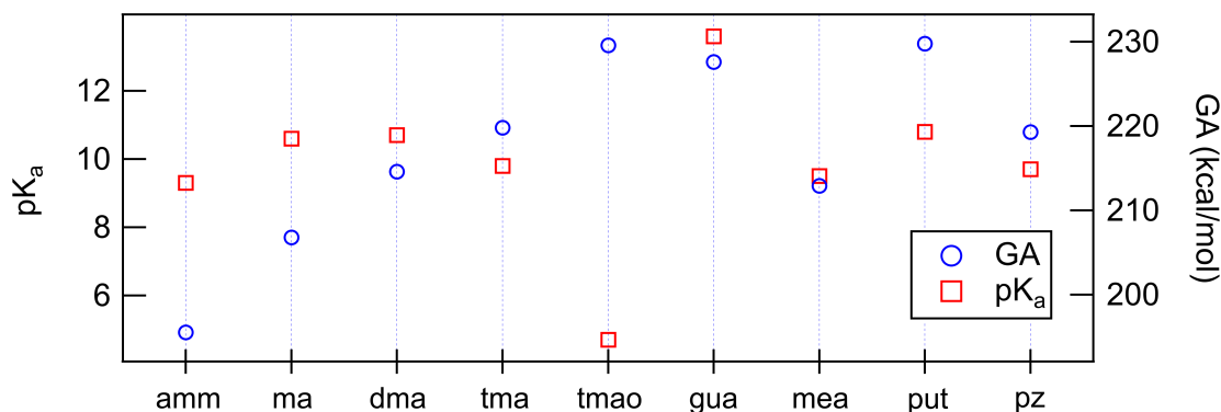
Figure 2. Calculated GA vs literature pK_a values from Haynes (2014).
