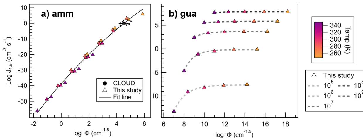
Figure 12. A) Amm and b) gua sa salts' J_{1.5} plotted against \Phi , where triangles are colored according to the temperature of that point's calculation. CLOUD data are shown as black dots, and their \Phi values were calculated according to Equation 5. All trendlines used an exponential fit.
