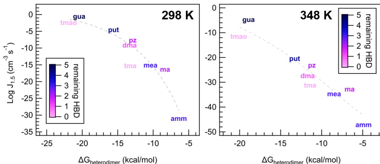
Figure 9. Individual data points and trendlines from Figure 8a colored according to the number of remaining hydrogen bond donors (HBD) on the heterodimer. The left is data from the 298 K case, and the right is data from the 348 K case, at [\text{acid}] = [\text{base}] = 10^6 \text{ molec cm}^{-3} .
