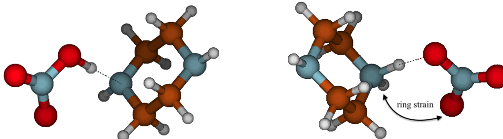
Figure 6. Deprotonated (left) and protonated (right) conformers of pz for the na–pz salt showing the ring strain necessary to form another intermolecular hydrogen bond.
