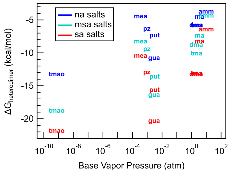
Figure 7. Base vapor pressure plotted against \Delta G_{\text{heterodimer}} for sa, msa, and na salts.
