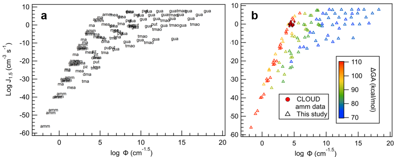
Figure 13. All sa salts plotted with a) base names as markers and b) markers colored according to their \Delta G_A values. CLOUD observations are shown as filled circles.
