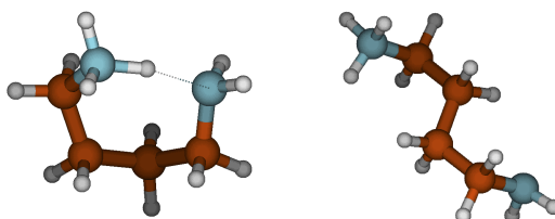
Figure 3. Cyclic and acyclic configurations of protonated put. The lowest energy acyclic structure is 14.6 kcal/mol higher in free energy than the cyclic, global minimum structure.
