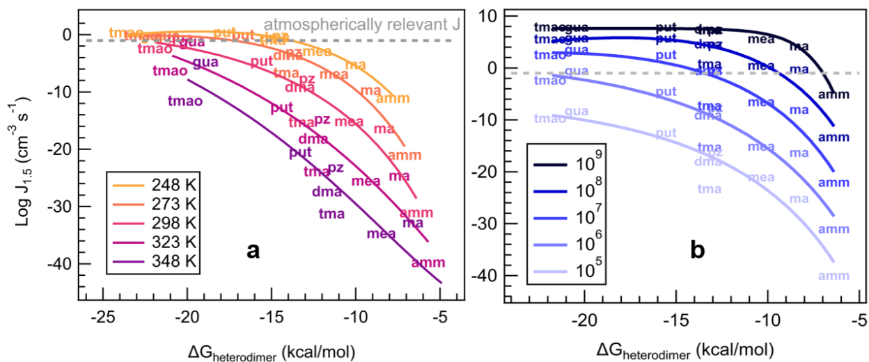
Figure 8. Heterodimer stability ( \Delta G_{\text{heterodimer}} ) plotted against NPF rate ( J_{\text{theory}} ) in varied conditions. a) Vapor concentrations are constant: [\text{acid}] = [\text{base}] = 10^6 \text{ molec cm}^{-3} at varying temperature: T = 248, 273, 298, 323, \text{ and } 348 \text{ K} . b) Temperature is constant: T = 298 \text{ K} at varying vapor concentrations: [\text{acid}] = [\text{base}] = 10^5, 10^6, 10^7, 10^8, \text{ and } 10^9 \text{ molec cm}^{-3} . Text markers are centered over the data point.
