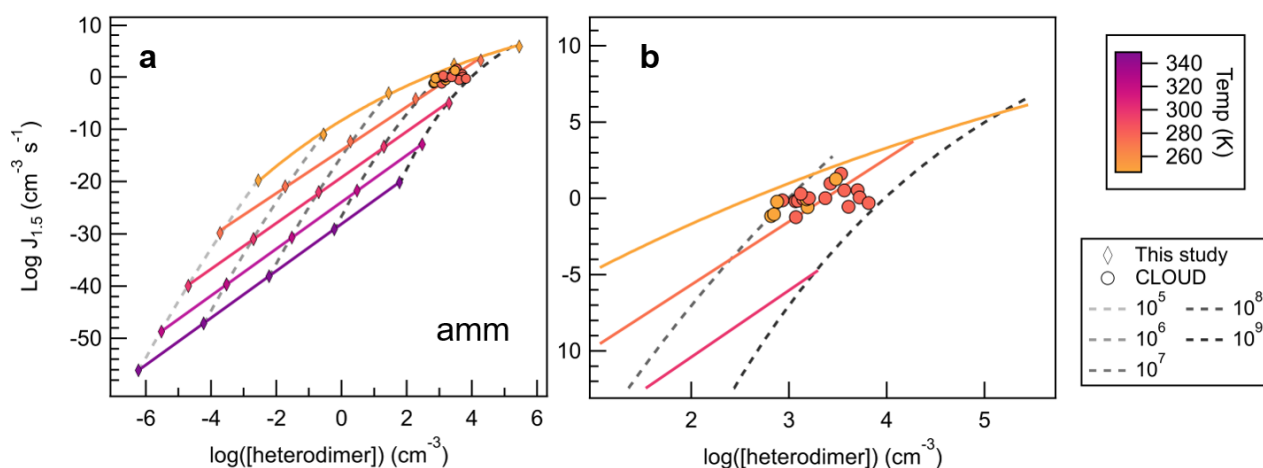
Figure 10. Heterodimer concentration plotted against J_{1.5} for sa–amm across 25 computational conditions (filled diamonds) from 248–348 K and monomer concentrations from 10^5 – 10^9 \text{ cm}^{-3} , where a) shows the full set of conditions calculated for sa–amm, and b) shows a magnification of how CLOUD data compares to the computational dataset. Colored lines correlate to temperature trendlines that were drawn through all data points calculated at the same temperature. Dashed lines represent data points calculated at the same monomer concentrations. We calculated heterodimer concentrations for CLOUD data whose acid and base concentrations were within 50% of each other according to Equation 3. All CLOUD data points were collected at temperatures of either 248 or 273 K (colored circles corresponding to color scale) and with monomer concentrations between approx. 10^8 – 10^9 \text{ cm}^{-3} .
