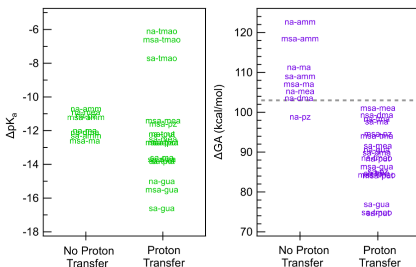
Figure 5. \Delta GA and \Delta pK_a values separated based on whether the heterodimer structure exhibits proton transfer. The grey dashed line on the \Delta GA graph at 103 kcal/mol shows the cutoff point for proton transfer.
