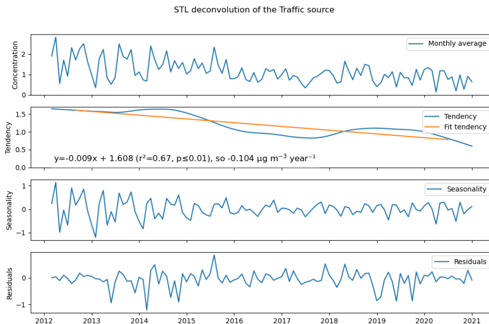
Figure 1: The Season-trend (STL) deconvolution of contributions in \mu\text{g m}^{-3} from the traffic factor to \text{PM}_{10} from year 2012 to 2020.
