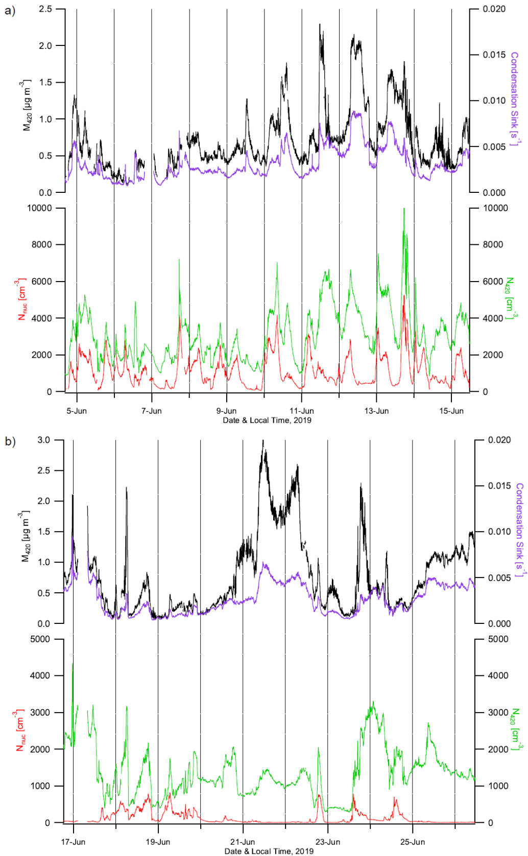
Fig. 4: Mass and number concentrations of aerosol particles <420 nm ( M_{420} and N_{420} ), number concentrations of nucleation mode particles <24 nm ( N_{\text{nuc}} ), and condensation sink at a) Eagle Lake and b) Nazko River.
