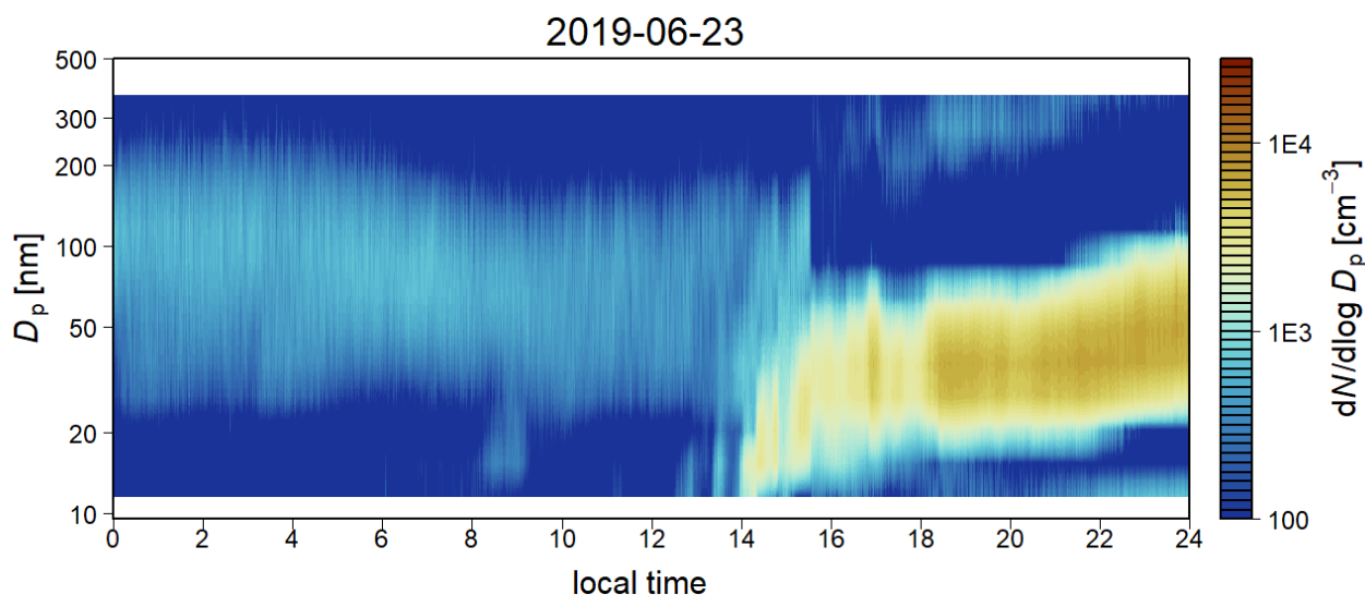
Fig. 7: Time series plots of the aerosol number size distribution of aerosol particles on exemplary days at a) Eagle Lake and b) Nazko River.
