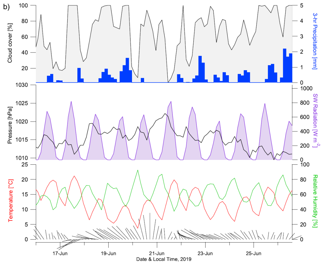
245 Fig. 2: Meteograms for the study periods at the a) Eagle Lake and b) Nazko River sites. Wind direction and speed are indicated by barbs at the bottom of the plots. (All data are from the NARR (North American Regional Reanalysis) database.)
