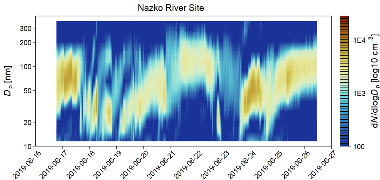
Fig. 5: Time series of aerosol number size distributions at a) Eagle Lake and b) Nazko River.
