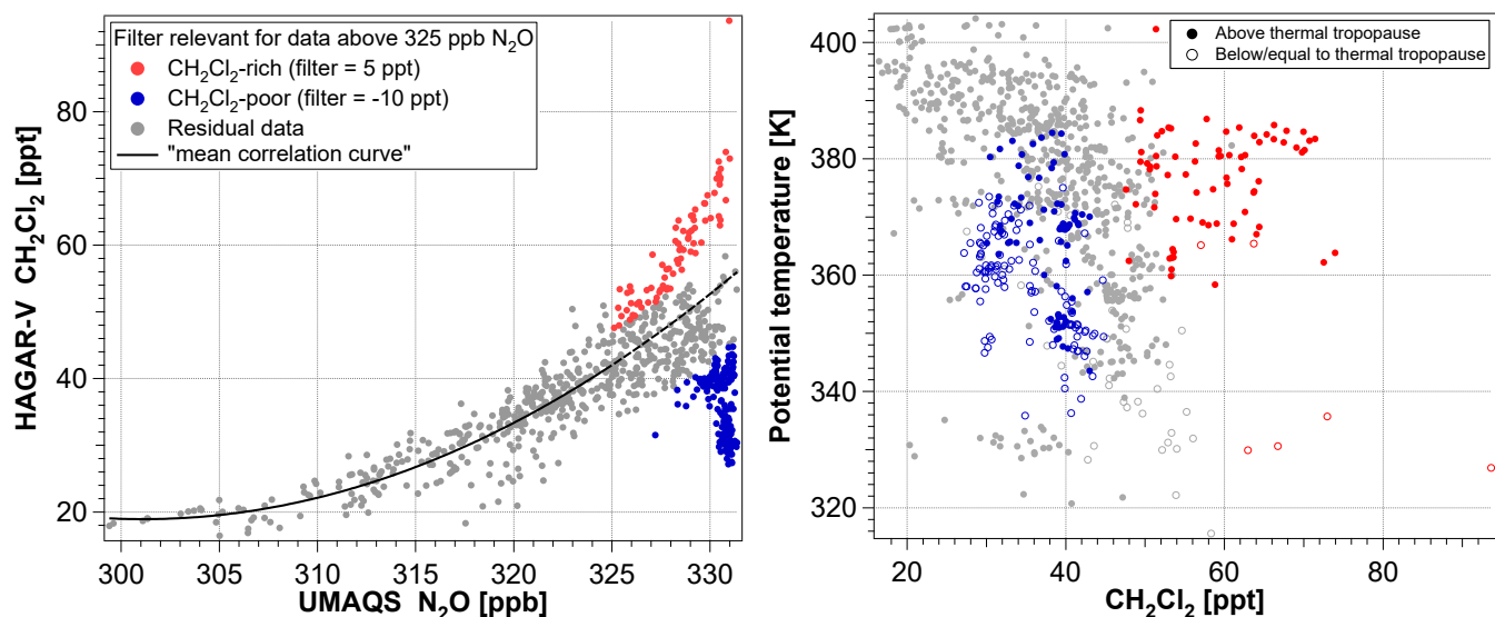
Figure 5. Left panel: \text{CH}_2\text{Cl}_2 - \text{N}_2\text{O} correlation relationship color coded with the used definition of the data filter. Red data points are considered measurements of considered as being \text{CH}_2\text{Cl}_2 -rich air, consisting of measurements with mixing ratios more than 5 ppt higher than the “mean correlation curve” and \text{N}_2\text{O} \geq 325 ppb. Blue data points are considered measurements of considered as being \text{CH}_2\text{Cl}_2 -poor air, consisting of measurements with mixing ratios more than 10 ppt lower than the “mean correlation curve” and \text{N}_2\text{O} \geq 325 ppb. The “mean correlation curve” is derived from a quadratic fit to the correlation \text{CH}_2\text{Cl}_2 - \text{N}_2\text{O} relationship for \text{N}_2\text{O} < 325 ppb extrapolated to higher mixing ratios relevant for the data filter (dashed line). Right panel: Scatter plot of \text{CH}_2\text{Cl}_2 as a function of the potential temperature and color coded to highlight \text{CH}_2\text{Cl}_2 -rich (red) and \text{CH}_2\text{Cl}_2 -poor (blue) air. On average the \text{CH}_2\text{Cl}_2 -rich air is found at higher potential temperatures than the \text{CH}_2\text{Cl}_2 -poor air.
