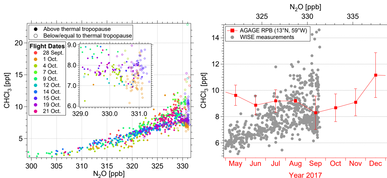
Figure C1. \text{CHCl}_3 - \text{N}_2\text{O} correlation relationship color coded by flight date (left) and monthly averaged ground-based \text{CHCl}_3 measurements of \text{CHCl}_3 from the AGAGE network at Ragged Point, Barbados (right; Prinn et al., 2018) overlaid by a detailed plot of the \text{CHCl}_3 - \text{N}_2\text{O} correlation relationship. The right plot showing the AGAGE \text{CHCl}_3 time series of the AGAGE network is similar to Figure 4 where a detailed description is given.
