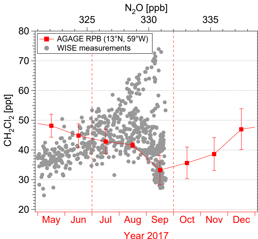
Figure 4. Monthly averaged ground-based CH 2 Cl 2 measurements of CH 2 Cl 2 from the AGAGE network at Ragged Point, Barbados (13° N Prinn et al., 2018) overlayed by a detailed plot of the CH 2 Cl 2 -N 2 O correlation relationship observed during WISE. The AGAGE CH 2 Cl 2 time series (shown in red) shows CH 2 Cl 2 ’s seasonality and is overlayed by the correlation CH 2 Cl 2 -N 2 O relationship such that the CH 2 Cl 2 minimum at N 2 O ≥ 325 ppb measured during WISE in October 2017 matches the surface CH 2 Cl 2 minimum at Barbados in September 2017. Further, the axis of the time series is adjusted so that 1 month corresponds to a change of ≈ 2 ppb N 2 O, which is the typical N 2 O change per month of age in the UTLS (Andrews et al., 2001). The gradient of the CH 2 Cl 2 -N 2 O correlation relationship ’s lower branch ( low CH 2 Cl 2 mixing ratios between dashed red lines ) qualitatively fits the temporal variation of the ground-based CH 2 Cl 2 measurements. The graph illustrates the congruence of ground-based tropical AGAGE measurements of CH 2 Cl 2 measurements from the AGAGE network and airborne extratropical WISE measurements of CH 2 Cl 2 measurements from the WISE campaign when assuming that the variation of stratospheric CH 2 Cl 2 with age (here expressed in terms of N 2 O mixing ratio) arises from the temporal variation of CH 2 Cl 2 at the ground (“tape recorder effect”). Although this simplified view ignores the impact of mixing processes and chemical reduction of CH 2 Cl 2 it qualitatively explains the lower branch of the correlation curve CH 2 Cl 2 -N 2 O relationship for air parcels younger than a few months.
