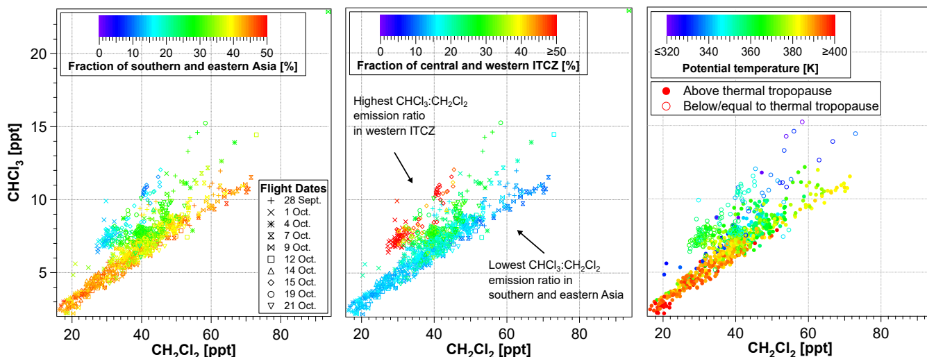
Figure 13. \text{CHCl}_3 - \text{CH}_2\text{Cl}_2 correlationrelationship color coded with the SaEA (left) and the W-ITCZ (center) surface origin tracer, and the potential temperature (right). The correlationrelationship exhibits different correlation slopes clearly depending on the origin of air. A large impact of sources from southern and eastern Asia coincides with a low correlation slope dominating the larger part of the correlationrelationship. A large impact of sources from the central and western part of the ITCZ coincides with the steepest correlation slope implying a relatively larger \text{CHCl}_3 : \text{CH}_2\text{Cl}_2 emission ratio in this region compared to the emission ratio in southern and eastern Asia. The highest \text{CHCl}_3 mixing ratios and the majority of measurements with the steepest correlation slope were observed in the tropopause region and the upper troposphere.
