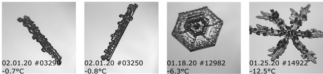
222 FIG. 2. Examples of representative PHIPS particles with different degrees of riming categorized by the 223 surface riming degree (SRD): unrimed (SRD=0%), slightly rimed (0% < SRD < 25%) and moderately rimed 224 (25 ≤ SRD ≤ 50%) particles. Heavily rimed (50% < SRD < 100%) and graupel particles (SRD = 100%) are 225 shown in Fig. 3.
