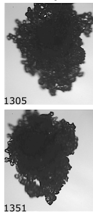
486 FIG. 11. Corresponding representative PHIPS images of particles sampled during the segment indicated by 487 the dashed black lines in in Fig. 10. The numbers in the bottom left denote the image number.
