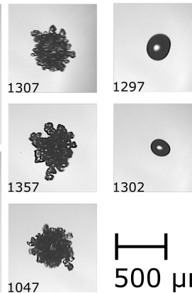
486 FIG. 11. Corresponding representative PHIPS images of particles sampled during the segment indicated by 487 the dashed black lines in in Fig. 10. The numbers in the bottom left denote the image number.
