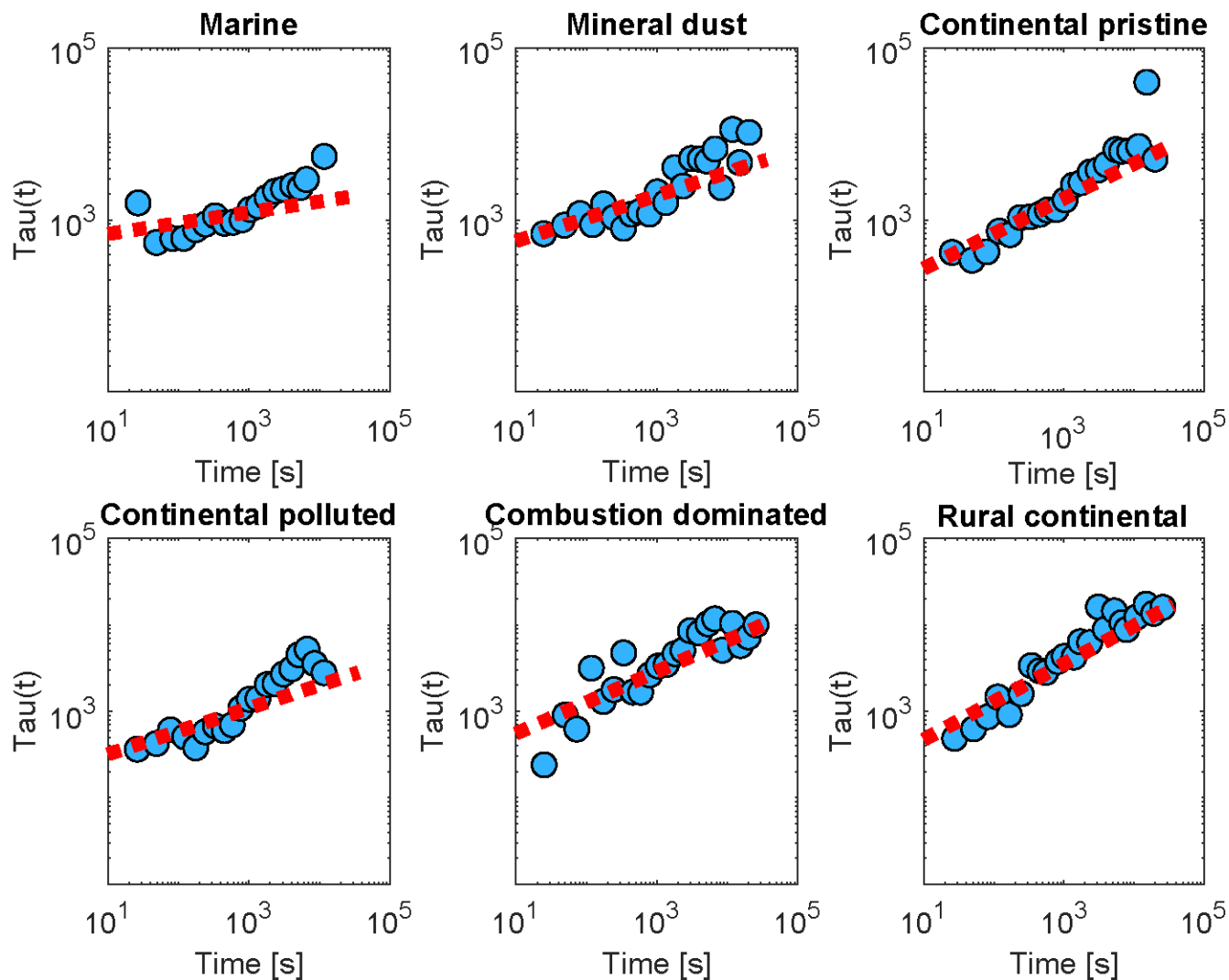
Figure 12: The relaxation time \tau inferred from the isothermal experiments (up to 10 hours) using the averaged data (yellow dots in Figure 9), with Eq (3) as a function of time since the start of the isothermal phase (blue dots) for the marine dominated, mineral dust influenced, continental pristine, continental polluted, combustion dominated and rural continental samples of aerosol material (panels from top left to lower right). Also shown are empirical fits for all measurements of each sample using
