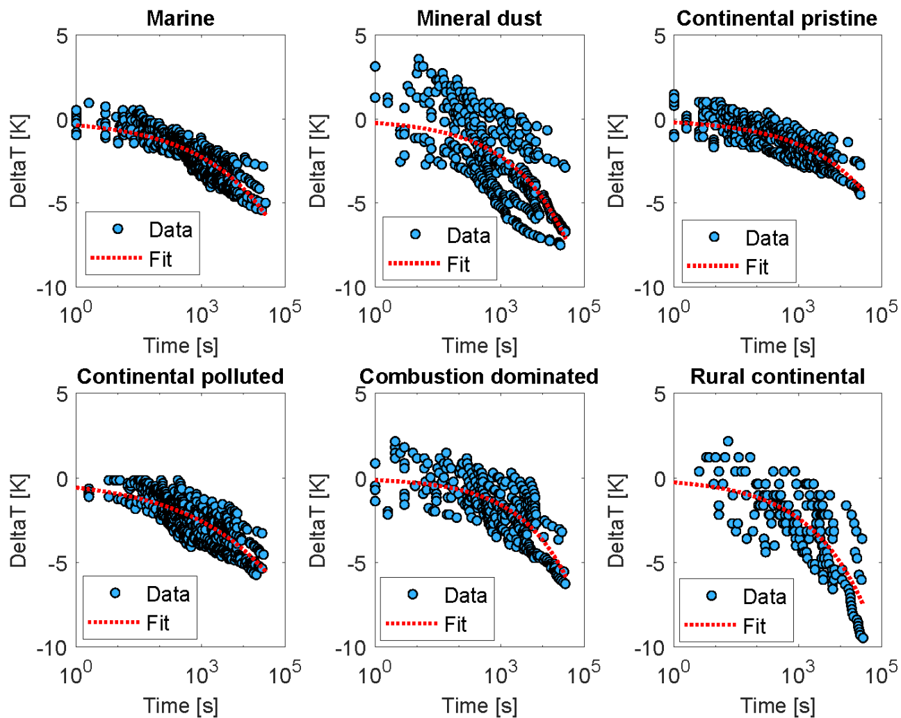
1570 Figure 13: The apparent temperature shift, \Delta T , required to match the empirical parameterization of the INP activity (Phillips et al. 2013) with the measurements of frozen fraction from the isothermal experiments (blue dots), for the marine dominated, mineral dust influenced, continental pristine, continental polluted, combustion dominated and rural continental samples of aerosol material (panels from top left to lower right). Evolution over time since the start of the isothermal phase is displayed. Also shown is the fit (Eq (6)) assuming a power law dependent on time (red dotted line).
