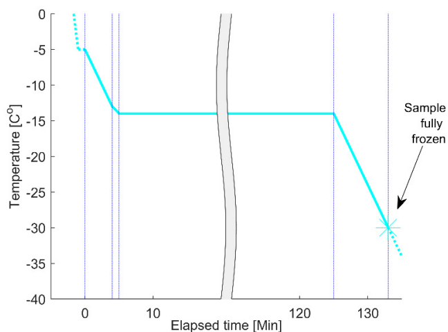
Figure 4: The cooling programs used in this study. The cyan lines display the evolution of temperature as a function of time, the blue dotted lines indicate where the cooling rate was changed and where the experiment was completed (when the sample was fully frozen). Left panel: the cooling program for the constant cooling rate experiments. Right panel: The cooling program used for the 2-hour isothermal experiments. One isothermal experiment with a longer isothermal period (11 – 16 hours) was also done on each drop population (not shown). In this figure, the timescale starts ( t = 0 ) at the first cooling ramp after the 1 min pause at -5\text{ }^{\circ}\text{C} , all times referred to in the analysis for the isothermal experiments are from the start of the isothermal phase, if nothing else is specifically stated.
