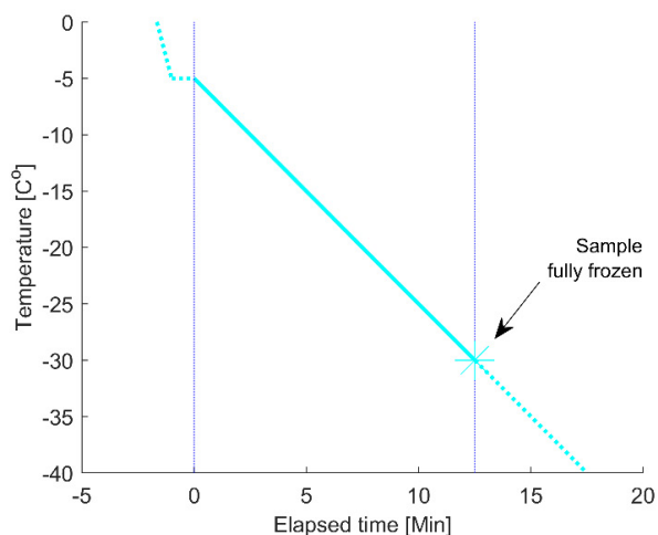
Figure 4: The cooling programs used in this study. The cyan lines display the evolution of temperature as a function of time, the blue dotted lines indicate where the cooling rate was changed and where the experiment was completed (when the sample was fully frozen). Left panel: the cooling program for the constant cooling rate experiments. Right panel: The cooling program used for the 2-hour isothermal experiments. One isothermal experiment with a longer isothermal period (11 – 16 hours) was also done on each drop population (not shown). In this figure, the timescale starts ( t = 0 ) at the first cooling ramp after the 1 min pause at -5\text{ }^{\circ}\text{C} , all times referred to in the analysis for the isothermal experiments are from the start of the isothermal phase, if nothing else is specifically stated.
