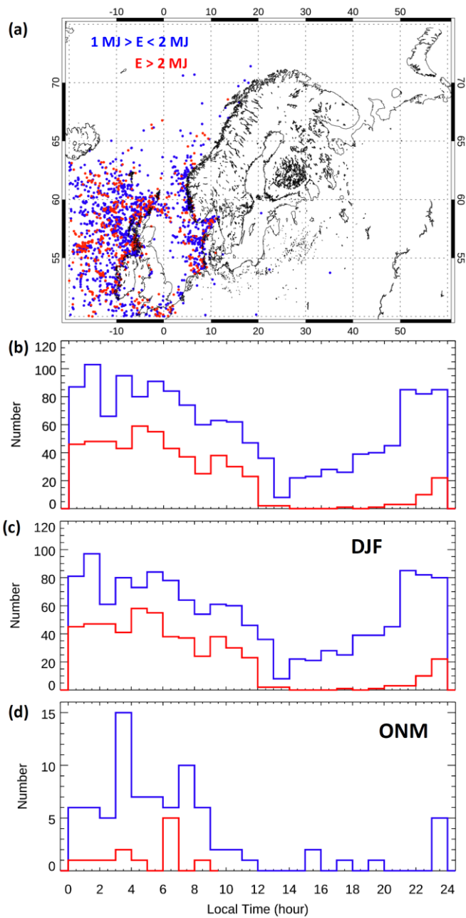
225 Figure 4: a) Spatial distribution of superbolts (strokes with energies between 1 and 2 MJ and above 2 MJ are respectively represented by blue and red color). b) Temporal distribution of superbolts as a function of the local time. The same as in (b), but for DJF (c) and ONM (d).
