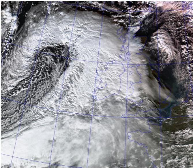
Figure 1: Infrared image collected by the polar-orbiting NOAA19 satellite shows the storm Rachel that threatened the UK and Ireland on 14 January 2015.
