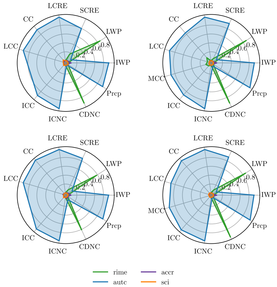
Figure C2. Same as Fig. 9-12 but using the whole response surface for the first order sensitivity analysis indices.
