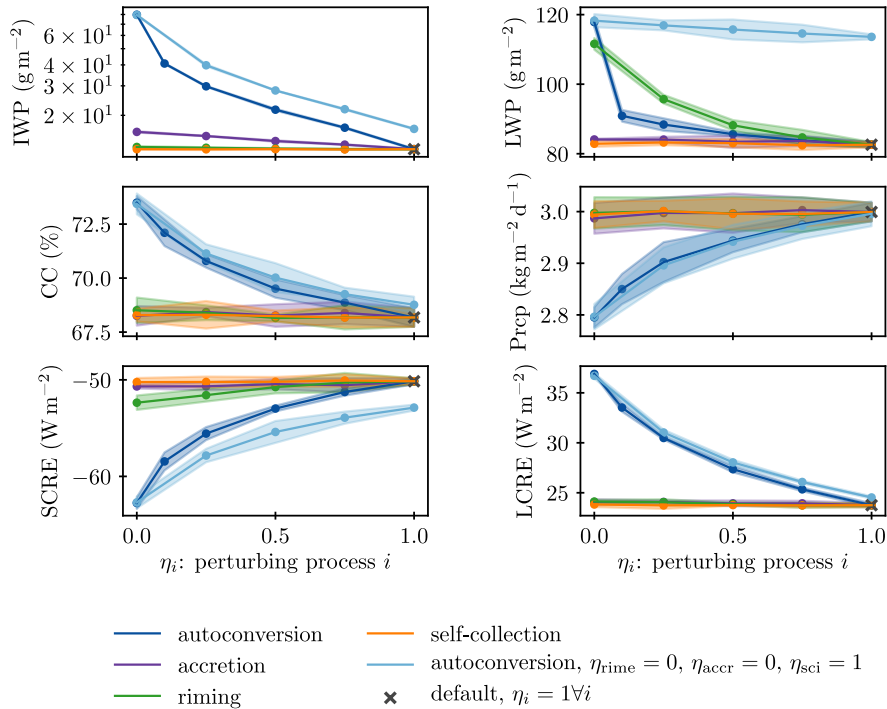
Figure 5. Model response to phasing perturbations of four CMP processes: aggregation autoconversion , accretion, riming and self-collection (as illustrated in Fig. 1) in terms of global annual mean IWP, liquid water path (LWP), cloud cover (CC), precipitation (Prep), shortwave and longwave cloud radiative effect (SCRE, LCRE). An additional experiment was conducted to highlight interactive effects between the phasing perturbation of aggregation autoconversion and the inhibition of riming and accretion (light blue). The points and line indicate the mean and the shading indicates 2 times the standard deviation of annual mean values of a five-year simulation. Classical sensitivity studies would only show \eta_i = 0 and \eta_i = 1 . Note that we added an extra simulation at \eta_{autc} = 0.1 to better illustrate the threshold behaviour discussed in the text and that for the IWP the shading is hidden behind the lines.
