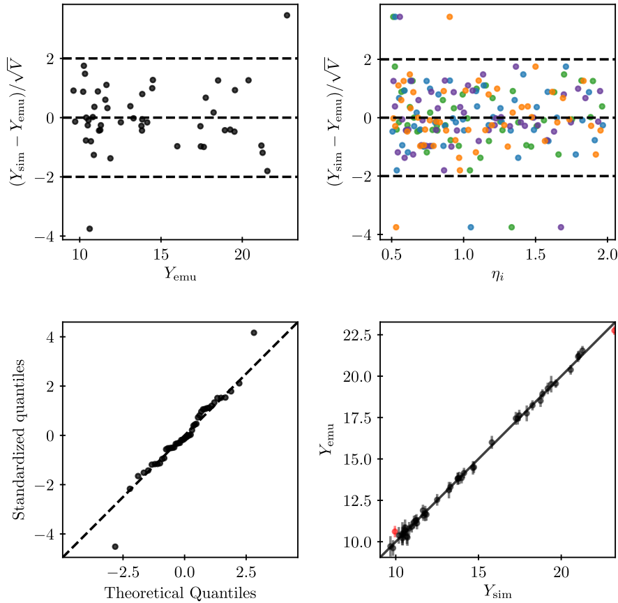
Figure 4. 1-out-validation Leave-one-out validation of the emulator for global annual mean IWP according to Bastos and O’Hagan (2009). Each point corresponds to the training of the emulator on all points except one and then testing on exactly that point. Individual standardized errors are plotted against a) emulator output and b) input parameters (colors according to Fig. 5: aggregation autoconversion (blue), accretion (purple), riming (green), self-collection (orange)). The dashed lines are drawn at an individual standardized error of zero and 2, which is the threshold discussed in Bastos and O’Hagan (2009). c) QQ-plot of the individual standardized errors against a student-T distribution. d) Emulator against model output, with the error bars indicating the 95% confidence interval on the emulator predictions. Predictions for which the model result lies outside that interval are marked red.
