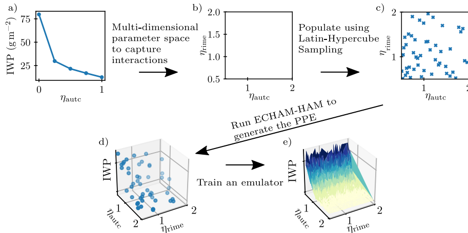
Figure 3. Sketch of the employed methodology: we move from a) one-dimensional sensitivity studies where one process is phased-perturbed by varying the parameter \eta (Sect. 3.1) to b) a multi-dimensional parameter space. c) The input parameter space is filled with Latin Hypercube sampling and supplied as input to ECHAM-HAM. The simulations form the perturbed parameter ensemble (PPE). The d) PPE output is e) fitted using a Gaussian Process emulator for each variable of interest to generate a smooth response surface, upon which sensitivity analysis can be applied. Note that this is an illustrative sketch of the method for a PPE with two input dimensions, whereas our PPE has four dimensions, and that the data used to generate it is only illustrative as well. The shading in d) illustrates depth only.
