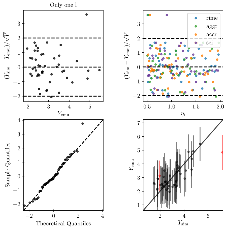
Figure D1. Validation of the emulated angular amplitude spectrum of degree l=16 \llcorner l=6 for the LWP.
