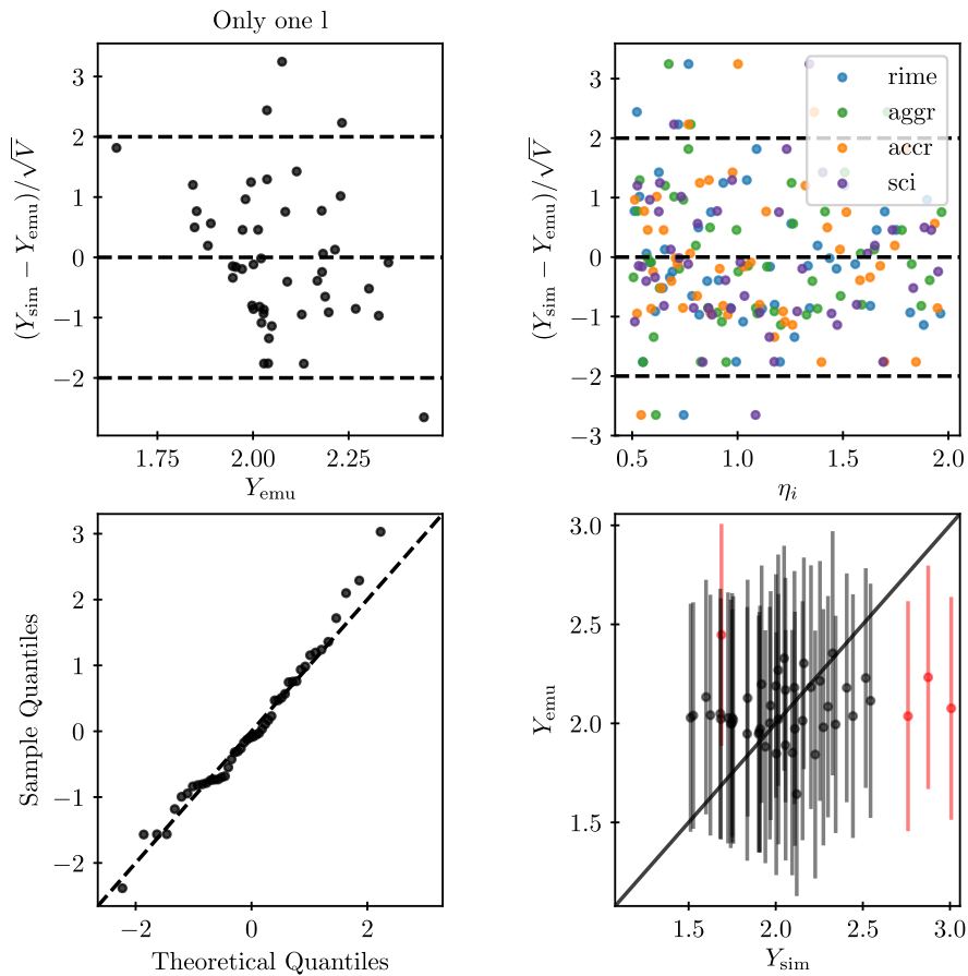
Figure D3. Validation of the emulated angular amplitude spectrum of degree l=11 l=16 for the LWP (see Fig. D2), which failed because of diagnosed defaulting.
