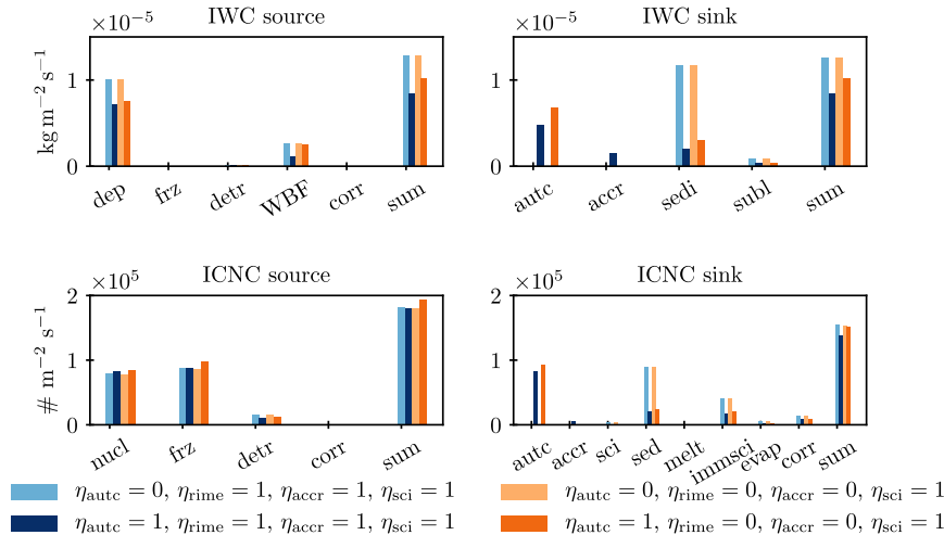
Figure 6. Global annual mean vertically integrated process rates for four experiments that illustrate the inhibition of snow formation through turning off aggregation-autoconversion (mean of a five-year simulation). The rates are diagnosed similar to Bacer et al. (2021), but correction terms were themselves subtracted from process rates where appropriate, i.e. where the correction belongs to the logical entity of the process rate (see Sec. 2.1). The process rates are: deposition (dep), heterogeneous and homogeneous freezing (frz), detrainment (detr), deposition in the Wegener-Bergeron-Findeisen process (WBF), correction terms (corr), aggregation-autoconversion ( aggrautc ), accretion (accr), sedimentation (sedi), sublimation (subl), ice nucleation in the cirrus scheme (nucl), melting (melt), immediate self-collection of ice crystals when the ICNC is larger than a maximal threshold (immsci), evaporation (evap).
