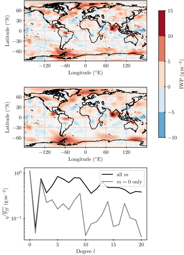
Figure 10. Spherical harmonics expansions for one illustrative PPE member ( \eta_{aggr} \approx 0.31 , \eta_{autc} \approx 0.87 , \eta_{acrr} \approx 0.90 , \eta_{acrr} \approx 1.43 , \eta_{rime} \approx 0.89 , \eta_{rime} \approx 0.81 , \eta_{sci} \approx 0.36 , \eta_{sci} \approx 1.89 ). a) Difference to control ( \eta_i = 1 \forall i ) in the global annual mean IWP, b) expansion of spherical harmonics representing the same data as a) , generated from the coefficients of the expansion displayed as an angular amplitude spectrum in c) as a function of the degree l (with m independent solutions, where modes of m = 0 most strongly resemble rotationally symmetric physical patterns of the Earth system such as a North-South contrast). Note that the variability explained by each degree l in general decreases with increasing l , which allows us to truncated truncate the expansion at the degree l where it represents 95% of the total data variance.
