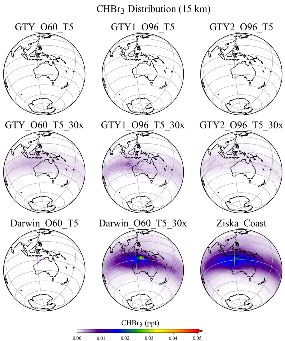
Figure S3. Same as Figure S2, but for 15 km.
