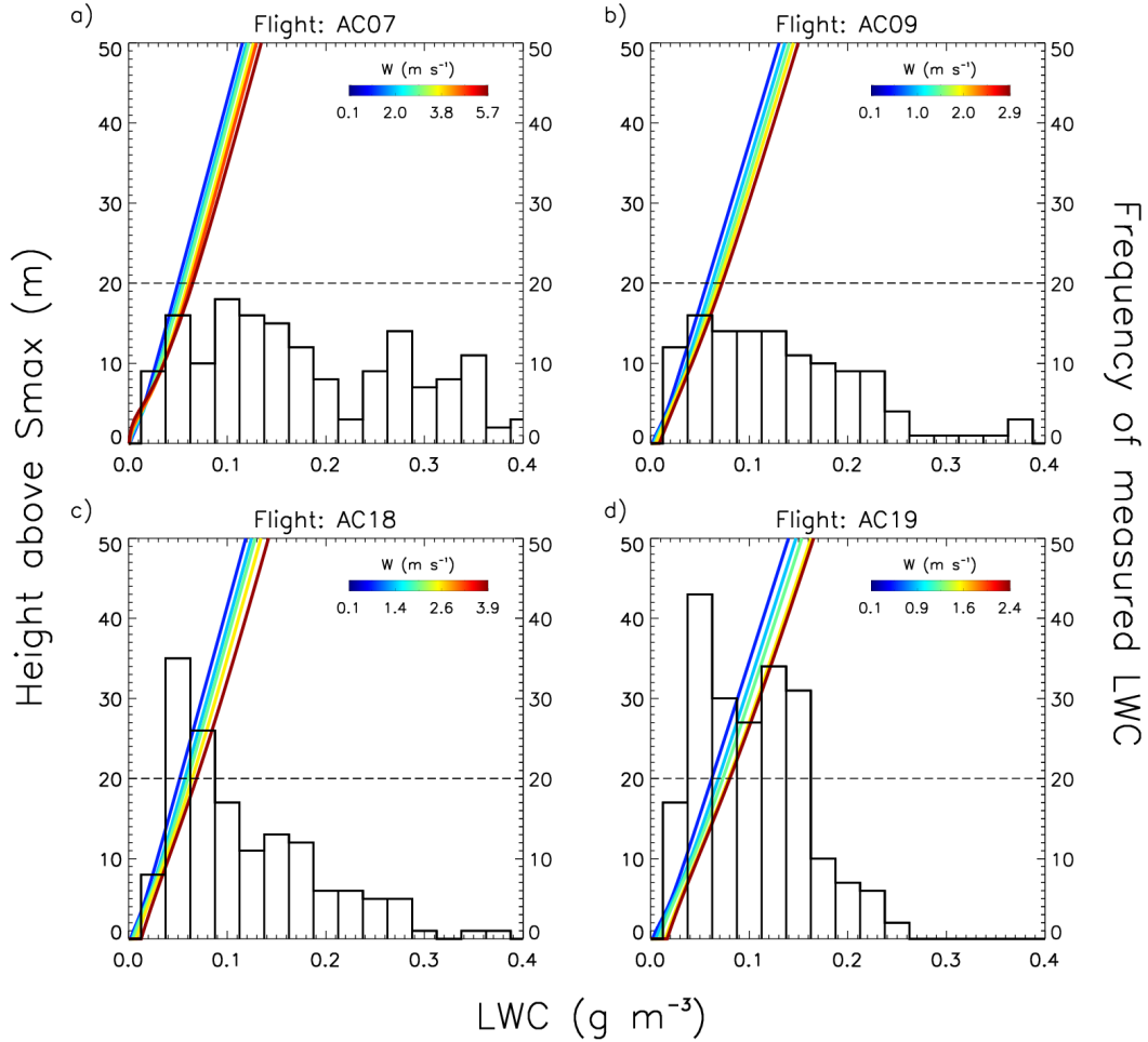
Figure 3. Predicted LWC [ \text{g m}^{-3} ] as a function of height above the level of S_{max} [left axis] and w (lines, color-coded by w [ \text{m s}^{-1} ]) for flights a) AC07, b) AC09, c) AC18, d) AC19. The vertical bars indicate the number of cloud passes (with a temporal resolution of 1 s) as a function of the measured LWC by CAS-DPOL and CCP-CDP in cloud (right axis). The dashed line denotes the level of 20 m above predicted maximum supersaturation, at which N_{d,p} is predicted (Section 3.2.2).
