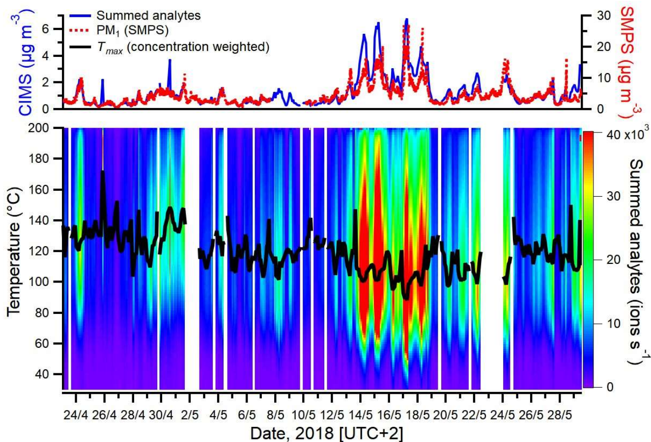
Figure 1: Comparison between the total summed analytes (excluding reagent ions) measured in particle phase by FIGAERO-CIMS and particle mass concentration (PM 1 ) calculated from SMPS size distribution measurements (upper panel), and thermograms of the summed analytes during each FIGAERO cycle (lower panel). Black line represents the concentration-weighted T_{\text{max}} for each measurement cycle.
