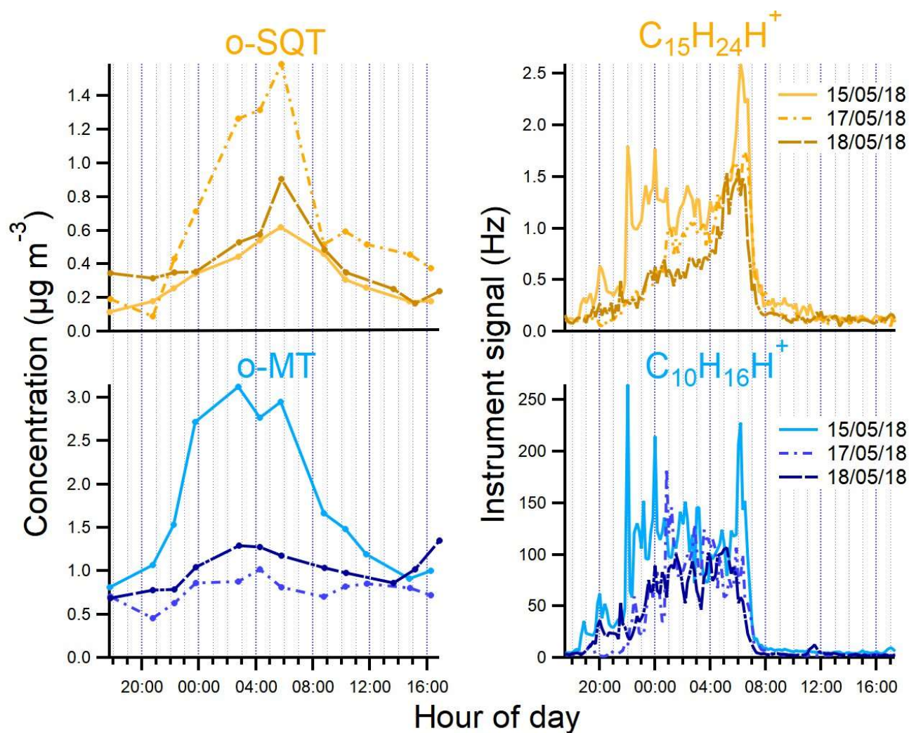
830 Figure 5: Diurnal variation of o-SQT and o-MT in particle phase measured by FIGAERO-CIMS and of sesquiterpenes ( \text{C}_{15}\text{H}_{24}\text{H}^+ ) and monoterpenes ( \text{C}_{10}\text{H}_{16}\text{H}^+ ) measured by PTR-ToF-MS during the events described in this study.
