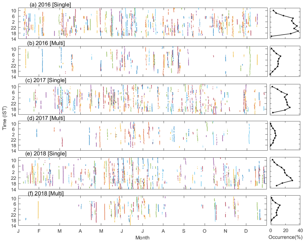
980 Figure 4: The day-to-day occurrence of the cirrus clouds from 14:00 IST on day one to 11:00 IST on day two and overall percentage occurrence for (a) single and (b) multi-layer cirrus clouds during 2016. (c-d) and (e-f) is the same as (a-b) but observed during 2017 and 2018, respectively. We referred to 'single' for the one-layer clouds and the first layer in the case of the multiple cirrus clouds. At the same time, 'multi' is referred for the second layer of cirrus clouds in the cases of multiple cirrus layers. Note that the colours used here have no specific meaning but are simply used to make it easier to distinguish between different days.
