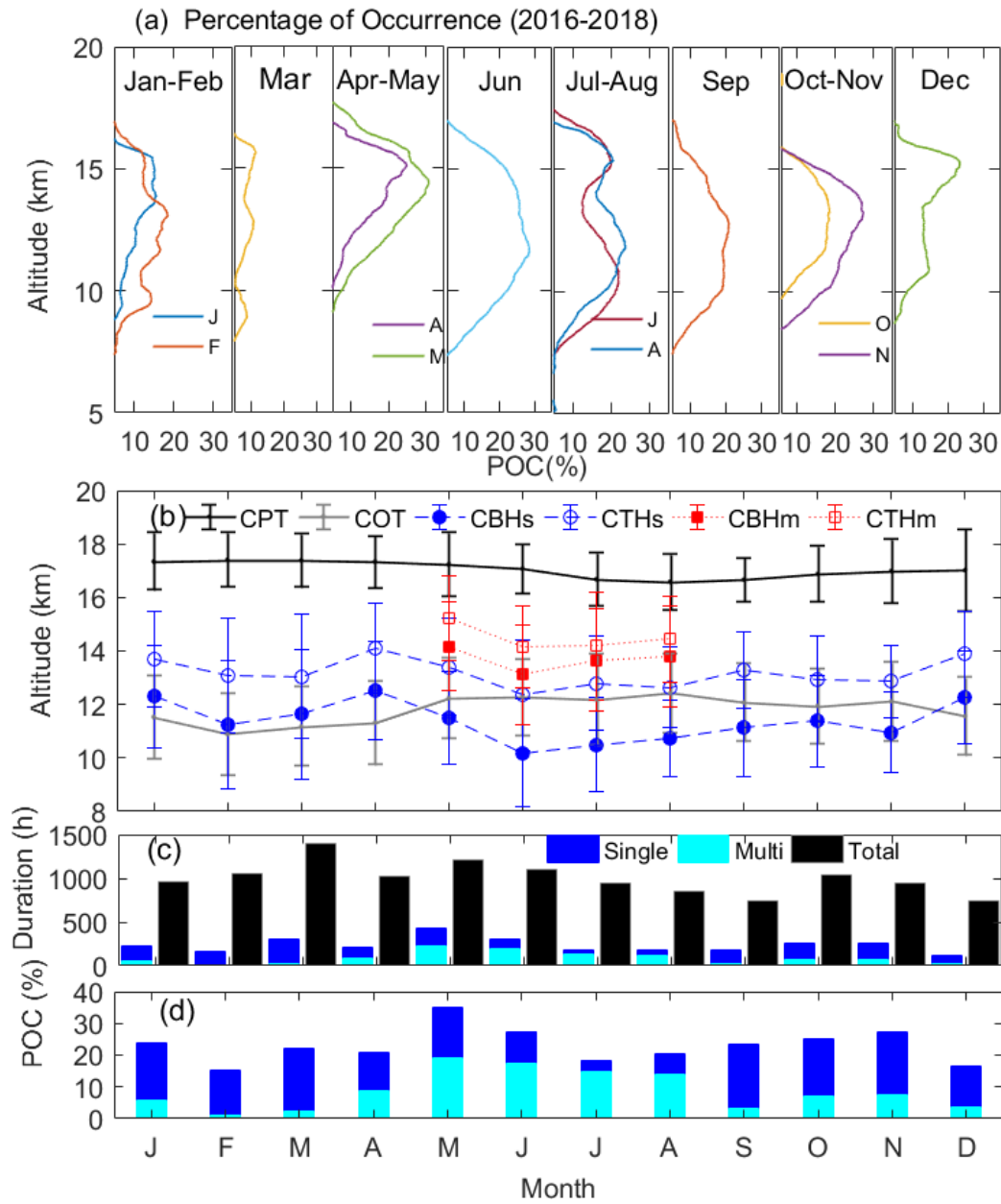
1040 Figure 7: (a) Monthwise variation of the altitude extent of the POC, (b) monthly mean and standard deviations of the altitudes of cloud base and top, CPT and COT, (c) monthwise total observations of MPL and (d) cirrus the occurrence of the single and multi-layered clouds over the period 2016-2018.
