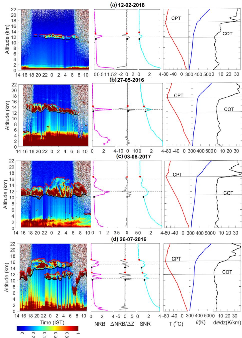
935 Figure 2: Time height section of the normalized backscattered (NRB) signals over the altitude 0.3 -22 km observed on 15:00 IST on the first day to 11:00 IST on the second day. The vertical profiles of the NRB, the gradient of NRB and SNR signals at 01:30 IST using MPL over Kattankulathur along with the daily mean temperature, potential temperature, and potential temperature gradient using radiosonde observation over Meenambakkam for different types of the cirrus clouds cases (a) laminar cirrus (12-02-2018) (b) descending cirrus (27-05-2016) (c) broad cirrus (03-08-2017), and (d) multi-layered cirrus clouds (26-07-2016). Red and black dots denote the cirrus cloud top and base of the cloud layers, respectively. Dashed lines indicate the peak altitudes of the cirrus layers. Dotted horizontal lines indicate the associated secondary peak with the main peak. Cold point tropopause (CPT) and convective 940 tropopause (COT) are also shown. Note that 10 point running mean has been applied to the NRB gradient and temperature gradient profiles to smooth out the small-scale fluctuations.
