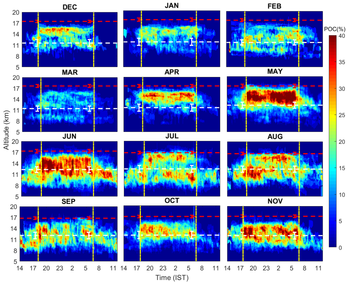
1025 Figure 6: Monthly occurrence of cirrus clouds as a function of time and altitude from 2016 to 2018. The mean CPT (red line) and COT (white line) altitudes for the corresponding months are also embedded. The standard deviation of the CPT altitude at 17:30 IST and 05:30 IST is also shown. Vertical dashed lines indicate the sunset and sunrise timings.
