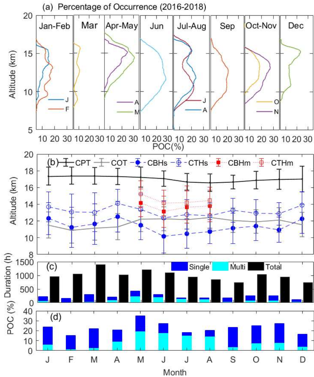
Figure 7: Monthwise variation of the altitude extent of the POC (top panels) and monthly variation of the peak altitude of the POC and CPT altitude.
