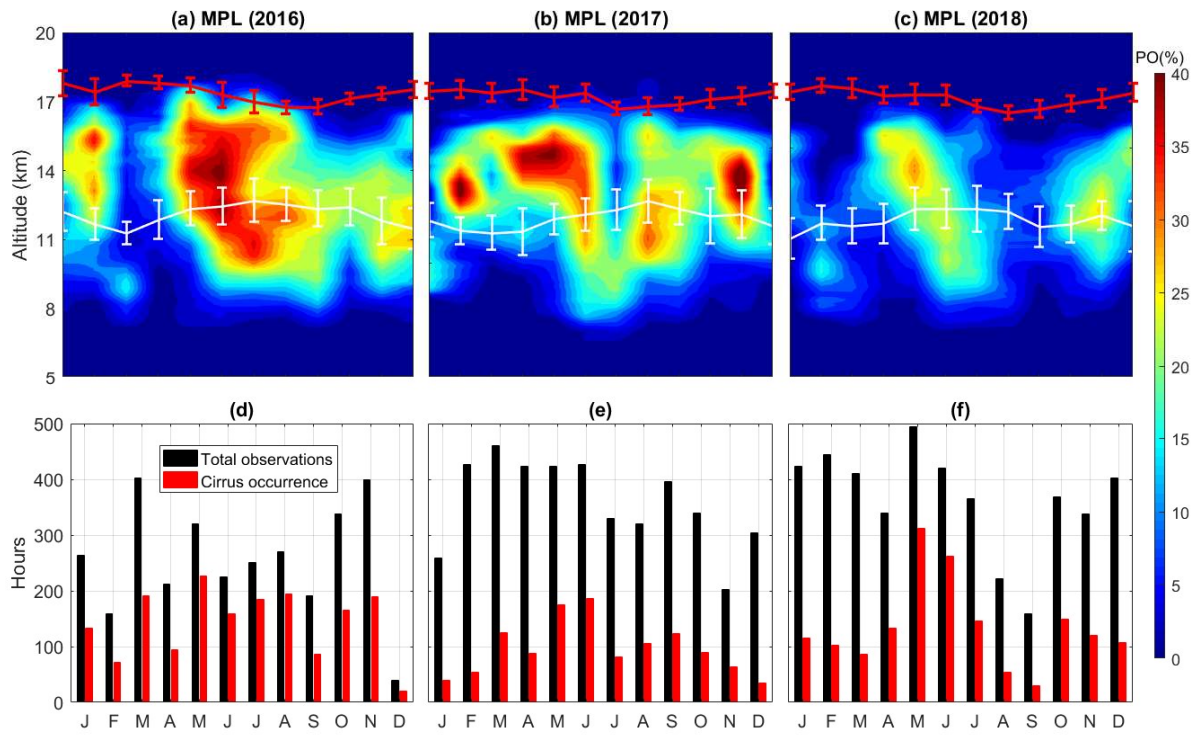
Figure 9: Monthly variation of the POC as a function of altitude during (a) 2016, (b) 2017 and (c) 2018. Monthly mean CPT altitude (red line) and COH (white line) with their standard deviations. (d-f) Total hours of lidar operation (black bars) and the available cirrus observation (red bars) for the corresponding year.
