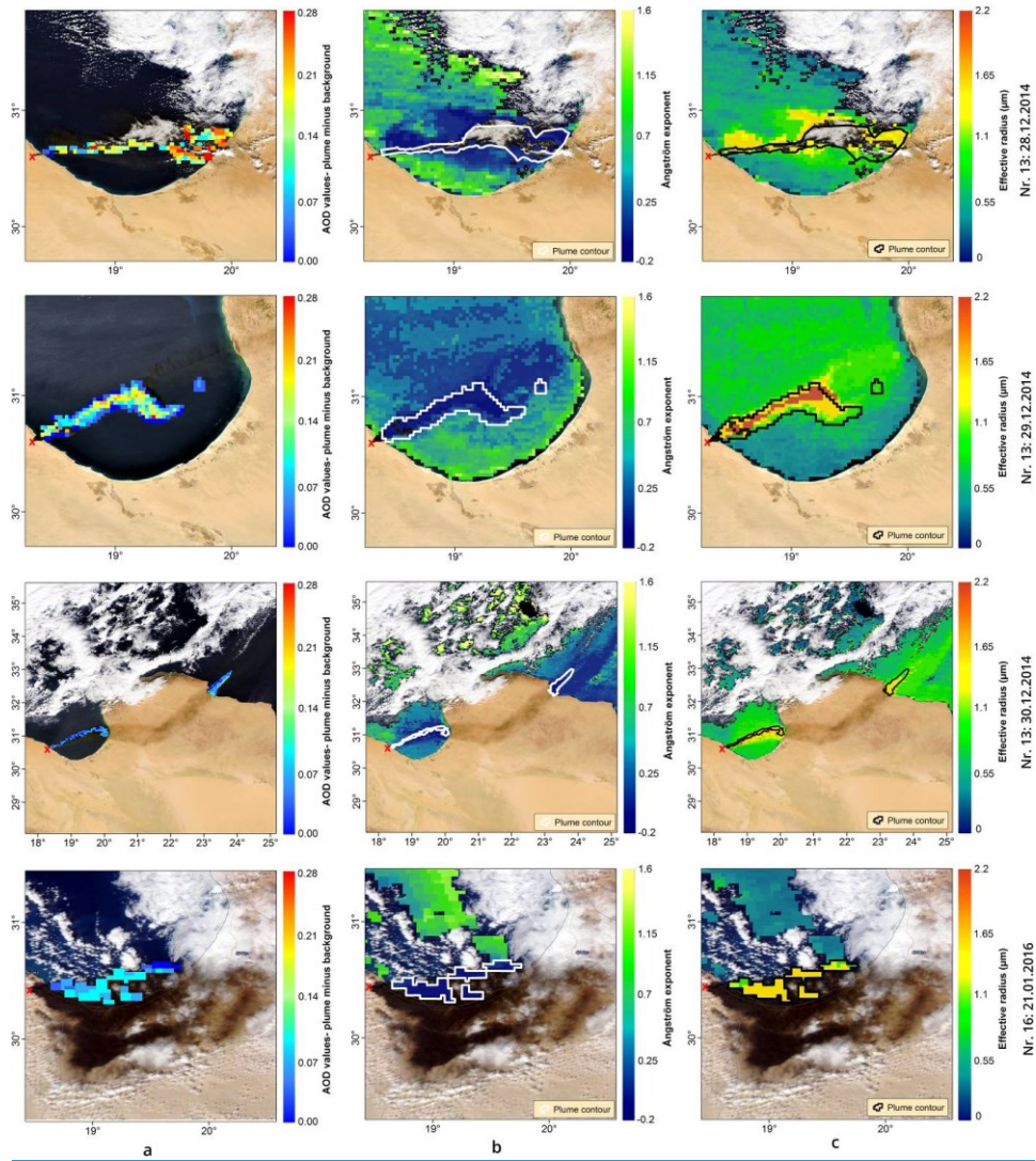
435 Figure 7. (a) Successful retrievals of aerosol properties for events 13 and 16. Plume specific AOD; (b) AE values for plume and the local background; (c) R_{eff} values for plume and the local background. The red coloured “x” indicates the event origin.
