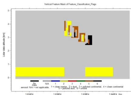
370 Figure 5 (a) Image of event 14 plume based on CALIPSO Total Attenuated Backscatter (532 nm) vs Lidar data altitude data; (b) Aerosol 375 feature classification; (c) cloud feature classification
