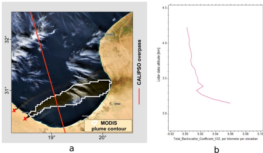
Figure 4 (a): CALIPSO overpass and MODIS plume contour; (b): Particulate backscatter coefficient profile CALIPSO level 2 (532 nm)
