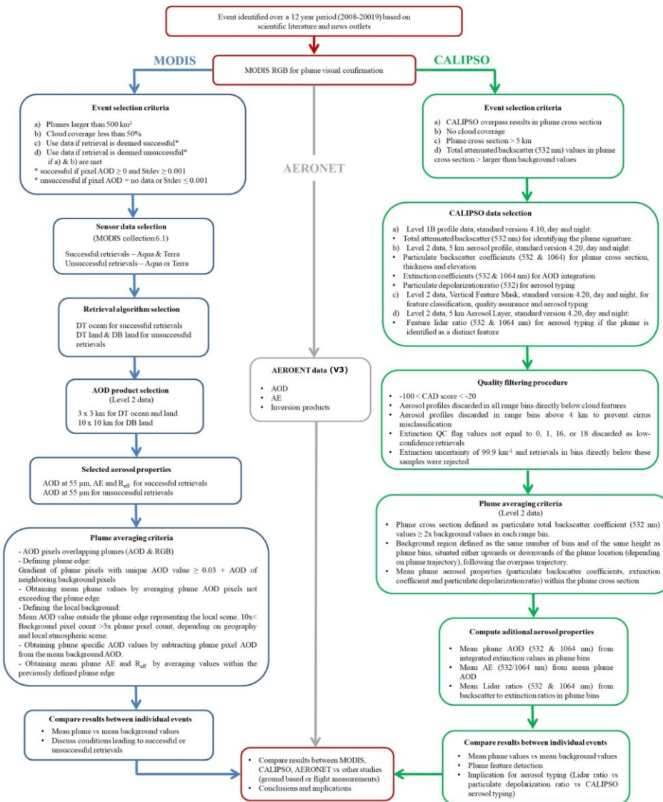
Flowchart of the plume analysis method
