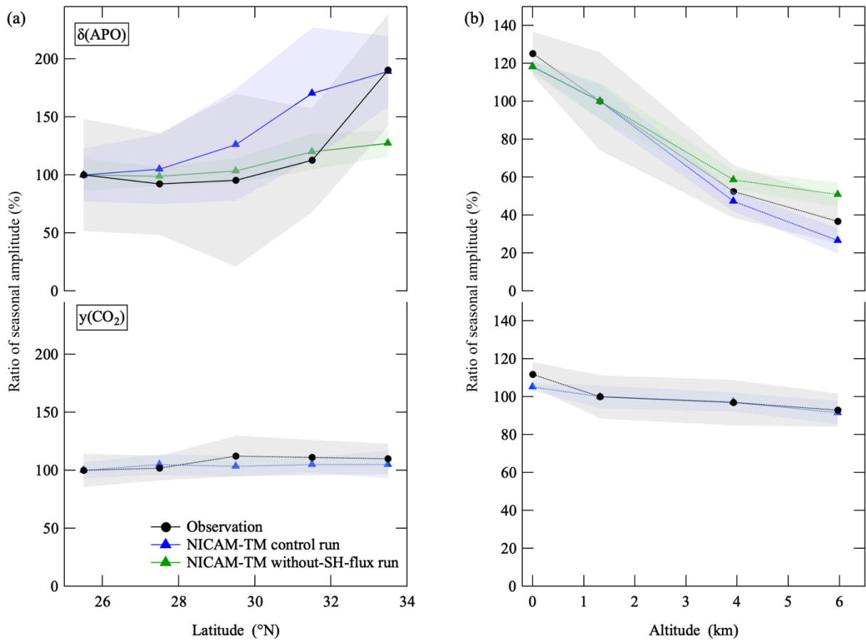
Figure 8: (a) Latitudinal distribution of average ratios of the observed seasonal \delta(\text{APO}) and \text{CO}_2 amount fraction amplitudes calculated relative to the values observed at 25.5^{\circ}\text{N} in the troposphere over the western North Pacific throughout the observation period (black filled circles). Error bands (shaded) indicate year-to-year variations ( \pm 1\sigma ). The corresponding results calculated using NICAM-TM control run (blue triangles) and without-SH-flux run (green triangles) are also shown. Amplitude of seasonal APO cycle was calculated as a difference between an average value during July to September and that during February to April considering its broad peak, while that of \text{CO}_2 amount fraction was evaluated as a difference between a seasonal maximum and minimum values. (b) Same as in (a) but for vertical distribution over MNM relative to the corresponding values at 1.3 km, and amplitude of seasonal APO cycle was evaluated as a difference between an average value during July to October and that during February to April. The average fractions of surface seasonal cycles obtained from continuous observations of \delta(\text{O}_2/\text{N}_2) and \text{CO}_2
