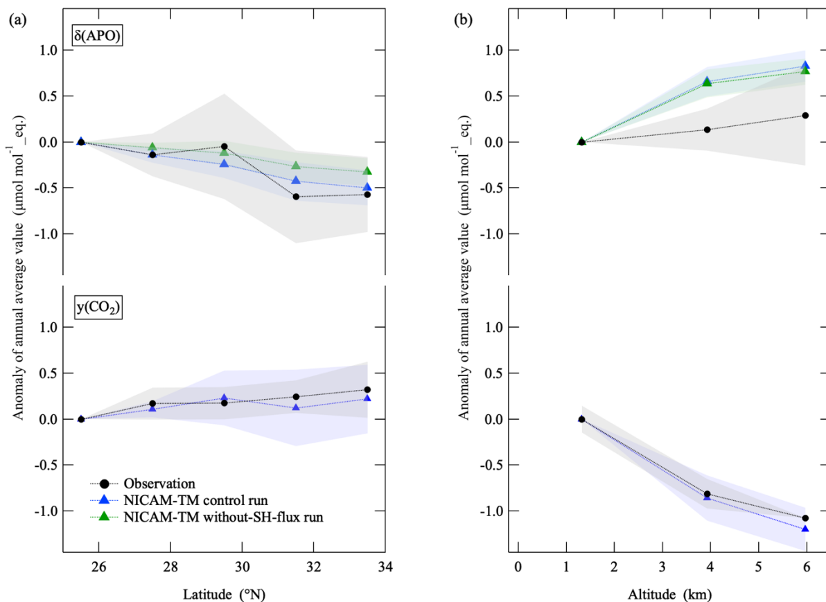
Figure 9: (a) Latitudinal distribution of average deviations of the annual mean values of \delta(\text{APO}) and \text{CO}_2 amount fraction relative to those at 25.5^{\circ}\text{N} in the troposphere over the western North Pacific throughout the observation period (black filled circles). Error bands (shaded) indicate year-to-year variations ( \pm 1\sigma ). The corresponding results calculated using NICAM-TM for control run (blue triangles) and without-SH-flux run (green triangles) are also shown. (b) Same as in (a) but for vertical distribution over MNM relative to the corresponding values at 1.3 km.
