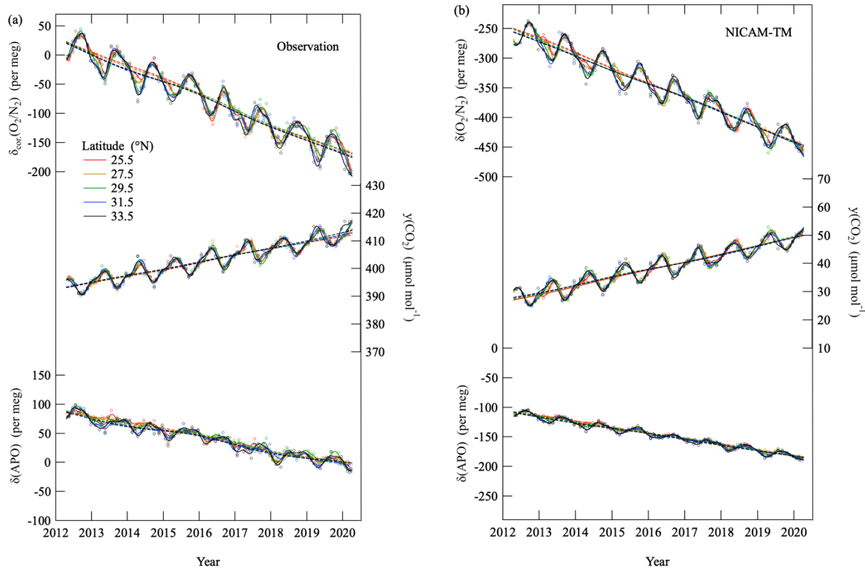
Figure 4: (a) \delta_{\text{cor.}}(\text{O}_2/\text{N}_2) , \text{CO}_2 amount fraction and \delta(\text{APO}) observed at the altitude of (6.1 \pm 0.5) (\pm 1\sigma) km at various latitudes over the western North Pacific. Best-fit curves to the data (solid lines) and secular trends (dashed lines) are also shown (Nakazawa et al., 1997). (b) Same as in (a) but for calculated values obtained from the NICAM-TM control-run. The data from NICAM-TM are reported on arbitrary scales different from those of observations.
