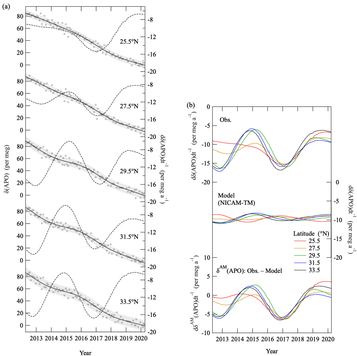
Figure 10: (a) Same secular trends in Fig. 4(a) and their annual change rates along with the deseasonalised values of \delta(\text{APO}) at each latitude over the western North Pacific. Error bands (shaded) indicate standard deviations of the deseasonalised \delta(\text{APO}) from the secular trends ( \pm 1\sigma ). (b) Same annual change rates in (a) (top). The corresponding change rates for the APO obtained from the control run of NICAM-TM (middle) and those of \delta^{\text{AM}}(\text{APO}) obtained by subtracting the calculated \delta(\text{APO}) from the observed \delta(\text{APO}) (bottom) are also shown.
