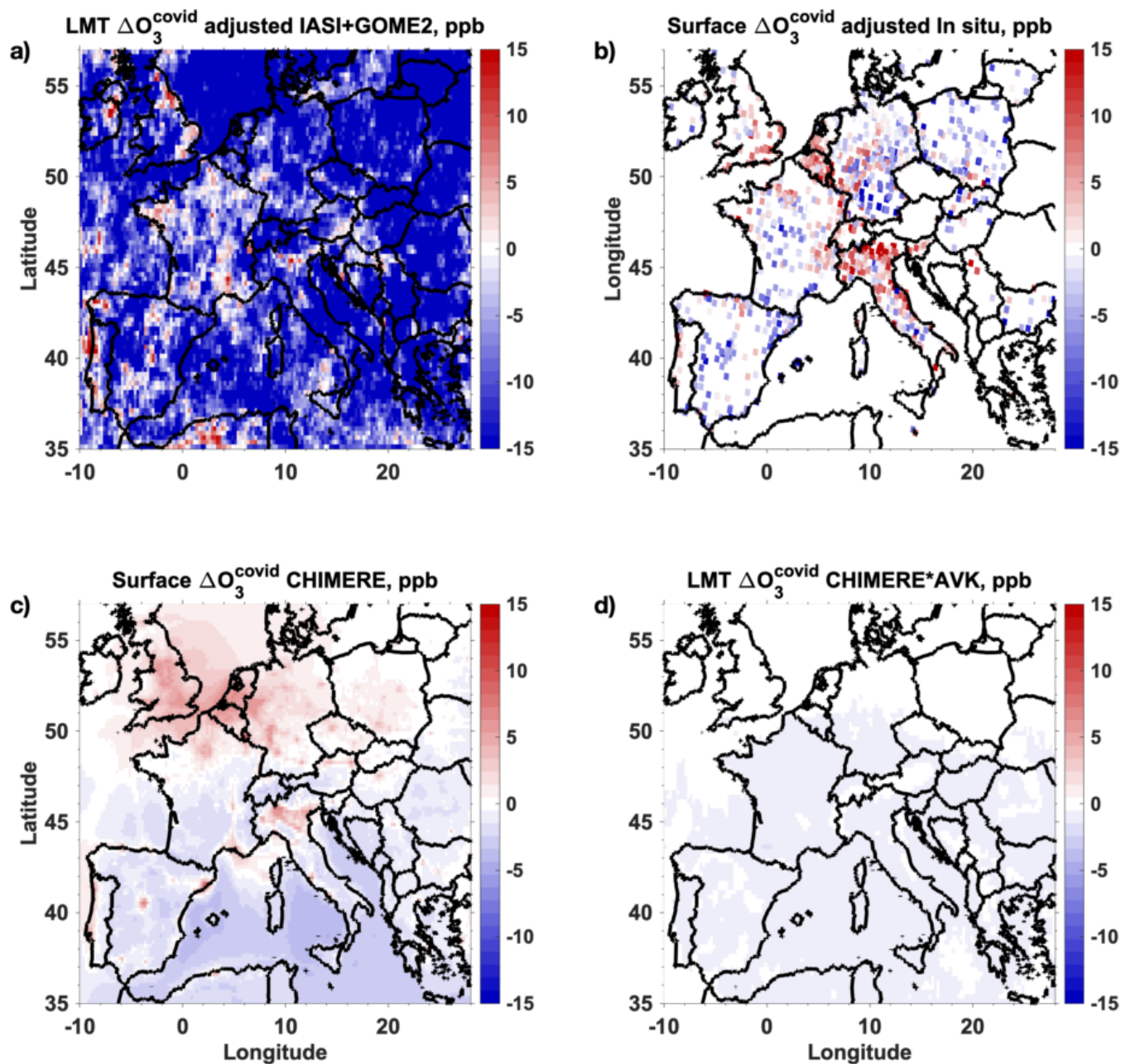
740 Figure 5. Changes in ozone pollution (ppb) associated with the pandemic lockdown in 1-15 April 2020, derived from adjusted observations (using Eq. 1) for avoiding the influence of meteorological conditions at (a) the lowermost troposphere (LMT, < 3 km asl) retrieved with IASI+GOME2 multispectral satellite approach and the surface, (b) measured by in situ sensors and simulated by the CHIMERE model (c) at the surface and (d) at the LMT smoothed by IASI+GOME2 averaging kernels.
