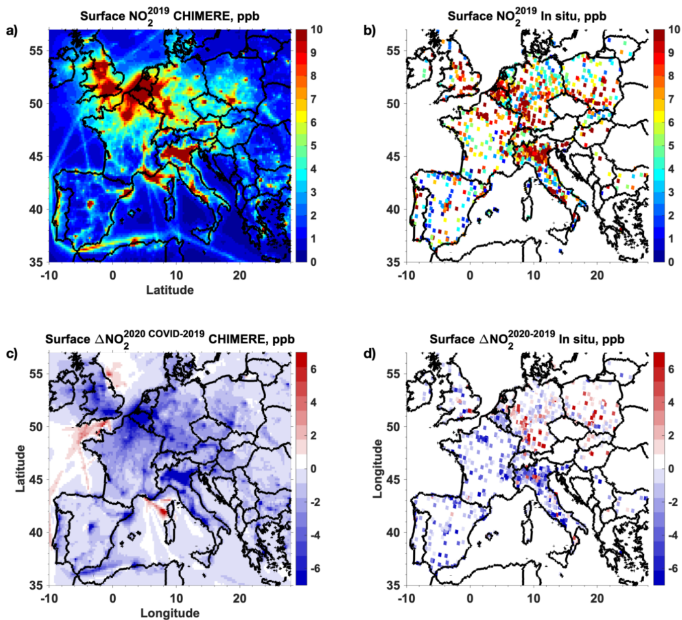
Figure 6. Surface \text{NO}_2 concentrations (ppb) averaged over the period 1-15 April 2019 (a) simulated by the CHIMERE and (b) measured by in situ sensors. (c) Idem of (a), (d) of (b) but for changes between 1-15 April 2020 with respect to the same period in 2019.
