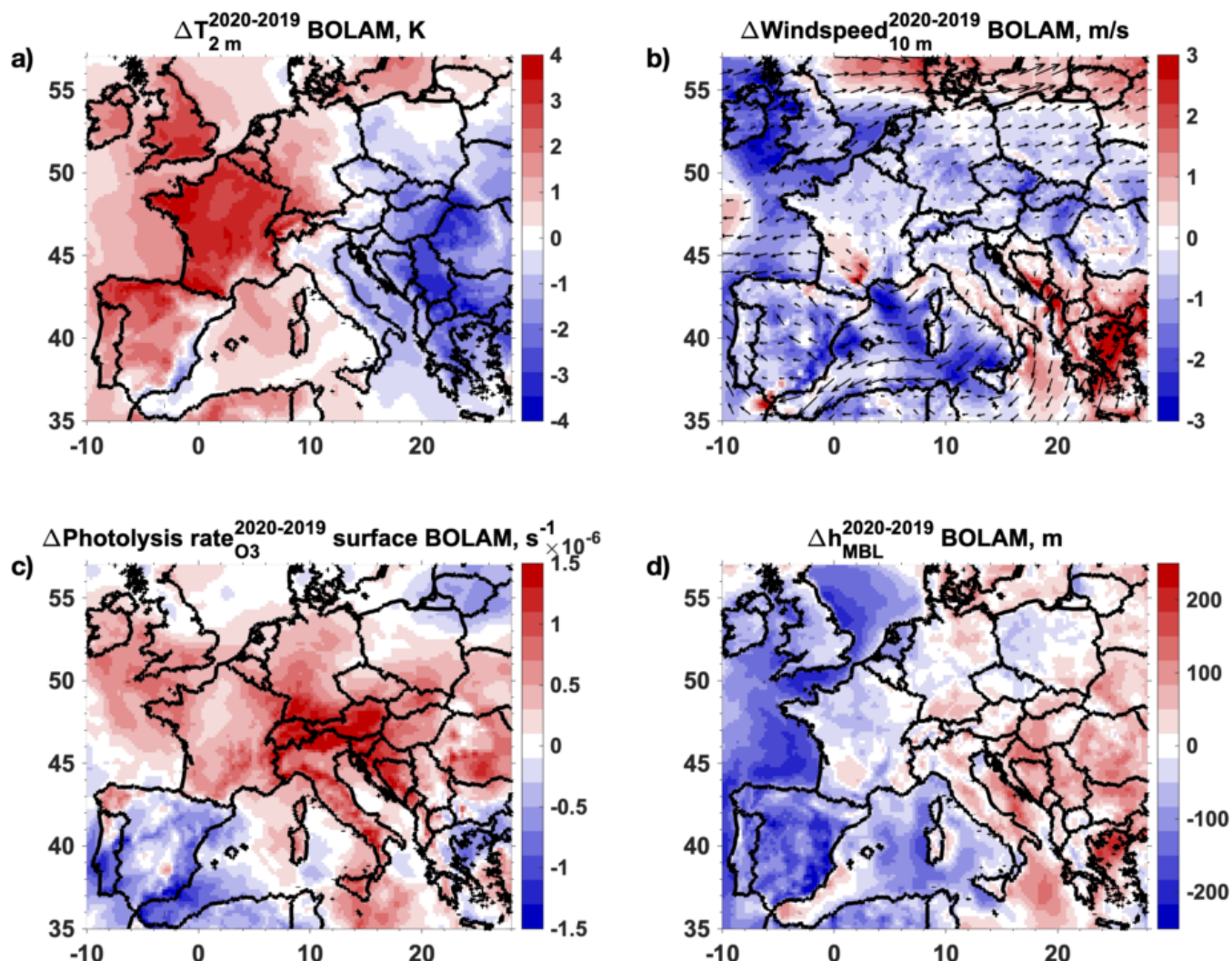
Figure 7. Changes in (a) Temperature at 2 m (K), (b) Windspeeds (m/s) and wind vectors, (c) Ozone photolysis rates (s -1 ) and (d) Height of the mixing boundary layer (m) averaged over the period 1-15 April 2020 with respect to the same period in 2019
