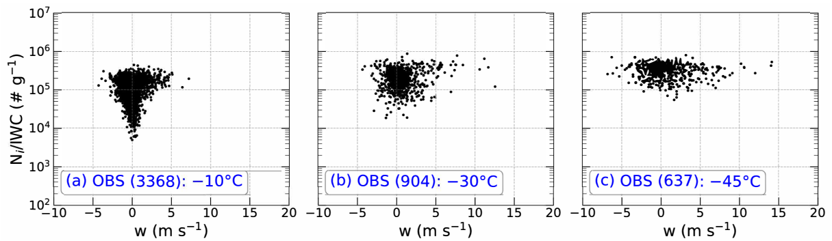
Figure 3. Scatter plots of observed ice number concentration ( N_i , \# m^{-3} ) divided by ice water content (IWC, g m^{-3} ) (denoted as N_i/IWC ) as a function of vertical velocity ( w , m s^{-1} ) in regions with IWC > 1 g m^{-3} from all flights during the Cayenne field campaign at temperatures of (a) -10^\circ C , (b) -30^\circ C , and (c) -45^\circ C , and the observed temperature ranges of samples at the three levels are -12.9 to -7.3^\circ C , -33.0 to -27.3^\circ C , -45.4 to -42.4^\circ C , respectively. The numbers in parentheses represent the total number of samples.
