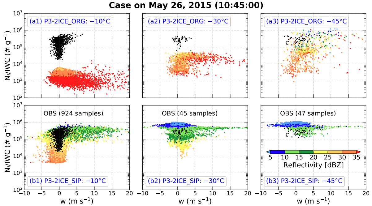
Figure 9. Scatter plots of (black) observed and (colorized) simulated ice number concentration ( N_i , \# m^{-3} ) divided by ice water content (IWC, g m^{-3} ) (denoted as N_i/IWC ) as a function of vertical velocity ( w , m s^{-1} ) in regions with IWC > 1 g m^{-3} at temperatures of (a1, b1) -10^\circ C , (a2, b2) -30^\circ C , and (a3, b3) -45^\circ C . The observations are from the two flights, SAFIRE Falcon 20 and NRC Convair 580 (shown in Fig. 1 of Huang et al. (2021)), during the Cayenne field campaign, and the observed temperature ranges of samples at the three levels are -12.6 to -7.9^\circ C , -30.4 to -29.7^\circ C , -44.7 to -43.6^\circ C , respectively. The simulation using the original P3 two-ice category configuration is shown in a1–a3, and the simulation using the P3 two-ice category configuration including the three SIP processes is shown in b1–b3. The simulations at the three temperature levels are interpolated from the 1-km model outputs. The scatters of simulations are color-coded according to the magnitude of radar equivalent reflectivity factor (dBZ).
