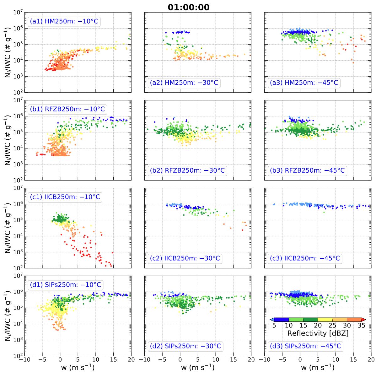
Figure 6. As Fig. 4 but for experiments (a1–a3) HM250m, (b1–b3) RFZB250m, (c1–c3) IICB250m, and (d1–d3) SIPs250m, respectively. The acronyms HM, RFZB, IICB and SIPs represent Hallett–Mossop process, raindrop freezing breakup, ice-ice collision breakup, secondary ice production processes, respectively.
