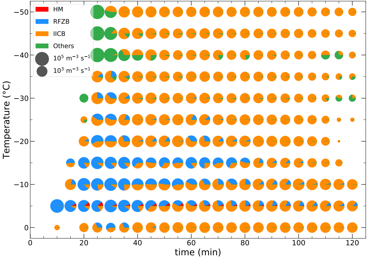
Figure 8. Time evolution of the averaged microphysical process rates relevant for ice particle production processes including (red) H-M mechanism, (blue) shattering of freezing droplets, (orange) fragmentation of ice–ice collision, and (magenta/green) other microphysical processes (i.e., ice nucleation, homogeneous and heterogeneous freezing of cloud droplets and rain) in regions with IWC > 1 \text{ g m}^{-3} at different temperatures. The pie charts denote ice particle production rates summed over all the source terms with the area of each color proportional to the ice particle production rate.
