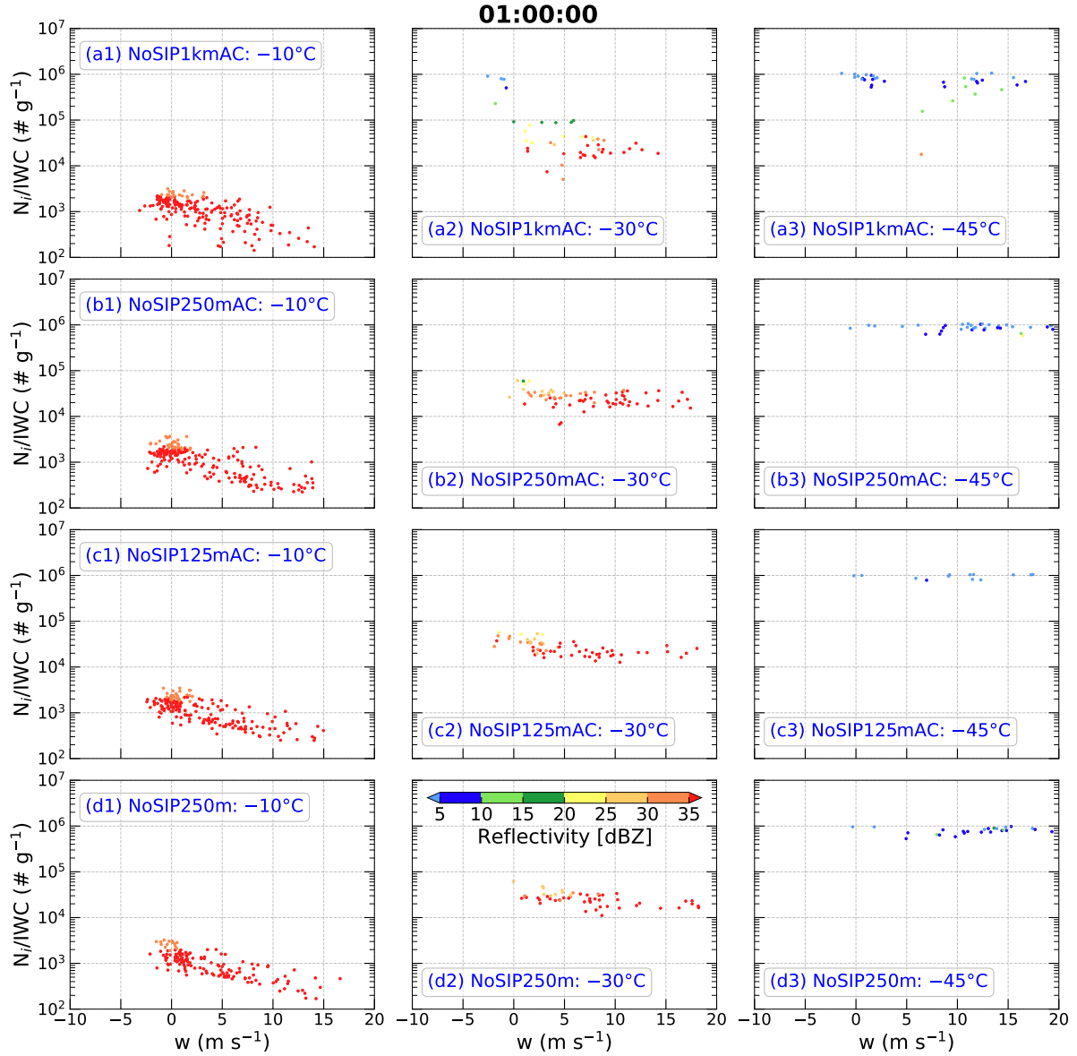
Figure 4. Scatter plots of simulated ice number concentration ( N_i , \# m^{-3} ) divided by ice water content (IWC, g m^{-3} ) (denoted as N_i/IWC ) as a function of vertical velocity ( w , m s^{-1} ) in regions with IWC > 1 g m^{-3} at temperatures of (left column) -10^\circ C , (middle column) -30^\circ C , and (right column) -45^\circ C at t = 60 min in experiments (a1–a3) NoSIP1kmAC, (b1–b3) NoSIP250mAC, (c1–c3) NoSIP125mAC, and (d1–d3) NoSIP250m, respectively. The simulations at the three temperature levels are interpolated from the model outputs. The simulations with horizontal grid spacing < 1 km have been coarsened to 1 km for comparison by spatially averaging with a window size of 1 km \times 1 km . The points are color-coded according to the magnitude of radar equivalent reflectivity factor (dBZ).
