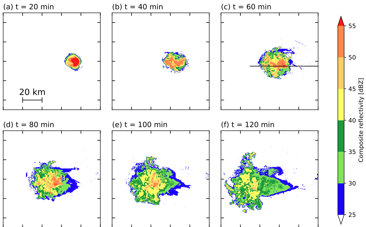
Figure 2. Composite reflectivity (dBZ) in SIPs250m at (a–f) t = 20, 40, 60, 80, 100, and 120 min, respectively. The black solid line in (c) indicates the location of cross section shown in Fig. 7. Tick marks are included every 20 km.
