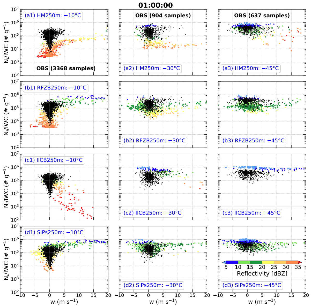
Figure A2. As Fig. 6 but overlaid with observations in Fig. 3.
