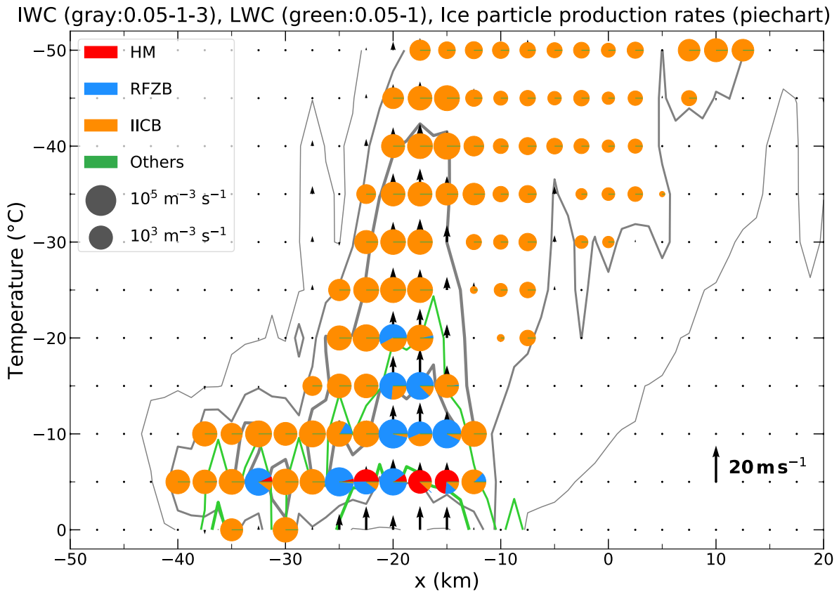
Figure 7. Vertical cross section along the line aligned along X shown in Fig. 2c of IWC (gray contours: 0.05, 1, and 3 \text{ g m}^{-3} from thin to the thick), LWC (green contours: 0.05, and 1 \text{ g m}^{-3} from thin to the thick), vertical velocity (vertical vectors), and the microphysical process rates relevant for ice particle production processes including (red) H-M mechanism, (blue) shattering of freezing droplets, (orange) fragmentation of ice-ice collision, and (magenta/green) other microphysical processes (i.e., ice nucleation, homogeneous and heterogeneous freezing of cloud droplets and rain) in regions with \text{IWC} > 1 \text{ g m}^{-3} at different temperatures in SIPs250m at t = 60 \text{ min} . The pie charts denote ice particle production rates summed over all the source terms with the area of each color proportional to the ice particle production rate.
