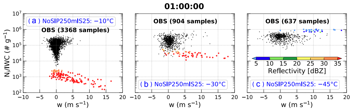
Figure 5. As Fig. 4 but for the experiment NoSIP250mIS25 overlaid with observations in Fig. 3.
