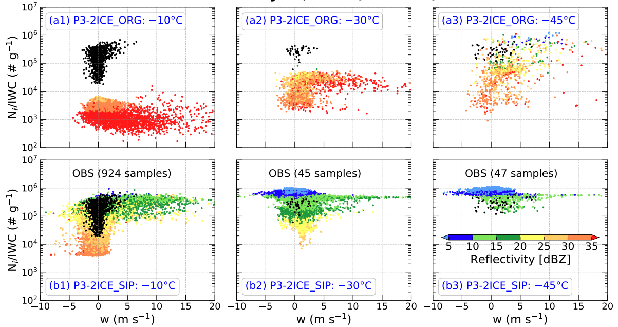
Figure 9. Scatter plots of (black) observed and (colorized) simulated ice number concentration ( N_i , \# m^{-3} ) divided by ice water content (IWC, g m^{-3} ) (denoted as N_i/IWC ) as a function of vertical velocity ( w , m s^{-1} ) in regions with IWC > 1 g m^{-3} at temperatures of (a1, b1) -10^\circ C , (a2, b2) -30^\circ C , and (a3, b3) -45^\circ C . The observations are from the two flights, SAFIRE Falcon 20 and NRC Convair 580 (shown in Fig. 1 of Huang et al. (2021)), during the Cayenne field campaign, and the observed temperature ranges of samples at the three levels are -12.6 to -7.9^\circ C , -30.4 to -29.7^\circ C , -44.7 to -43.6^\circ C , respectively. The simulation using the original P3 two-ice scheme-category configuration is shown in a1–a3, and the simulation using the P3 two-ice scheme-category configuration including the three SIP processes is shown in b1–b3. The simulations at the three temperature levels are interpolated from the 1-km model outputs. The scatters of simulations are color-coded according to the magnitude of radar equivalent reflectivity factor (dBZ).
