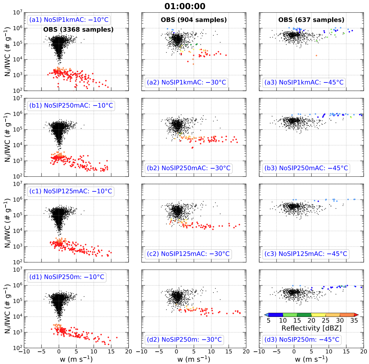
Figure A1. As Fig. 4 but overlaid with observations in Fig. 3.
