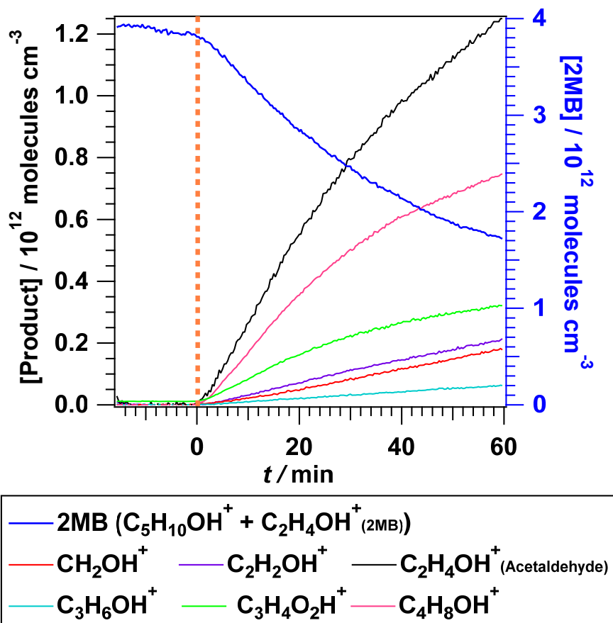
370 Figure 8. Temporal evolution of 2-methylbutanal (sum of the 2 identified ions) and the most abundant products measured by PTR-ToF-MS during the 2-methylbutanal + Cl reaction. Vertical dashed line indicates when UV lamps are switched on.
