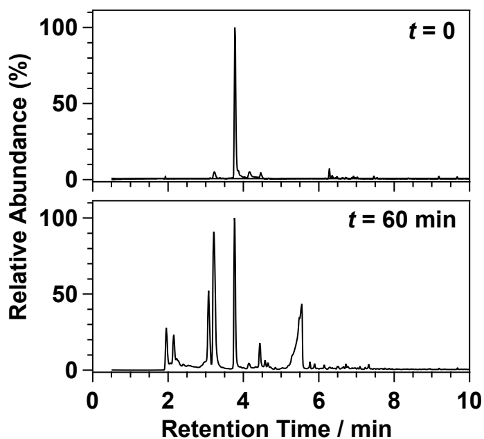
330 Figure 6. Chromatograms obtained for a 2MB/Cl 2 mixture before irradiation (top panel) and after 60 min of irradiation (bottom panel).
