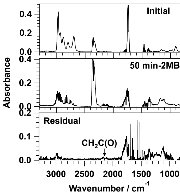
350 Figure 7. FTIR spectra used in the identification of the products in the Cl reaction of 2MB. The top panel shows the initial spectrum, the central panel shows the spectrum obtained after 50 min of Cl reaction, with the features of 2MB subtracted, and the bottom panel shows the residual spectrum after the subtraction of reaction products shown in the SI (Figure S6).
