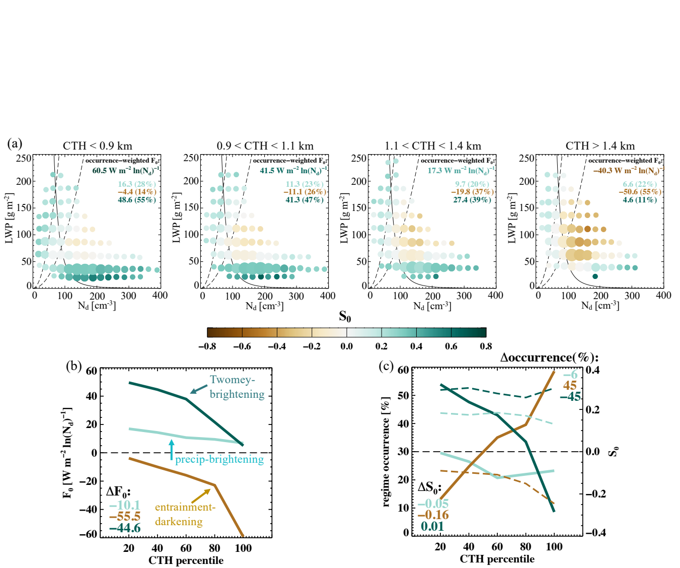
Figure 6. a ) as in Fig. 3, but conditioned on cloud top height (CTH) quartiles. Occurrence-weighted mean b ) F 0 and c ) regime-mean S 0 (dashed curves) and regime-occurrence (solid curves) of the 3 albedo susceptibility regimes (defined in Fig. 3) as a function of CTH, increment of 20 percentile.
