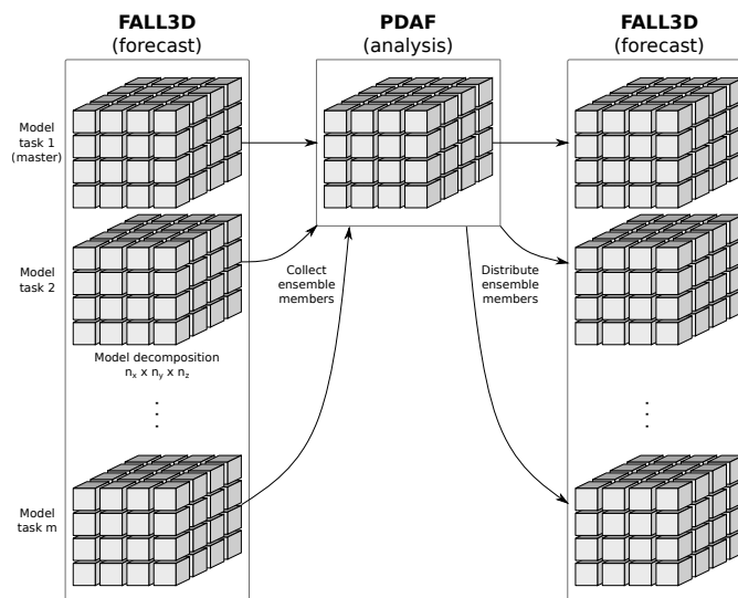
Figure 1. Scheme of the ensemble-based data assimilation system implemented in the FALL3D dispersal model. The system builds upon an efficient implementation by coupling FALL3D and the Parallel Data Assimilation Framework (PDAF) and uses a two-level parallelisation scheme based on MPI (Message Passing Interface).
