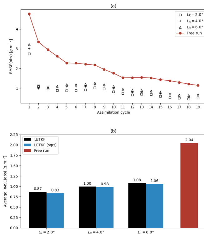
Figure 7. RMSE o computed in the observation space for the Raikoke experiment: (a) time series of RMSE o at analysis times for the free (red line) and LETKF runs for different localisation radius ( L_R = 2^\circ , L_R = 4^\circ and L_R = 6^\circ ) and (b) same with time-averaged values.
