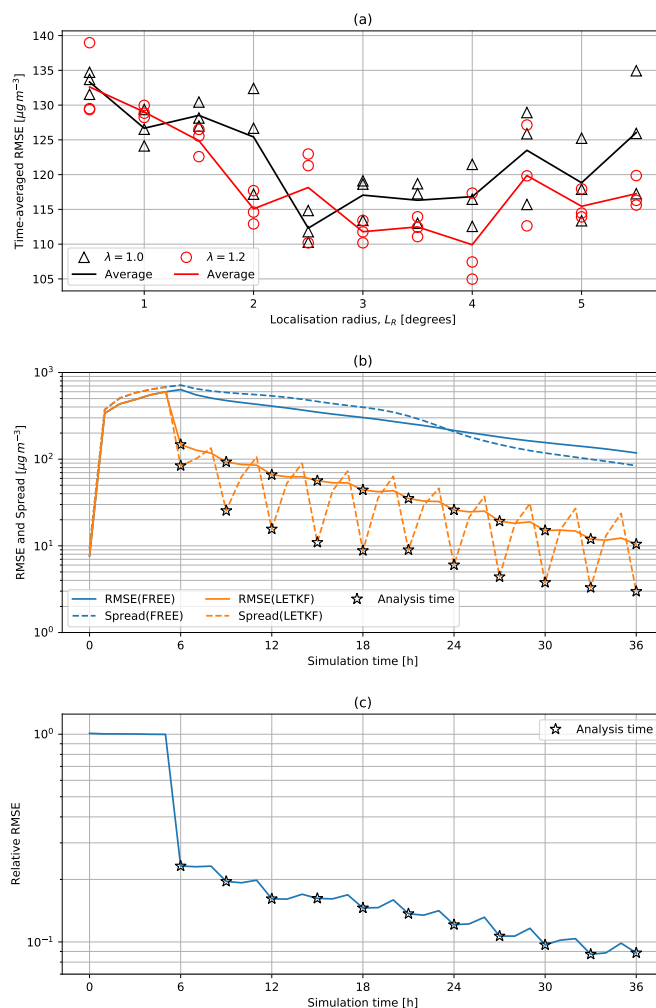
Figure 5. Evaluation metrics used for the twin experiment: (a) Time-averaged RMSE computed for different filter configurations and three ensemble realisations. Best performance was obtained for localisation radius, L_R , in the range 2\text{--}4^\circ and an inflation factor of \lambda = 1.2 ; (b) Temporal evolution of ensemble spread and RMSE for the FREE and LETKF runs; and (c) Time series of LETKF-to-FREE ratio of RMSE. Assimilation times are stated by star symbols.
