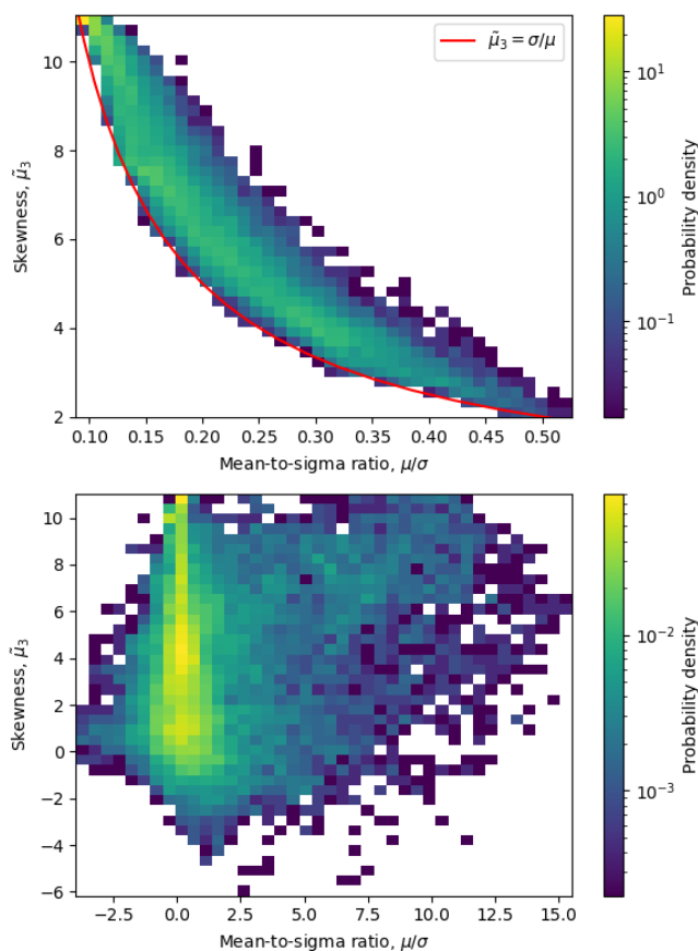
Figure 2. Two-dimensional histogram plot for the prior (top) and analysis (bottom) distributions showing the probability density for skewness ( \tilde{\mu}_3 ) and mean-to-sigma ratio ( \mu/\sigma ) values, where \mu refers to ensemble mean and \sigma to standard deviation. Results correspond to the first assimilation cycle of the Raikoke experiment.
