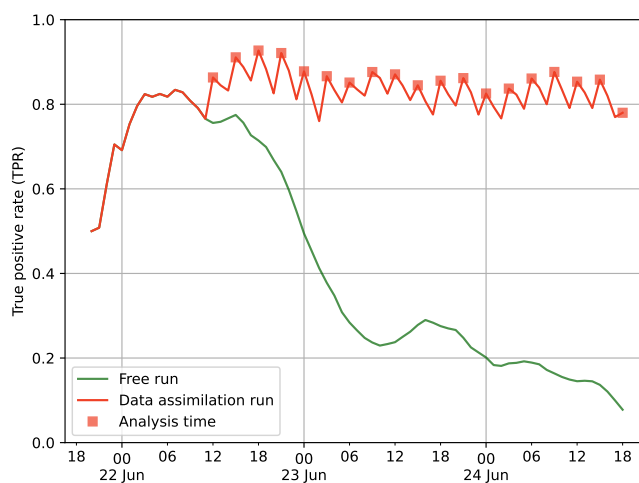
Figure 11. Temporal evolution of the Probability of Detection (POD) metrics according to the free and data assimilation runs for the Raikoke experiment. A localisation radius of L_R = 2^\circ was defined for the data assimilation simulation.
