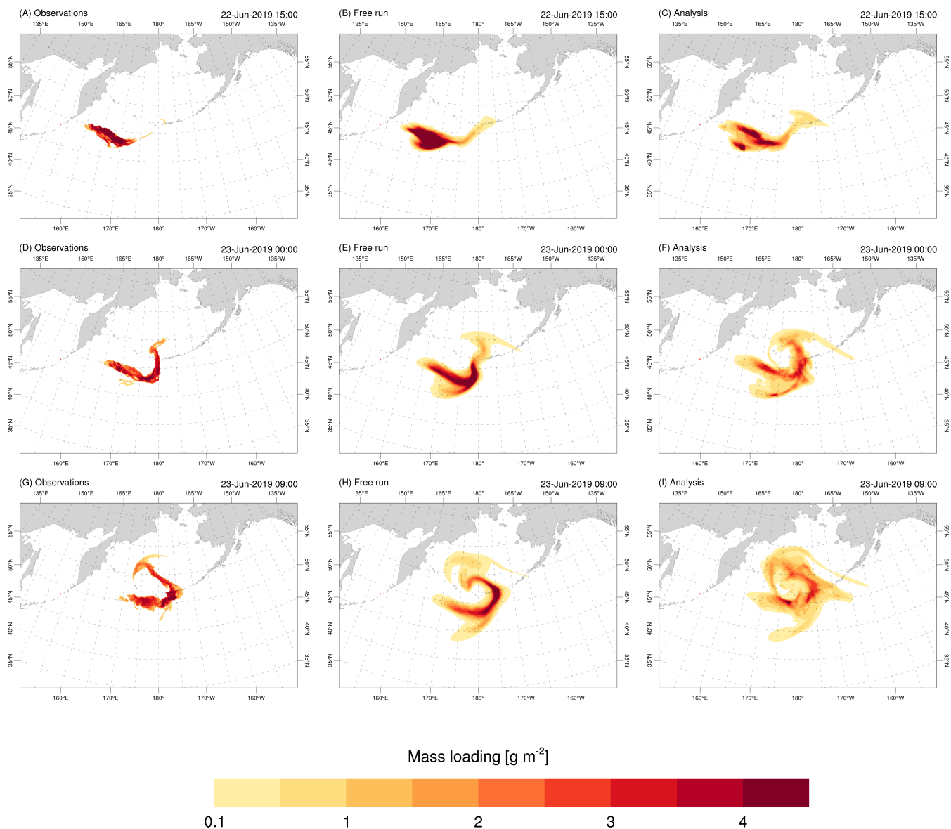
Figure 6. Spatial distribution of \text{SO}_2 mass loading at different time instants: (A-C) 22 June at 15:00 UTC, (D-F) 23 June at 00:00 UTC, and (G-I) 23 June at 09:00 UTC. The column panels show: observations (left panel), free run (central panel), and analysed mass loading (right panel).
