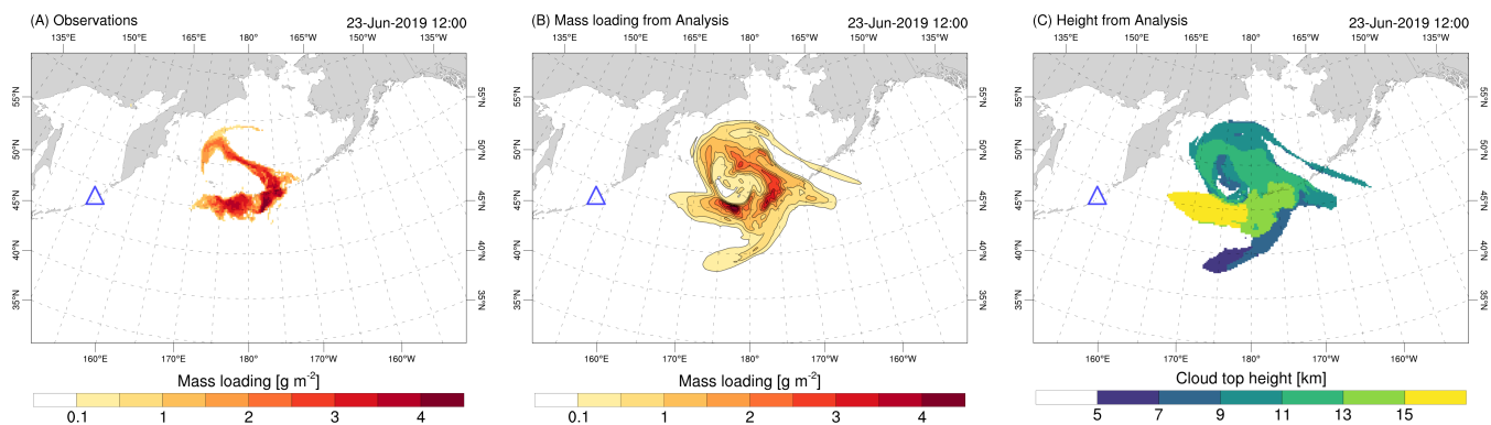
Figure 9. SO 2 cloud for the 2019 Raikoke eruption on 23 June at 12:00 UTC. Observed (a) and modelled (b) mass loading are compared at the same instant of time. In addition, the cloud top height (c) derived from the analysed state is also shown. The LETKF run was configured assuming a localisation radius of L_R = 2^\circ and an assimilation frequency of 3h, starting on 22 June 2019 at 12:00 UTC.
