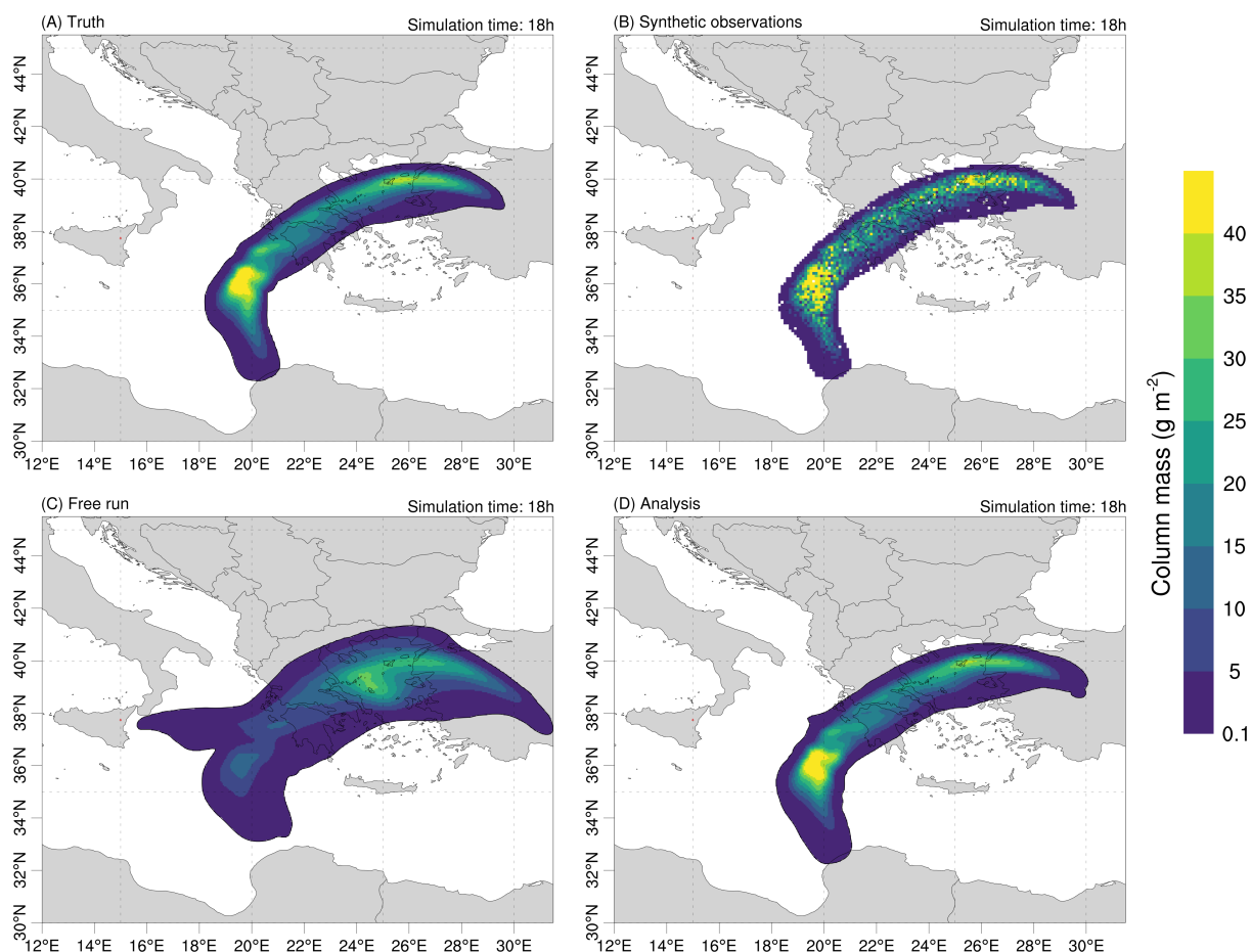
Figure 4. Spatial distribution of ash mass loading for the twin experiment at t = 18 h after eruption start. The true state (a) given by a single run assumes a time-varying emission. Synthetic observations (b) are generated from the truth by adding a Gaussian noise and assuming an observation error variance of 40%. The impact of the LETKF DA becomes evident by comparing results from the free ensemble run without assimilation (c) with the analysed mass loading (d).
