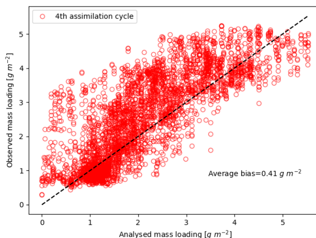
Figure 8. Comparison of SO 2 mass loading observations and the analysis state at the fourth assimilation cycle. In general, analysis underestimates observations. In this case, an average bias of 0.41 \text{ g m}^{-2} was found.
