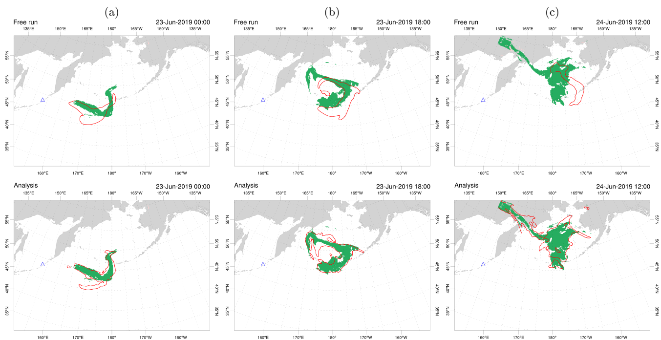
Figure 10. Maps of 1 \text{ g m}^{-2} contour of SO 2 mass loading according to observations (green shaded area) and model (solid red line) for different instants of time: (a) 00:00 UTC on 23 June 2019, (b) 18:00 UTC on 23 June 2019, and (c) 12:00 UTC on 24 June 2019. Model results corresponding to the free run (top panel) and the analysis (bottom panel) are compared. A localisation radius of L_R = 2^\circ was defined for the data assimilation method.
