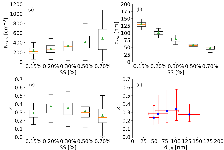
Figure 5. Boxplots of N_{CCN} (a), d_{crit} (b) and \kappa (c) at supersaturations (SS) from 0.15% to 0.70% based on all available data . Whiskers show the 90th to 10th percentiles. Green solid triangles show the mean values. (d) \kappa as a function of d_{crit} . Error bars of d_{crit} show 1 standard deviation. Error bars of \kappa show 1 geometric standard deviation.
