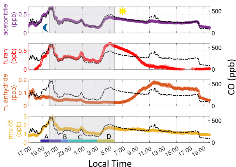
100 Figure 2: VOCs and CO on 3 – 4 Feb 2020 with the shaded area representing sunset to sunrise. The peak in CO after sunset (start of gray-shaded area) is used to denote the beginning of the smoke event. We limit our analysis to sunrise on the following day. The color labels A-D indicate individual times used to calculate ERs (see section 5.2 in main text).
