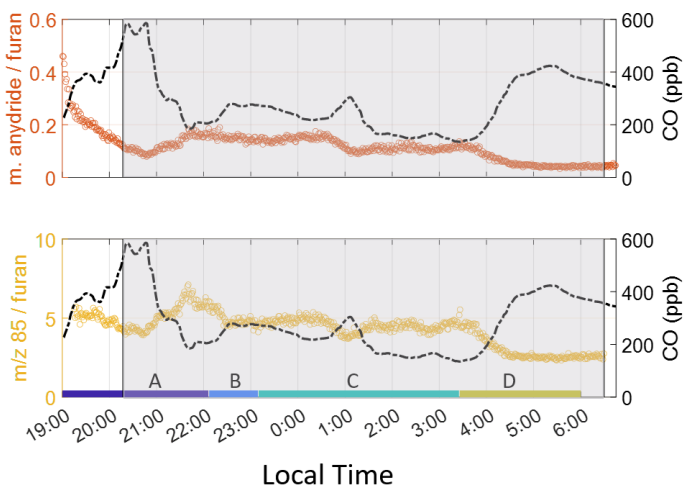
105 Figure 3: Product-to-reactant ratio for furan oxidation products. Both ratios indicate the period just before sunrise is least oxidized. Again, the color labels A-D indicate individual times used to calculate ERs.
