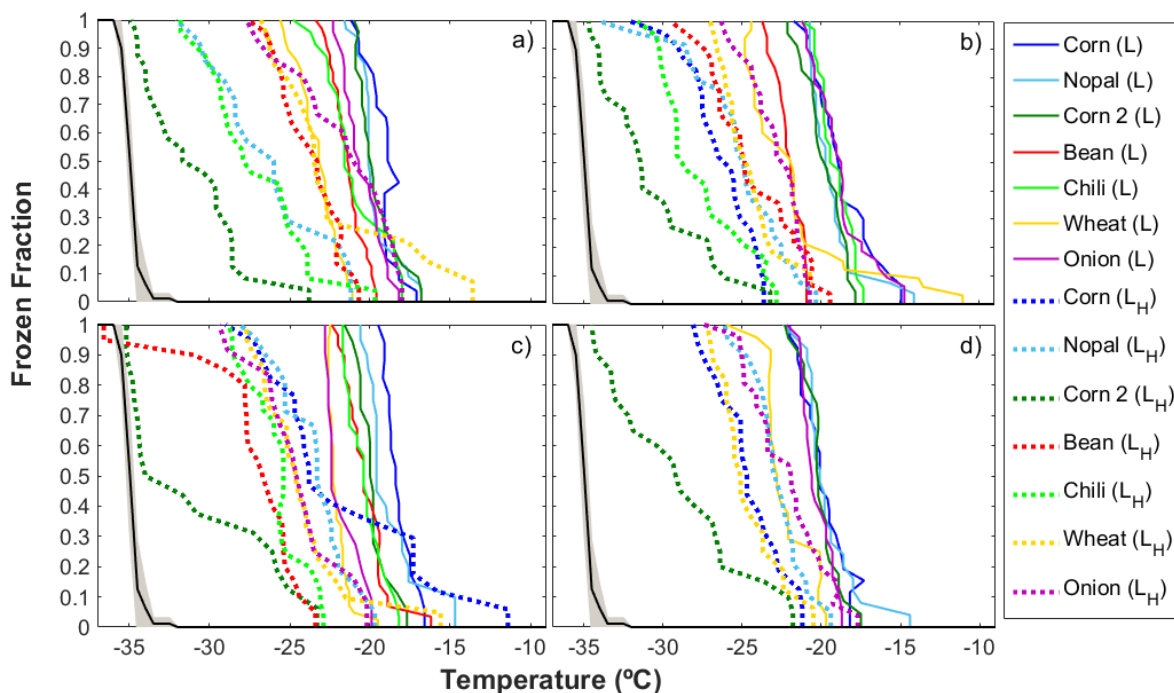
660 Figure 5: Ice nucleating abilities of agricultural dust particles generated in the laboratory (L) before and after the heating treatment as a function of temperature and particle size a) 3.2-5.6 \mu\text{m} , b) 1.8-3.2 \mu\text{m} , c) 1.0-1.8 \mu\text{m} , and d) 0.56-1.0 \mu\text{m} . The black line (Homo. frez.) depicts the average homogeneous freezing curve. The dashed and solid lines show the results of the heated samples (H) and non-heated samples, respectively. For the heating treatment, the samples were heated at 300°C for 2 h.
