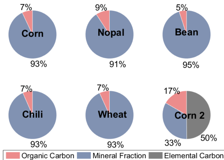
655 Figure 4: Organic carbon, elemental carbon and mineral contribution of the aerosol samples generated in the laboratory.
