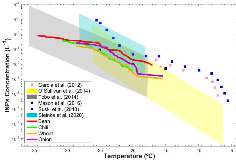
Figure 7: Inter-comparison of the INP concentrations as a function of temperature from the present study (colored solid lines) and literature data (blue, gray, and yellow area, and filled symbols).
