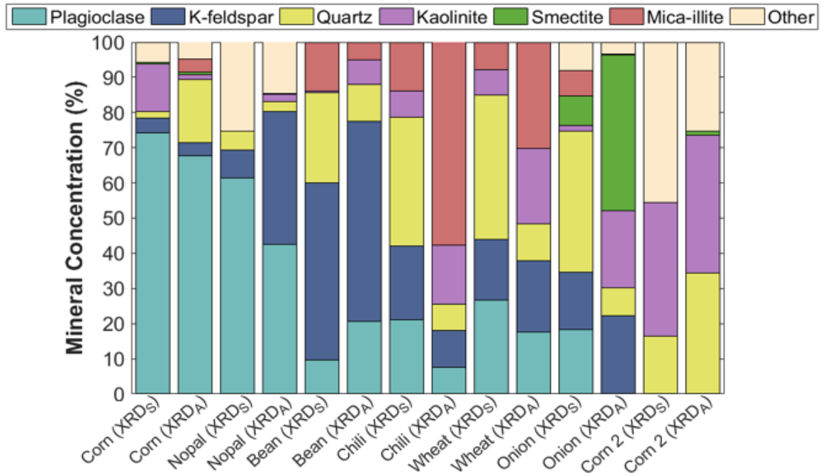
Figure 6: Summary of the mineralogical composition of the aerosol particles generated in the laboratory for dp=0.18 to 10 \mu\text{m} (XRD A ), and soil samples collected in the field for particle size <425 \mu\text{m} (XRD s ). The mineral phases were identified using X-ray diffraction (XRD).
