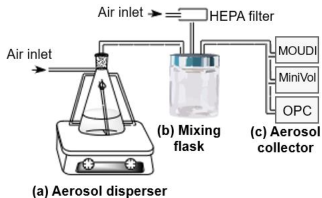
Figure 2: Dry aerosol generation system setup. (a) aerosol disperser, (b) mixing volume, and (c) aerosol collector (MOUDI 100R, MiniVol TAS or OPC).
