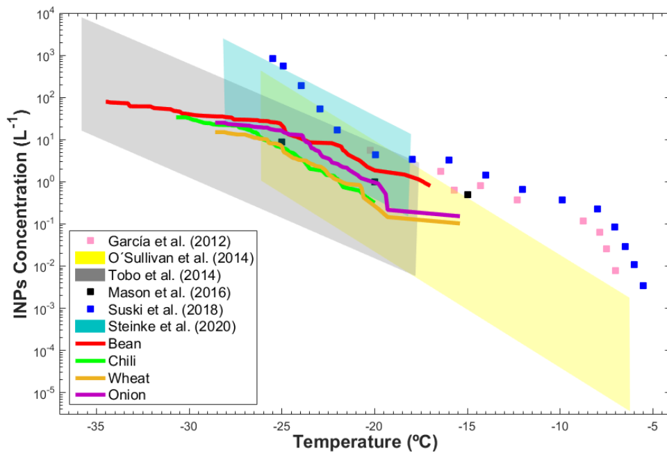
670 Figure 7: Inter-comparison of the INP concentrations as a function of temperature from the present study (colored solid lines) and literature data (blue, gray, and yellow area, and filled symbols).
