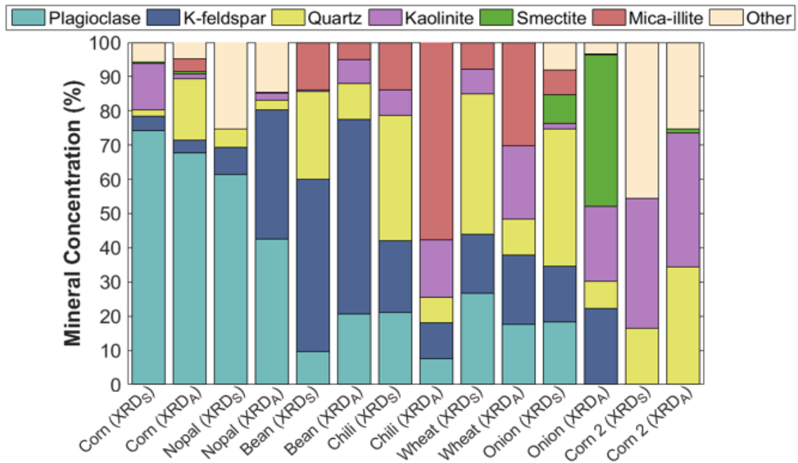
665 Figure 6: Summary of the mineralogical composition of the aerosol particles generated in the laboratory for dp=0.18 to 10\ \mu\text{m} ( \text{XRD}_A ), and soil samples collected in the field for particle size <425\ \mu\text{m} ( \text{XRD}_S ). The mineral phases were identified using X-ray diffraction (XRD).
