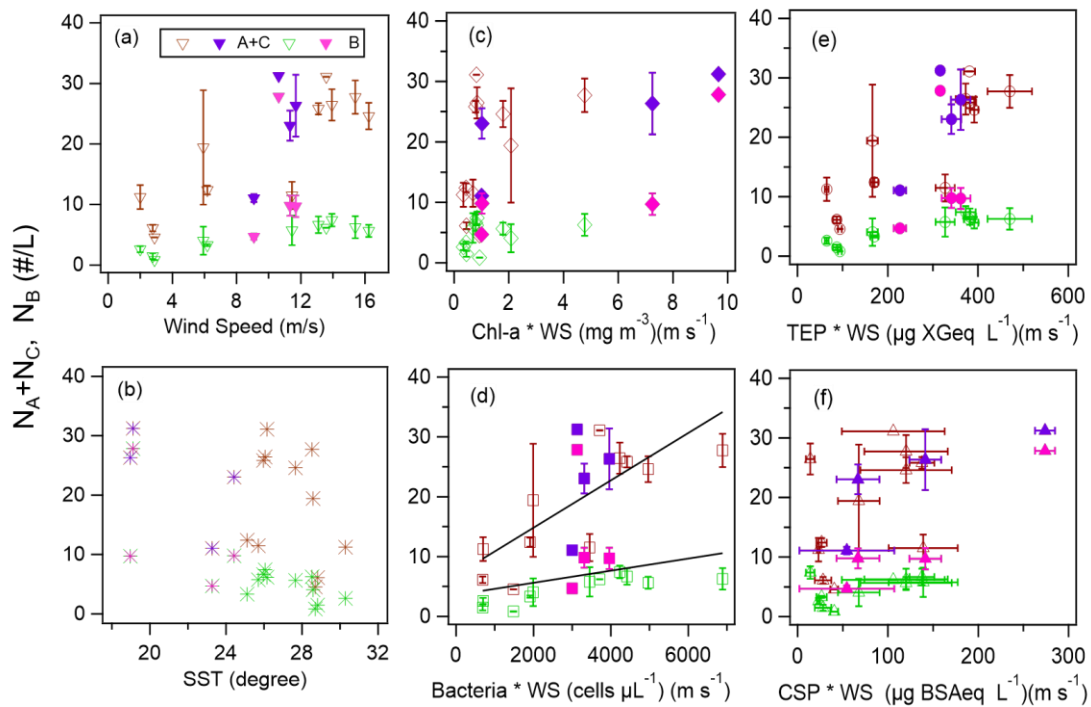
Figure 8. Number concentrations of Type A+C and Type B particles and (a) wind speed, (b) SST, (c) product of wind speed (WS) and Chl- a concentration, (d) product of WS and bacteria concentration, (e) product of W and TEP concentration, and (f) product of WS and CSP concentration. Open markers indicate Period 1 and solid markers indicate Period 2. The black lines in Fig. 8d are orthogonal regression lines for all Type A+C data and for all Type B data as an example. The error bars represent one standard deviation.
