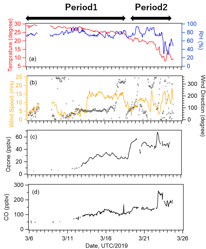
Figure 2. Time series of meteorological parameters: (a) air temperature and relative humidity, (b) wind speed and direction. Time series of concentrations of (c) ozone and (d) carbon monoxide.
