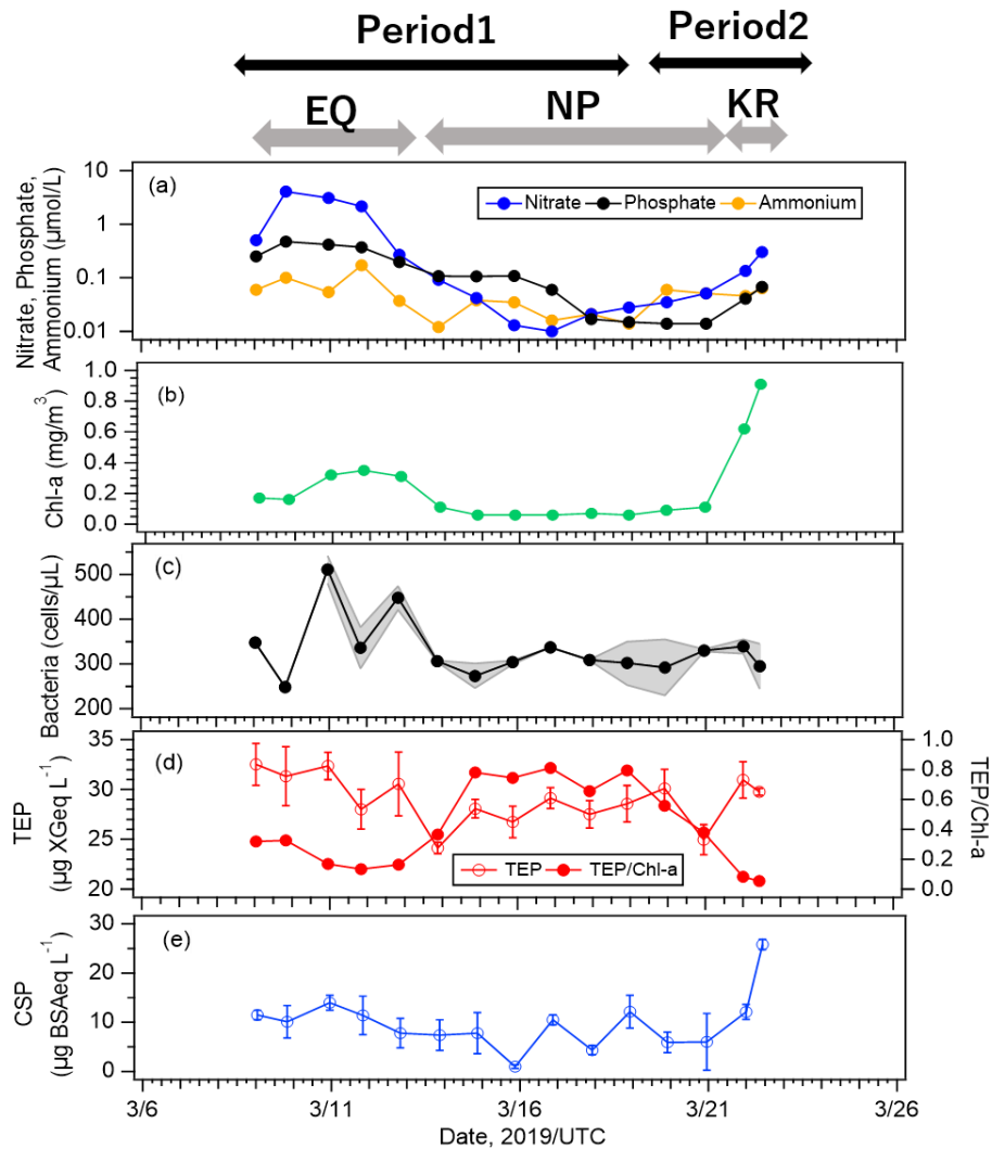
Figure 6. Time series of concentrations of (a) nutrients, (b) Chl- a , (c) bacteria, (d) TEPs and normalized TEP obtained by dividing TEP concentration by Chl- a concentration, and (e) CSPs at the South-Pacific subtropical region (SP) , equatorial upwelling region (EQ), North Pacific subtropical region (NP), and south of Kuroshio Extension (KR). The Y axis in Fig. 6a is displayed as logarithmic. The shade ranges in Fig. 6c are shown for samples where duplicate measurements were made. The error bars represent one standard deviation.
