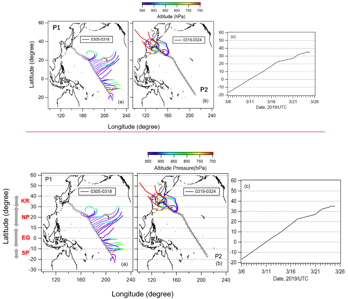
5 Figure 1. Five-day backward trajectories of air particles along with the cruise track initiated at twice a day (0600 and 1800 UTC of each day ) for (a) Period 1 (5–18 March 2019), and (b) Period 2 (19–24 March 2019). Open cycle markers represent the ship position during the observation. Color on trajectories show air parcel altitude. (c) Ship position during study period.
