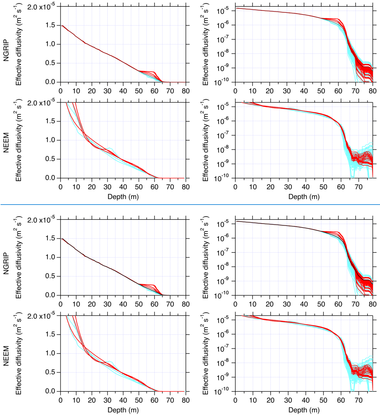
Figure 3: The 100 sets of effective diffusivity profile of CO 2 in the NGRIP (top panels, left panel on a linear scale and right panel on a log scale) and NEEM firn (bottom panels). The initial diffusivity profile (Ishijima et al., 2007) is shown in-by black dotted line
