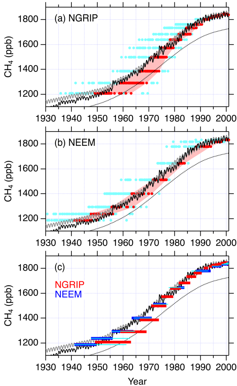
Figure 10: Results of reconstructions by the iterative dating method for the model cases with the 100 different diffusivity profiles (circles colored in the same manner as in Figures 3, 6 and 8) from the (a) NGRIP and (b) NEEM firn air, and (c) the ranges of reconstructions from both firn. The red shades indicate the range of \text{CH}_4 mole fraction trends reconstructed using the diffusivity profiles that better reproduce the trace gases except \text{CH}_4 . Black and grey solid lines are the atmospheric \text{CH}_4 scenarios of BZ and CMIP6, respectively, and black dotted line is the smoothed Antarctic \text{CH}_4 mole fraction (spline curve) from the Antarctic data shown in Figure 1. The thick horizontal bars in red and blue in panel c correspond to red shades in panels a and b. The light blue
