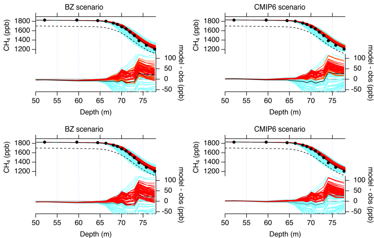
Figure 8: Same as Figure 6, but for CH 4 in the NGRIP firm . Simulation results with the atmospheric scenarios of BZ and CMIP6 are shown in left and right panels, respectively. The black dashed lines indicate the profiles calculated with the atmospheric scenarios for Antarctica (red line in Figure 2).
