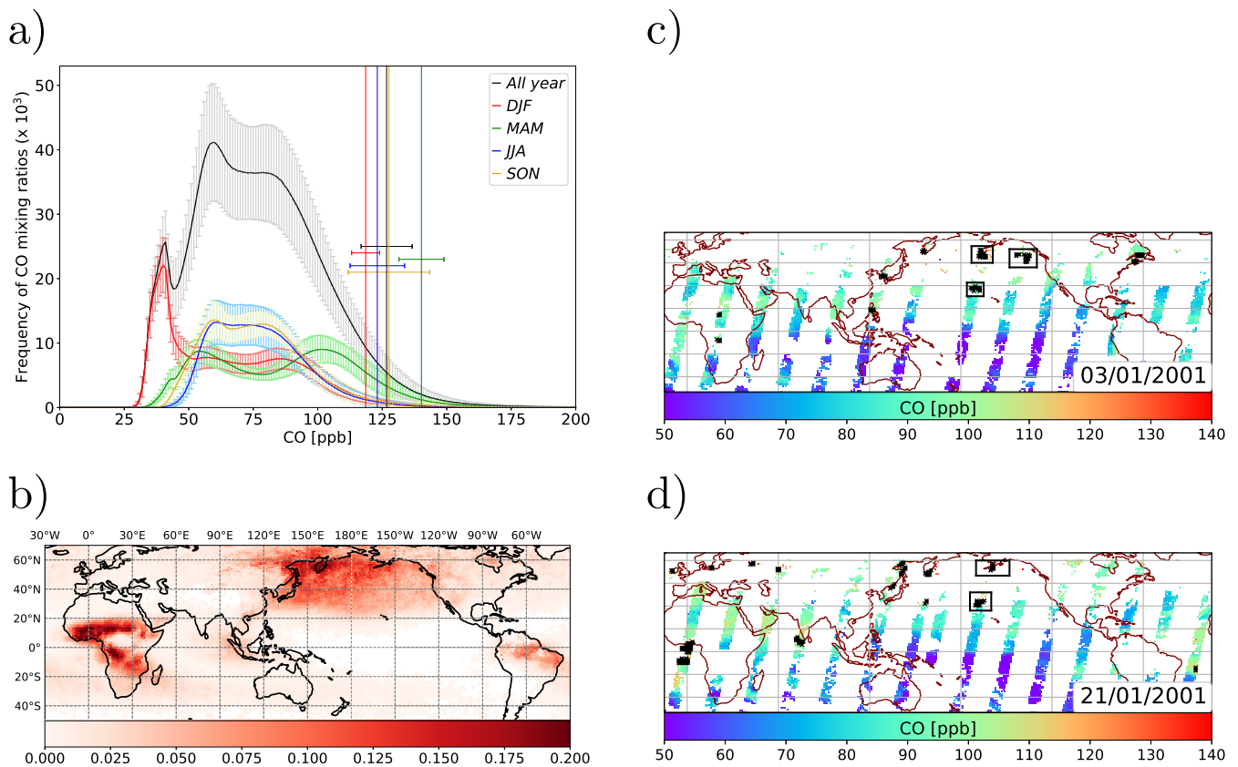
Figure 1. Fig. 1(a) shows the frequency distribution of mean CO mixing ratios [ppb] at 400hPa (years 2000–2019) as retrieved from MOPITT including the standard deviation. Vertical lines ranging from the bottom to the top of the plot denote the smallest (mean) mixing ratio, belonging to the highest 2% mixing ratios. Horizontal bars mark the standard deviation of this value. Fig. 1(b) shows the global frequency distribution (2000–2019) of the 2% data points (weighted with the total number of valid retrievals at each grid point).
