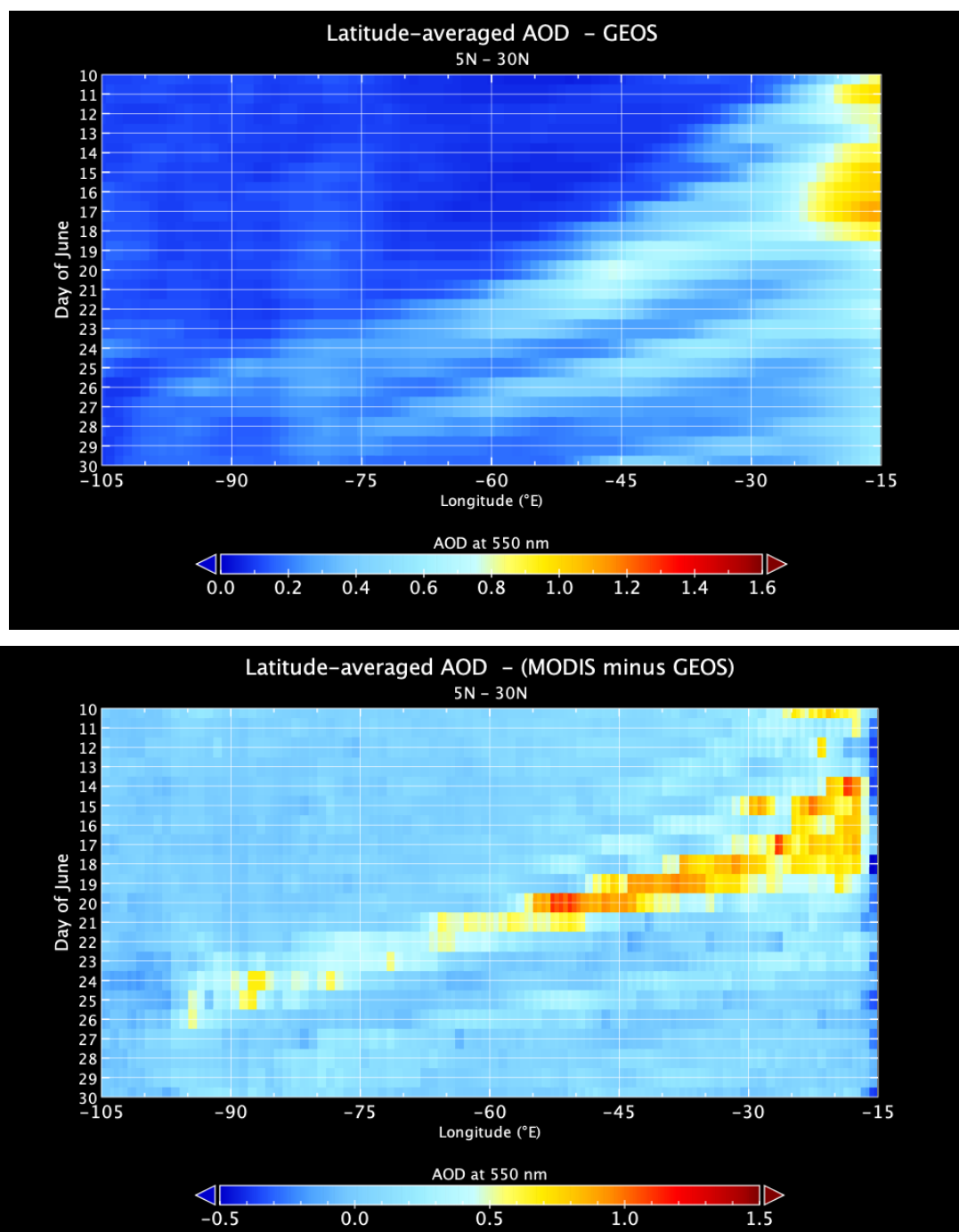
Figure 16: Time-longitude Hovmöller diagrams for GEOS latitude-averaged (5°N-30°N) AOD (top) and difference between MODIS and GEOS AOD (bottom).
