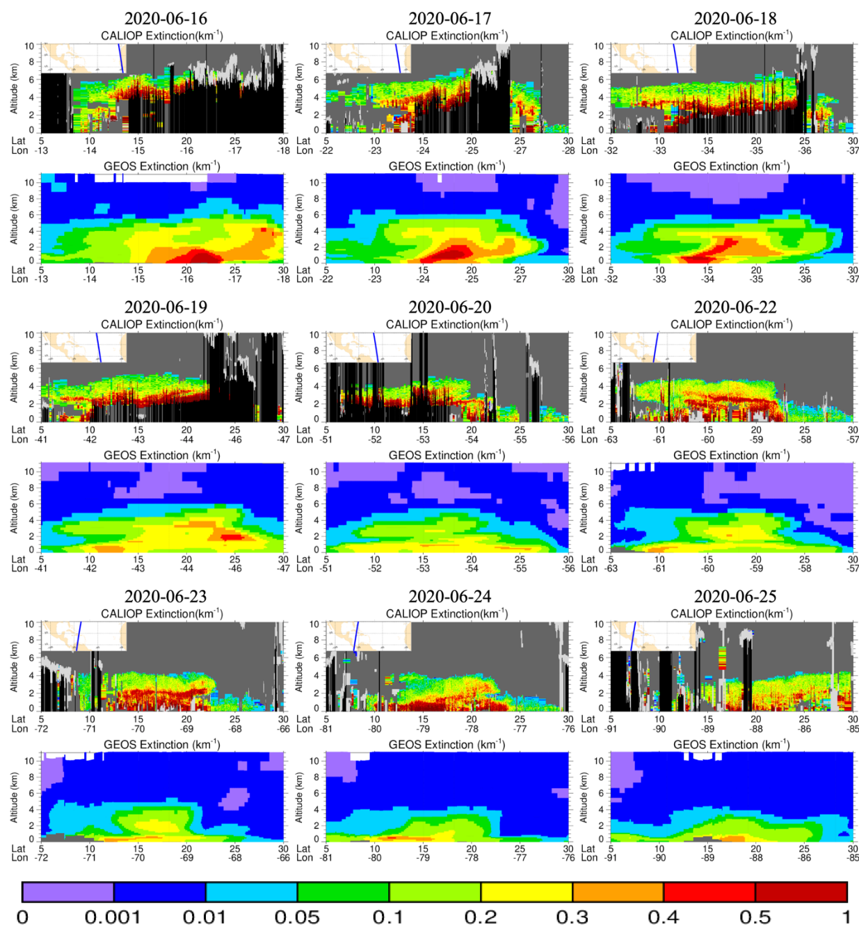
Figure 17: Comparison of altitude-latitude/longitude curtain of aerosol extinction coefficient ( \text{km}^{-1} ) between CALIOP (at 532 nm) and GEOS (at 550 nm) along the dust plume transit for 9 selected days. GEOS model outputs were sampled along the CALIPSO track shown as blue line overlying the geographical map (see insets). For CALIOP curtains, the cloudy scene, clear-clean scene, and totally attenuated feature is marked as light gray, dark gray, and black, respectively.
