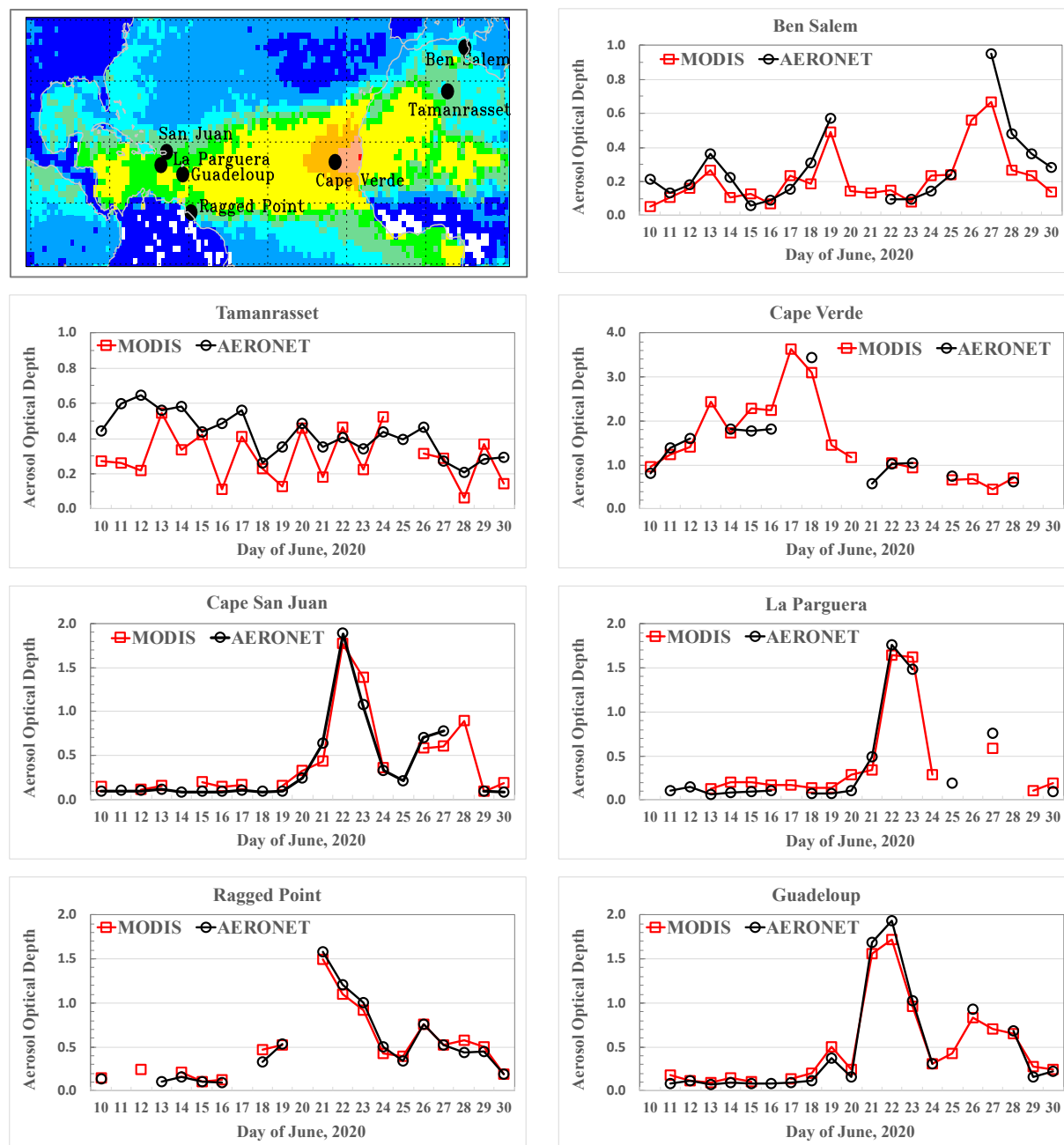
Figure 4: Time series of MODIS and AERONET daily AOD at 550 nm in seven AERONET sites from June 10 to 30, 2020.
