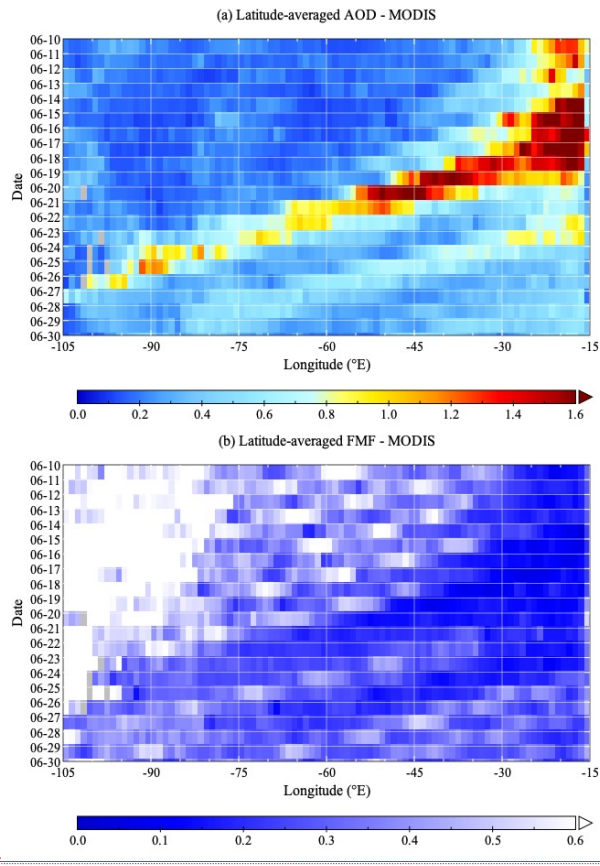
Figure 3: Tracks of trans-Atlantic dust plumes during June 10-30, 2020 as revealed in the longitude-time Hovmöller diagrams of MODIS daily AOD (top) and FMF (bottom). AOD and FMF are averaged over 5°N - 30°N.
