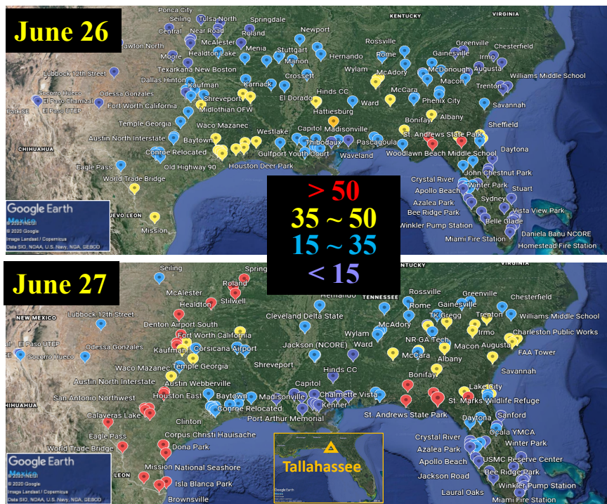
Figure 7: Observed \text{PM}_{2.5} concentrations at the EPA air quality network over southern U.S. on June 26 (top) and 27 (bottom), respectively. \text{PM}_{2.5} concentrations are categorized and marked with color into four ranges: <15 (purple), 15–35 (blue), 35–50 (yellow), and >50 (red) \mu\text{g m}^{-3} . Note that the EPA air quality standard for 24-hr \text{PM}_{2.5} is 35 \mu\text{g m}^{-3} . Location of Tallahassee is shown in inset of the June 27 map. The background maps are copyrighted by @Google Earth.
