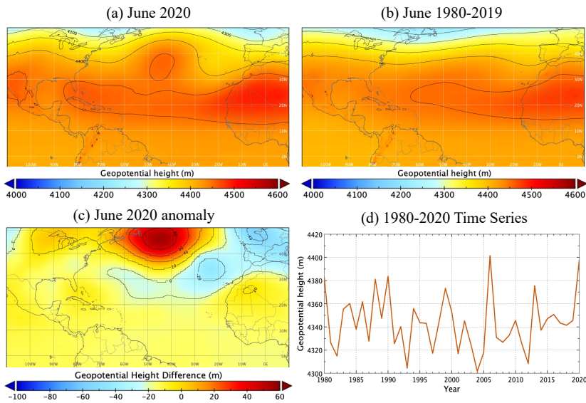
Figure 12: MERRA2 reanalysis geopotential height at 600 hPa: (a) June 2020, (b) June climatology (1980-2019), (c) June 2020 anomaly, and (d) 1980-2020 time series averaged over 35°N-50°N and 60°W-30°W.
