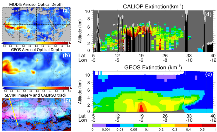
Figure 14: same as Figure 13 except for June 15, 2020.
