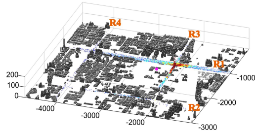
700 Figure 7: Density distribution of all trajectory points passing through the traffic roads that received from different receptor sites (S1, S2, S5, and S7, see details in Table 4). The four receptor sites are all marked with magenta dots.
