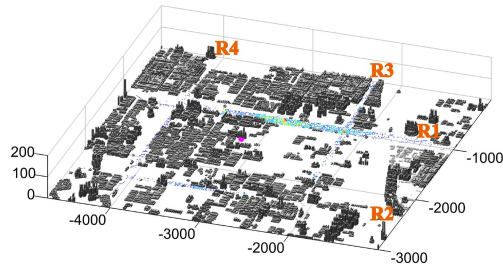
(c) Receptor site S5 (h = 15 m)
