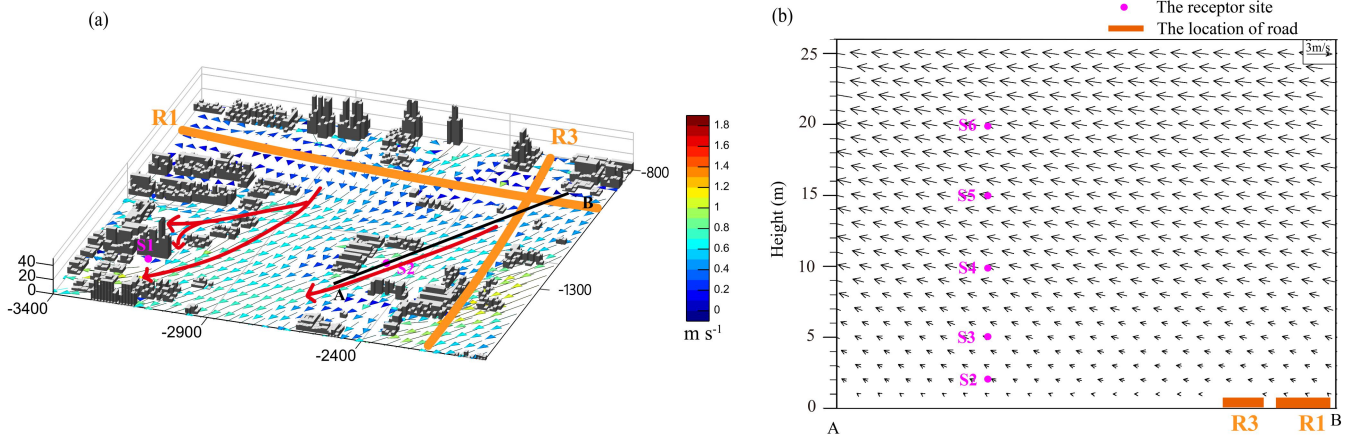
705 Figure 8: The (a) average surface wind and (b) vertical structure of average winds that along the wind direction around the receptor site S2 (line AB) in January 2019. The road R1 is marked with orange line; the location of the vertical profile is shown in black line, and the receptor sites S1 to S6 are all marked with magenta dots.
