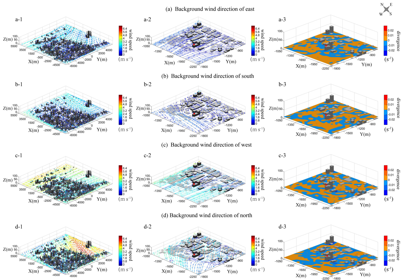
695 Figure 6: The wind field streamlines and divergences under the background wind directions of east (a), south (b), west (c) and north (d). The BSC monitoring site is marked with red dot.
