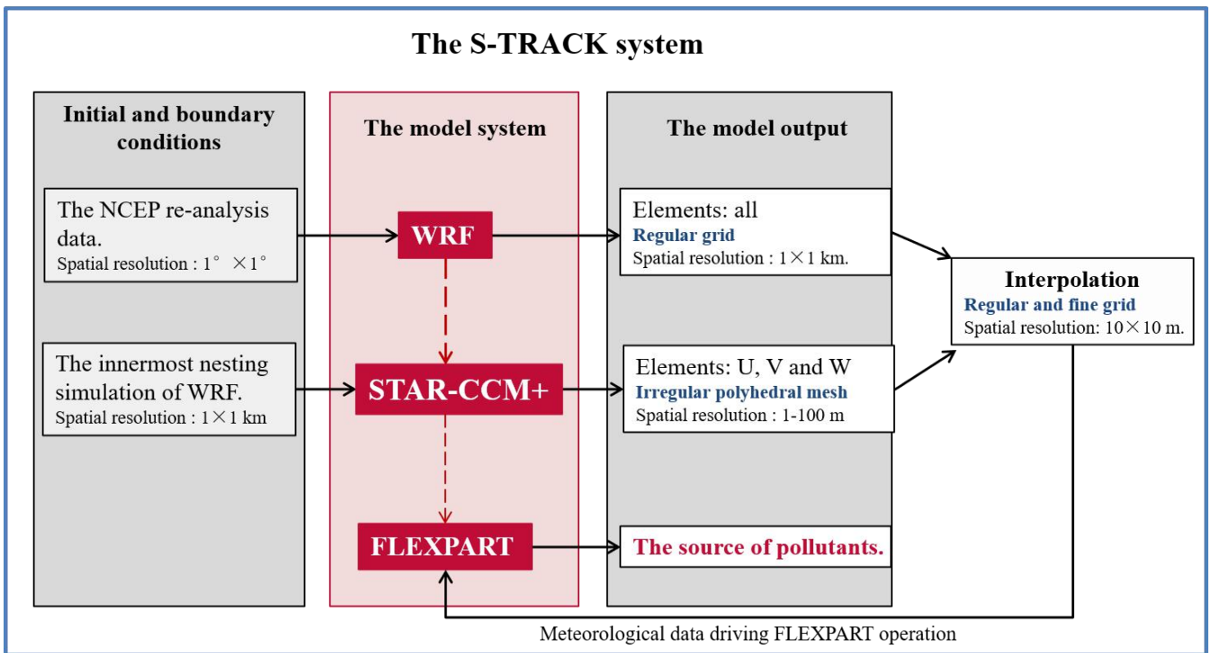
665 Figure 1: The S-TRACK system: The role of WRF, STAR-CCM+ and FLEXPART in the S-TRACK system and the process of gradual refinement of resolution.
