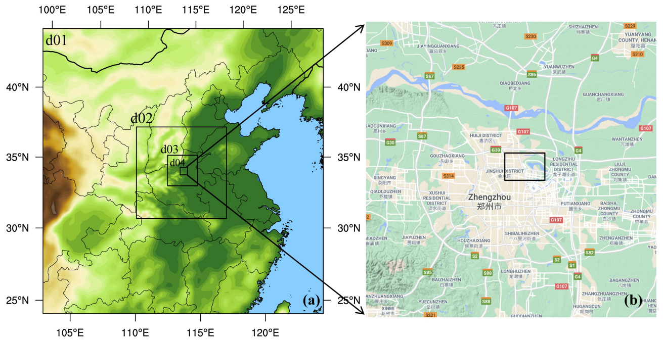
670 Figure 2: Domain configuration of the WRF model: (a) the range of the four nested domains (d1- d4); (b) the innermost nested domain (d4), within which the black box represents the STAR- CCM+ simulation domain (extracted from © Google Maps 2021).
