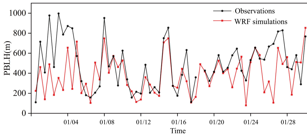
490 Figure A1. Time series of the observed (black) and simulated (red) PBLH at 8:00 and 20:00 Beijing time (BJT) in Zhengzhou sounding site.
