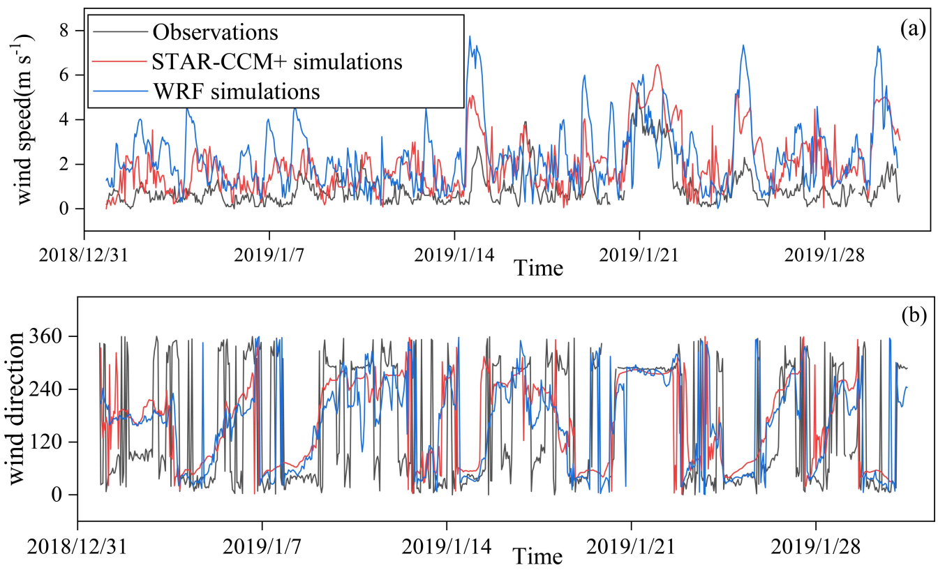
685 Figure 4: Evaluation of the wind simulation results at the BSC monitoring site (see in Fig. 3a): the simulated, by WRF (blue line) and STAR-CCM+ (red line) model, respectively, and the observed (grey line) hourly near-surface wind speeds (a) and wind directions (b).
