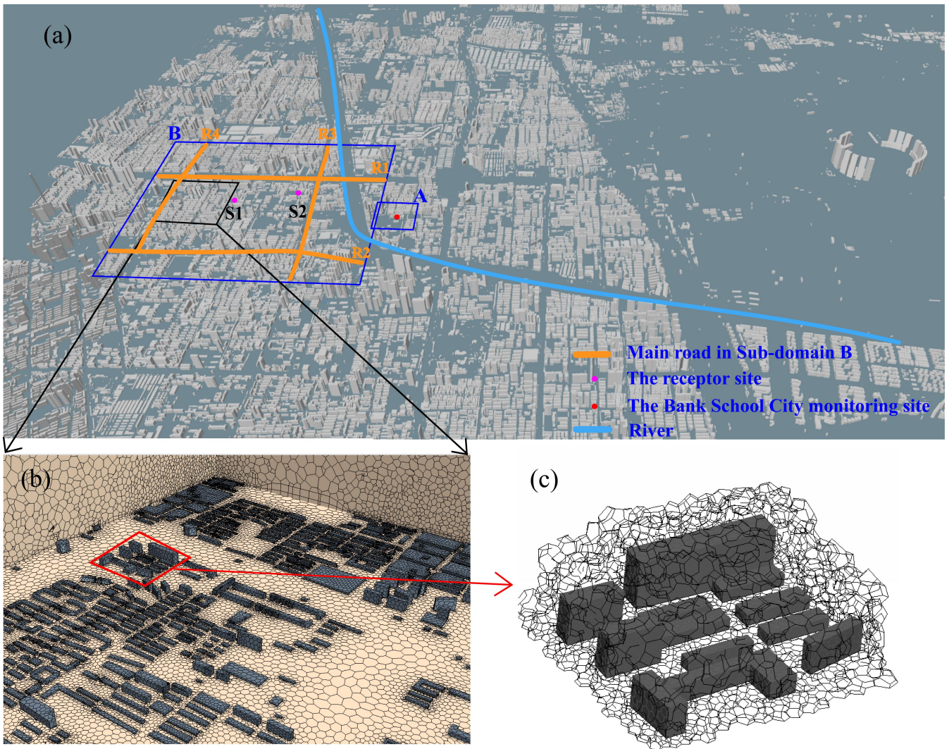
675 Figure 3: The computational domain of the STAR-CCM+ is shown in (a). The sub-domain A is used for detailed analysis of the wind environment, and the Bank School City (BSC) monitoring site is marked with the red dot. Sub-domain B is used to analyse the potential contribution of traffic source on receptor sites in the region, with magenta dots (S1 and S2) indicating the receptor sites and Orange line indicating the main roads. The polyhedral mesh is used to divide 680 the STAR-CCM+ simulation area. The mesh details of the vertical cross section and building surface are shown in (b), and the 3D meshes are shown in (c).
