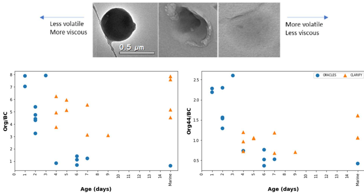
1000 Figure 3 Example of different viscosity/volatility organic aerosol (top panel) showing more round and viscous particles for ORACLES (on the left), and more volatile for CLARIFY (middle and right top panels) and Org/BC and Org44/BC ratios with time from fire source (bottom panel)
