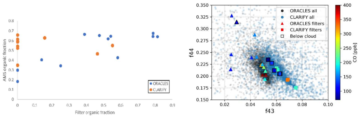
995 Figure 2 (left) AMS organic fraction vs filter organic fraction and (right) f44 vs f43 space for ORACLES and CLARIFY campaigns with filters marked as triangles for ORACLES and squares for CLARIFY. Colors of the marks denoting filter sampling represent CO concentration, as shown in the colorbar. Samples collected below-cloud are outlined with a black border.
