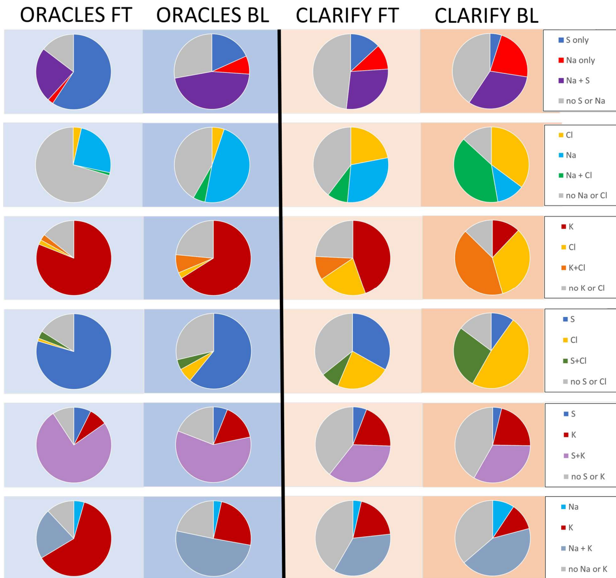
1065 Figure 10 Elemental mixing states for select elemental pairs for ORACLES (two left columns) and CLARIFY (two right columns), separated by filter collection in the free troposphere and boundary layer
