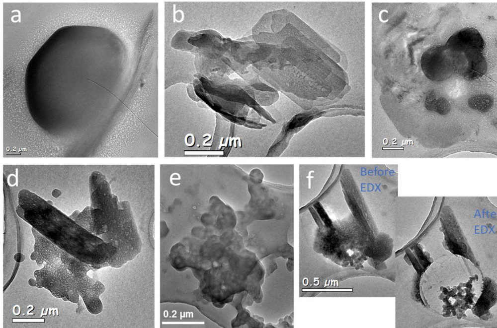
1020 Figure 6 Assorted sea salt particles. (a) ~1.5 micron rounded NaCl; Gold 1 (b) CaSO 4 ; Gold 1 (c) NaCl and Mg; Gold 1 (d) Na 2 SO 4 with K; Gold 1 (e) NaNO 3 mixed with BC; Gold 24 (f) BC encapsulated in Na 2 SO 4 with K ; Gold1
