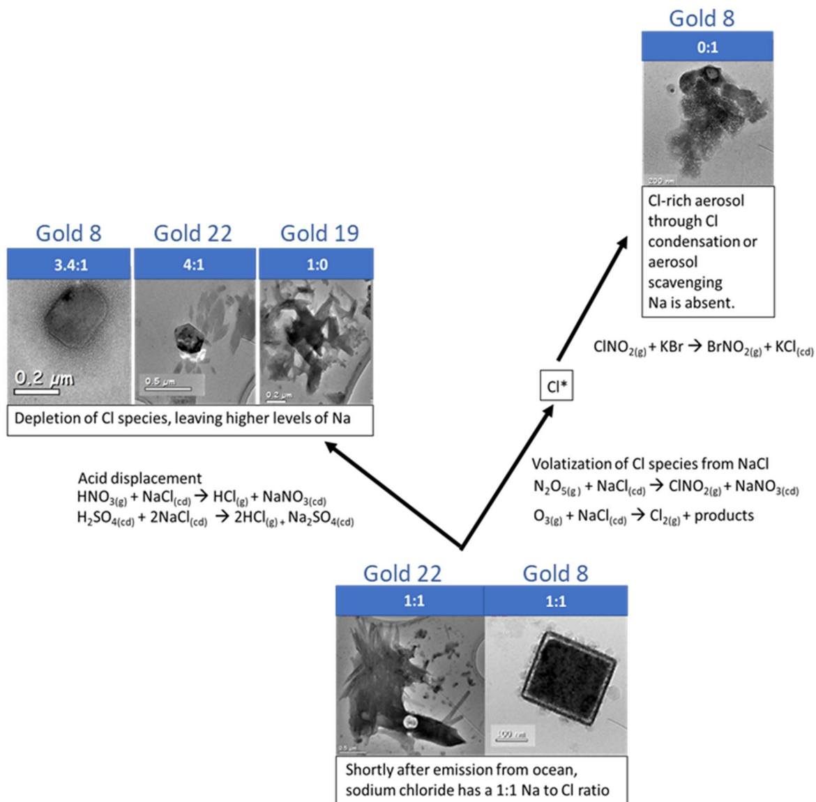
1015 Figure 5 Schematic showing different stages of sea salt conversion with example mechanisms. The particles are from CLARIFY filters and range from sea salts which have been freshly emitted to Cl-depleted particles containing nitrates and sulfates. Cl aerosol formation is also shown. Na:Cl ratios showing depletion of Cl with sea salt conversion are shown in the bar above each particle image.
