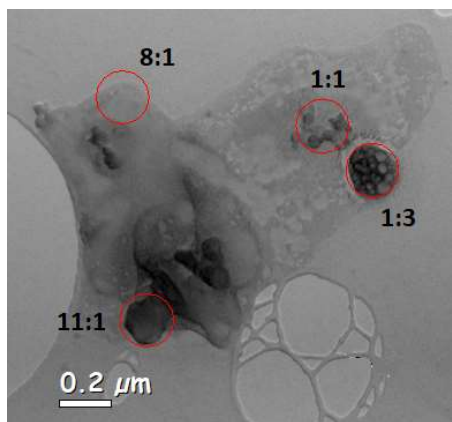
1055 Figure 8 Aqueous K-salt particle with varying levels of Na throughout particle, with Na:K weight ratio designated in red
