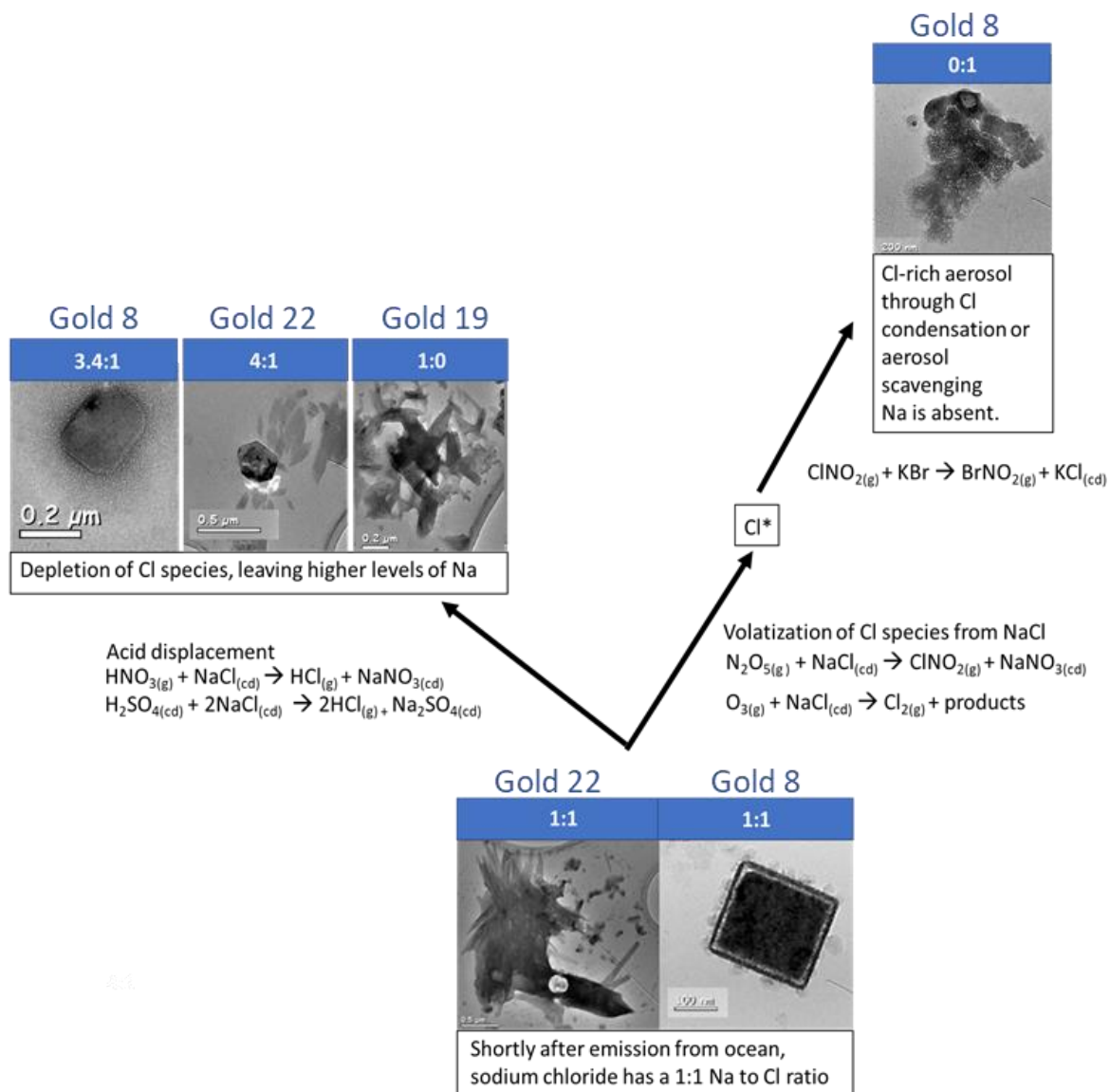
995 Figure 5 Schematic showing different stages of sea salt conversion with example mechanisms. The particles are from CLARIFY filters and range from sea salts which have been freshly emitted to Cl-depleted particles containing nitrates and sulfates. Cl aerosol formation is also shown. Na:Cl ratios showing depletion of Cl with sea salt conversion are shown in the bar above each particle image.
