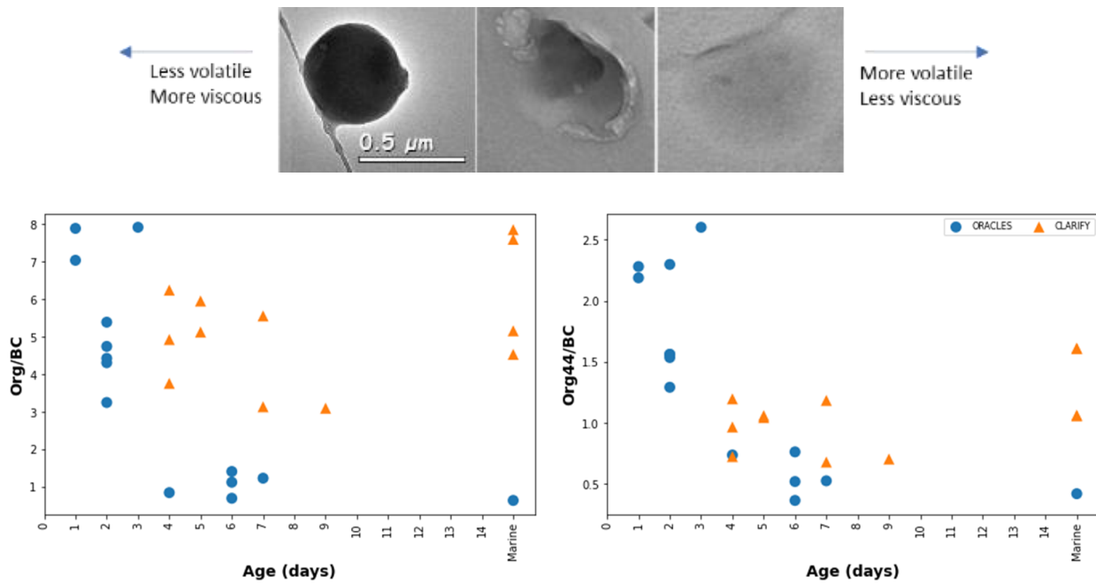
980 Figure 3 Example of different viscosity/volatility organic aerosol (top panel) showing more round and viscous particles for ORACLES (on the left), and more volatile for CLARIFY (middle and right top panels) and Org/BC and Org44/BC ratios with time from fire source (bottom panel)
