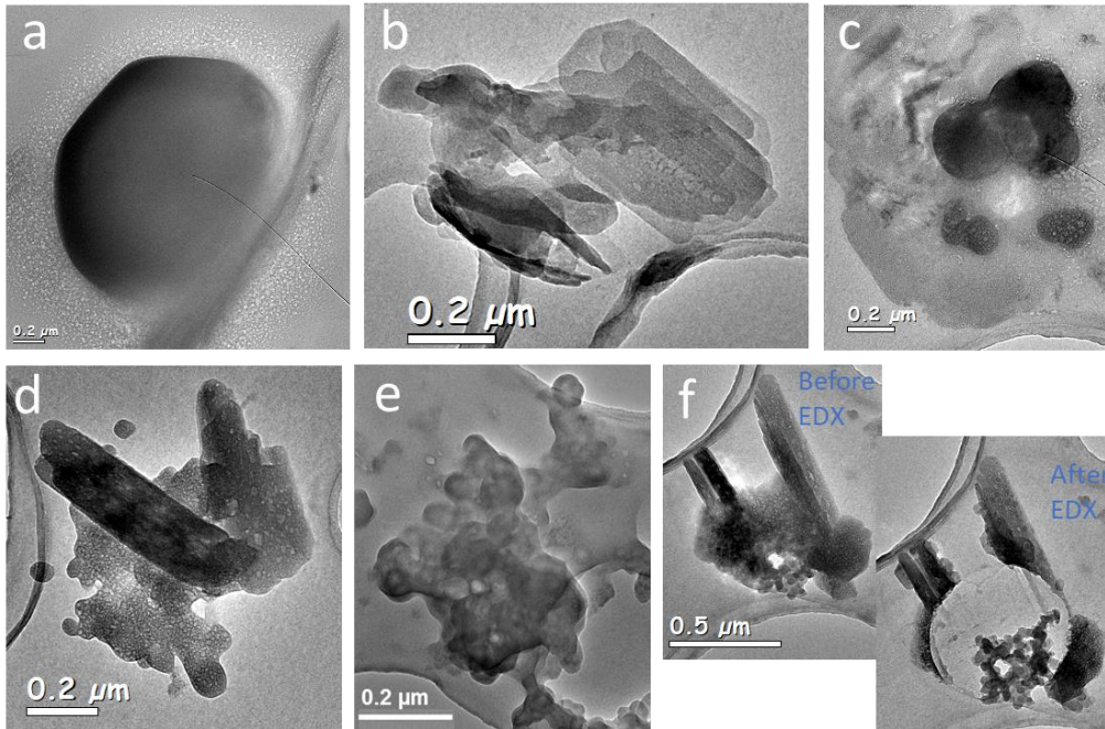
1000 Figure 6 Assorted sea salt particles. (a) ~1.5 micron rounded NaCl; Gold 1 (b) CaSO 4 ; Gold 1 (c) NaCl and Mg; Gold 1 (d) Na 2 SO 4 with K; Gold 1 (e) NaNO 3 mixed with BC; Gold 24 (f) BC encapsulated in Na 2 SO 4 with K ; Gold1
