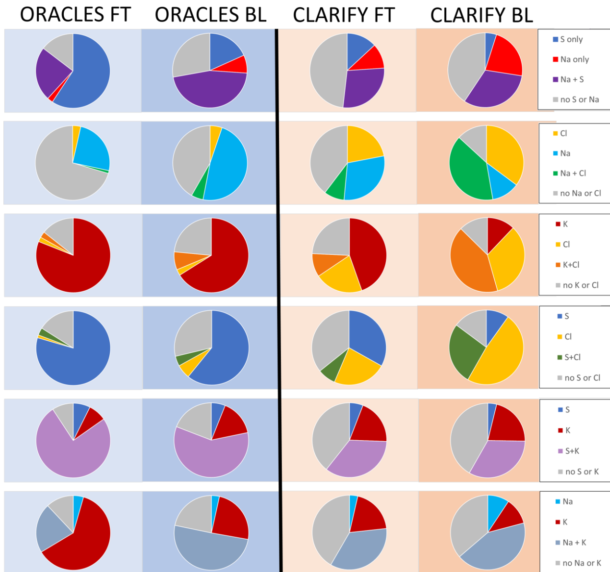
1045 Figure 10 Elemental mixing states for select elemental pairs for ORACLES (two left columns) and CLARIFY (two right columns), separated by filter collection in the free troposphere and boundary layer
