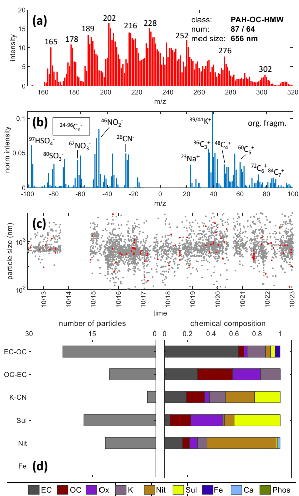
Figure 8: High molecular weight organics in addition to PAH peaks are frequently associated with fragments from oxidized OC (e.g. ^{43}\text{C}_2\text{H}_3\text{O}^+ ) and high sulfate signals. This supports the promoted SOA formation and oligomerization in acidic particles. Note also the cluster with dominating HMW-OC and high sulfate signals in Fig. S5. (For figure explanation, see Fig. 5.)
