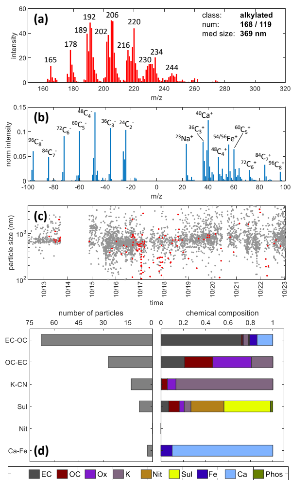
Fig. 9: Particles with dominant signals from alkylated phenanthrenes were observed during onshore wind periods. These rather small particles reveal soot and \text{Ca}^+ , but nearly no secondary material. They can be attributed to ship traffic with distillate fuels such as marine gas oil. (For figure explanation, see Fig. 5.)
