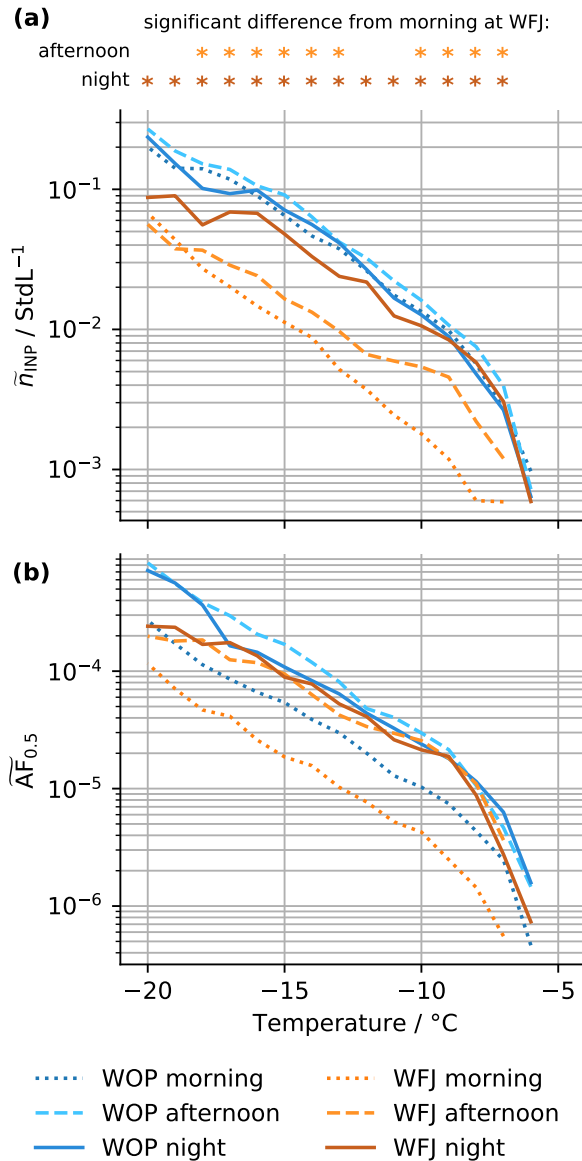
Figure 5. Median (cumulative) INP concentrations \tilde{n}_{INP} (a) and median activated fractions \tilde{AF}_{0.5} (b) for mountaintop (WFJ, orange) and high valley (WOP, blue) site for the three time periods of the day: Morning period (03:00 - 11:59 UTC) in dots, afternoon period (12:00 - 17:59) in dash and night period (18:00 - 02:59 UTC) in solid (see dotted lines in Figure 4b and 4c). Above panel (a), stars indicate if the median INP concentration at WFJ in the afternoon and night, respectively, is significantly (significance level p < 0.05 ) different from in the morning based on a Mann–Whitney U test per temperature.
