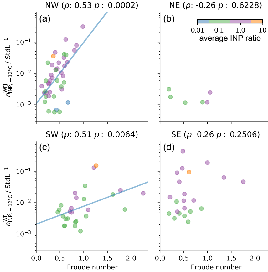
Figure 7. INP concentration at -12\text{ }^{\circ}\text{C} at WFJ ( n_{\text{INP}, -12^{\circ}\text{C}}^{\text{WFJ}} ) as a function of Froude number (see Equation 4) for the four meso-scale mesoscale wind direction sectors (as indicated in Figure 1). For each subplot the Spearman's rank coefficient ( \rho ) and the corresponding two-sided p-value ( p ) are shown at the top. The colors of the dots indicate the average INP ratio between WFJ and WOP (to assess the similarity of the INP concentration of both sites) as defined in Equation 5. Lines are exponential fits in case |\rho| \geq 0.5 .
