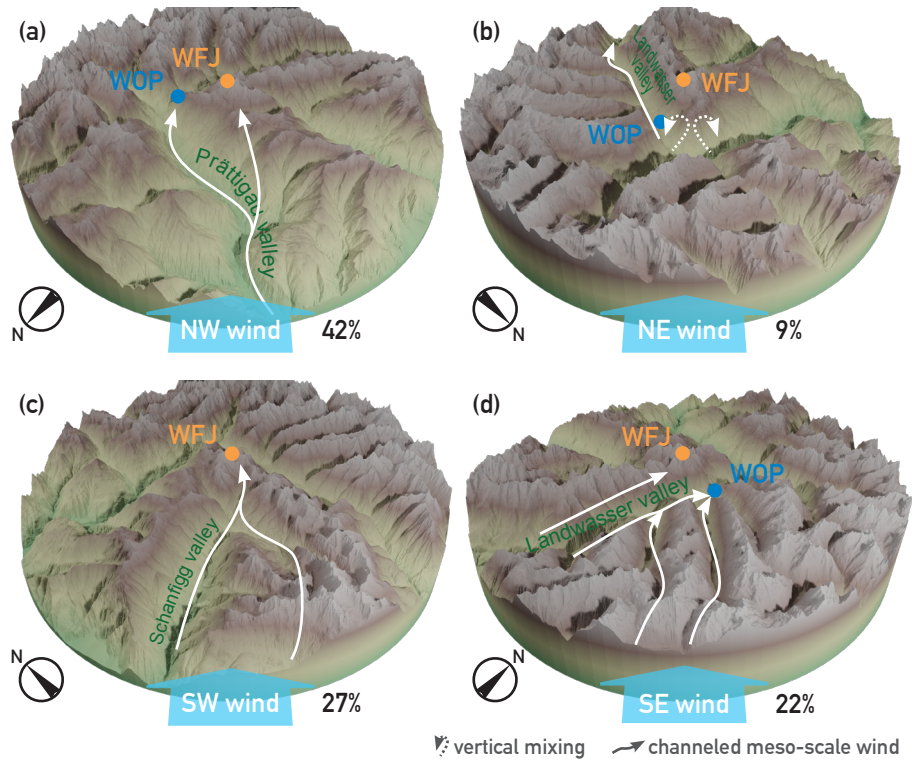
Figure 6. Channeled winds in the valleys (solid white arrows) of the meso-scale-mesoscale winds (light blue arrows) for the topography around the two measurement sites (WFJ: orange dot, WOP: blue dot) within a radius of 20 km around WFJ for the four wind direction sectors (as defined in Figure 1). The viewpoint in each panel is aligned with the meso-scale-mesoscale wind direction, is centered on WFJ (2693 m a.s.l.), and reaches down to an elevation of 500 m a.s.l.. The percentage of INP samples collected for each wind sector is indicated in the lower right of each subplot. In the NE wind case (b), the potential vertical mixing ( i.e. rising of air masses originating from the valley and mixing with the air masses aloft ) due to conditional instability of the narrow cross valley air masses is shown (dashed white arrows). The elevation data was obtained from the digital height model DHM2 from the Federal Office of Topography swisstopo.
