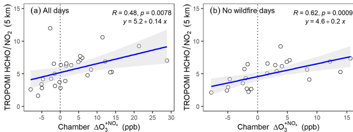
900 Figure 8. Ordinary least squares (OLS) regression between weekly averaged TROPOMI HCHO/ NO_2 at 5 km circular buffers and the weekly averaged \Delta O_3^{+NO_x} from ground-based measurement. The shaded area shows the 95% confidence interval of the mean response of the predicted value.
