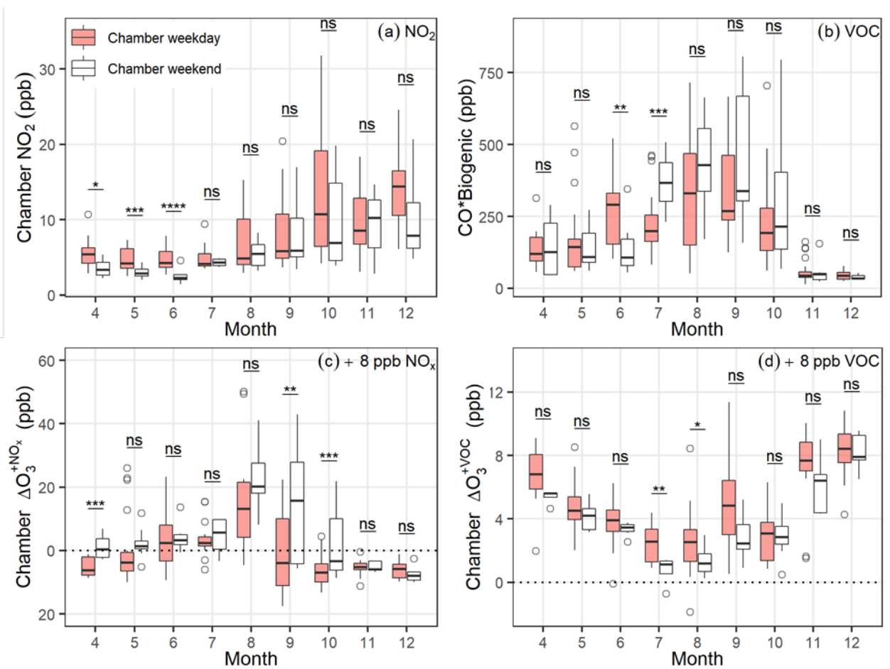
Figure 4 . Weekday (solid box) and weekend (open box) monthly-average concentrations of NO 2 and CO*biogenic (panels a, b), and \Delta O_3^{+NO_x} and \Delta O_3^{+VOC} (panels c, d) from April to December, 2020 after removing wildfire days. The stars above each box and whisker plot represent the significance of the weekday vs weekend difference. (*: p value < 0.1, **: p value < 0.05, ***: p value < 0.01, ****: p value < 0.001, ns (not significant): p value >= 0.1)
