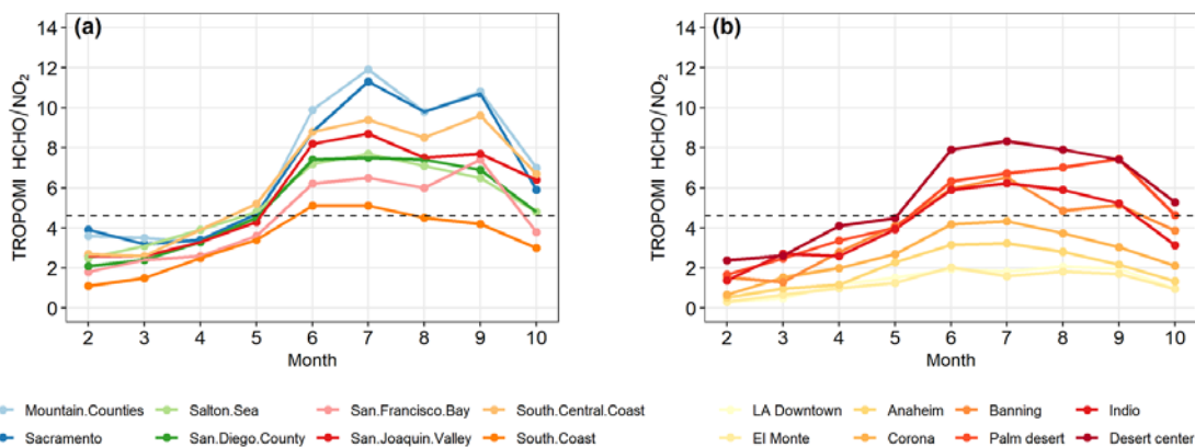
910 Figure 10. Monthly variation of TROPOMI HCHO/NO 2 in different air basins (left panel) and in different cities in Southern California (right panel). The darker colors in the right panel indicate increasing distance from the urban center of Los Angeles.
