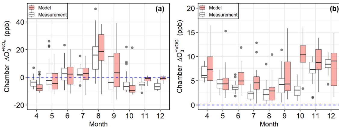
915 Figure 11. Monthly variation of the ΔO 3 +NO x (a) and ΔO 3 +VOC (b) predicted by the chamber model (solid box) and directly measured in the chamber (open box) from April to December, 2020 at the Sacramento measurement site.
