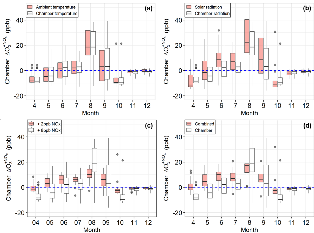
920 Figure 12. Effect of temperature, radiation, and perturbation amount on the monthly variation of the predicted chamber \Delta O_3^{+NO_x} from April to December, 2020 at the Sacramento measurement site. Open boxes show the predicted response under chamber measurement conditions (chamber temperature, radiation, and 8ppb NO 2 perturbation). Solid boxes show the predicted response when conditions are updated: (a) using the ambient temperature profile; (b) using clear-sky solar radiation; (c) using a 2 ppb NO x perturbation; (d) using the combination of ambient temperature, solar radiation, and 2ppb NO 2 perturbation.
