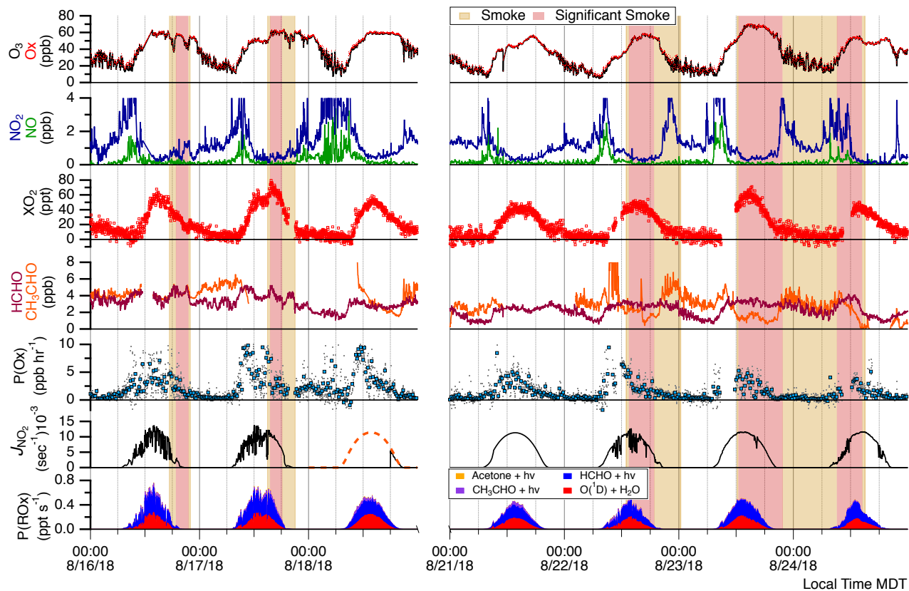
340 Figure 3 Time-series of O_3 , NO , NO_2 , total peroxy radicals ( XO_2 ), and aldehydes ( HCHO and CH_3CHO ). Modeled J_{NO_2} frequencies and calculated parameters of P(Ox) and P(ROx) are also provided. The red shading indicates periods of smoke influence, while somewhat smoky periods are shaded tan. P(Ox) is shown in both 16-minute averages (blue circles) and 2-minute data (grey points). The dashed J_{NO_2} trace is entirely simulated by NCAR TUV model whereas the rest of the data is derived from ARISense solar irradiance measurements.
