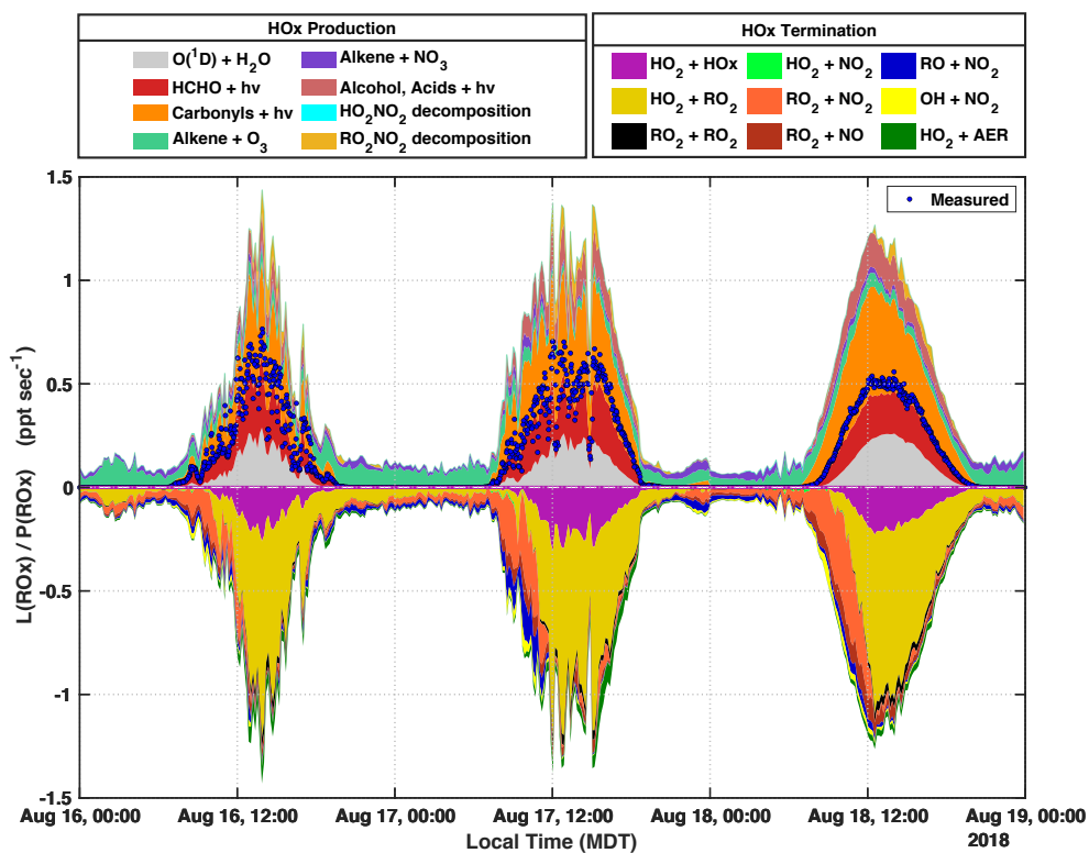
Figure 8 Modeled ROx production and termination for 16, 17, and 18 August. The results provided were modeled with F0AM using the MCM-BBVOc-het mechanism. Net rates are provided for reversible processes. ROx termination L(\text{ROx}) and ROx production P(\text{ROx}) are separated into several straightforward categories as represented in their respective legends. Heterogeneous \text{HO}_2 loss is represented by the \text{HO}_2 + \text{AER} category. P(\text{ROx}) derived from direct measurements, as presented in Fig. 3, is shown for comparison and is represented by the blue markers. The modeled results are shown in 10-minute intervals and were averaged from the 2-minute basis, while measurement-based P(\text{ROx}) is shown in 2-minute intervals.
