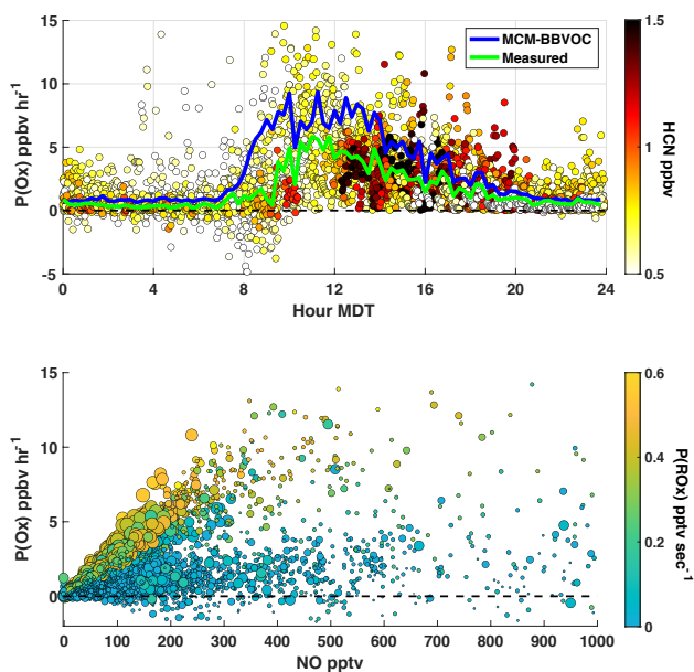
425 Figure 5 P(Ox) results derived from 2 min \text{XO}_2 observations. Panel A shows the diurnal profile of all calculated P(Ox) values. The data points are colored by smoke tracer HCN. The green and blue traces represent 15-minute median values of P(Ox) as determined using measurements and model results, respectively. The provided model results were acquired with FOAM using the MCM-BBVOC mechanism. Panel B shows the variation of P(Ox) with NO. Data is colored by P(ROx) and sized by [HCN].
