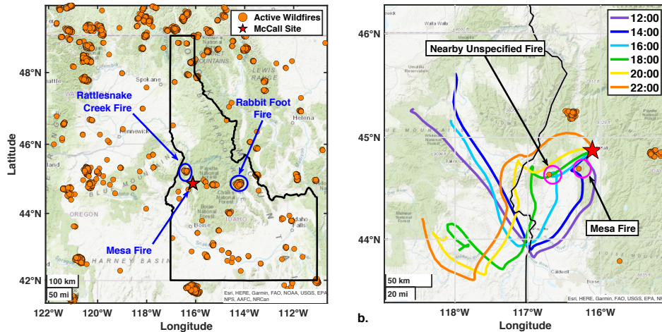
265 Figure 1 The McCall, Idaho site is indicated by the red star and wildfire locations indicated by orange circles. Panel A shows detected wildfires between 15 August 2018 and 24 August 2018. Panel B includes bihourly HYSPLIT back trajectories for the representative smoke impacted day of 17 August. Shown here are active wildfires of 15 August through 17 August, as back trajectories end 24 hours back. Fire locations were retrieved using the NOAA Hazard Mapping System (HMS) (NOAA, 2021).
