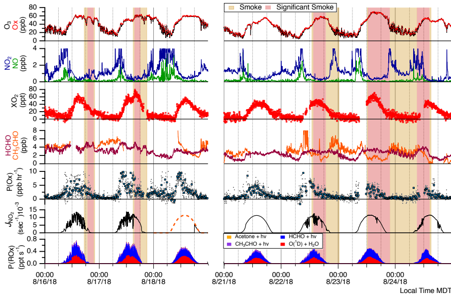
Figure 3 Time-series of O_3 , NO , NO_2 , total peroxy radicals ( XO_2 ), and aldehydes ( HCHO and CH_3CHO ). Modeled J_{NO_2} frequencies and calculated parameters of P(Ox) and P(ROx) are also provided. The red shading indicates periods of smoke influence, while somewhat smoky periods are shaded tan. P(Ox) is shown in both 16-minute averages (blue circles) and 2-minute data (grey points). The dashed J_{NO_2} trace is entirely simulated by NCAR TUV model whereas the rest of the data is derived from ARISense solar irradiance measurements.
