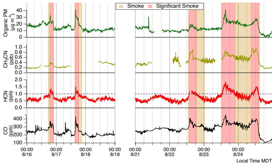
270 Figure 2 Time series of smoke tracers. Tan shading represents smoke presence, while red shading signifies significant smoke periods. Significant smoke periods are defined by HCN concentrations greater than 1 ppbv. This smoke-defining concentration is indicated by the purple dashed line.
