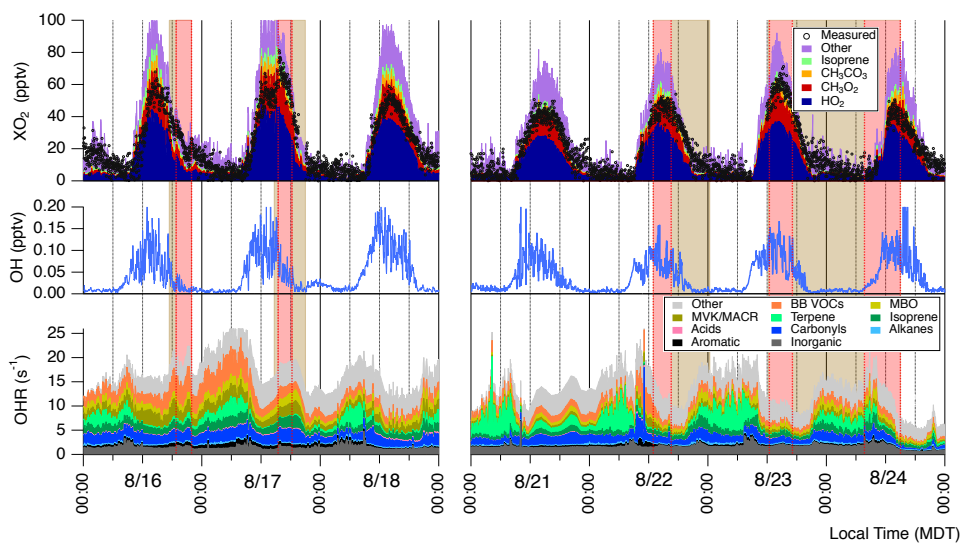
460 Figure 6 Time series of modeled OH, HO 2 , speciated RO 2 , and OH reactivity (OHR). These results were acquired using the MCM-BBVOC mechanism. Periods of smoke are shaded as per Fig. 2. Measured XO 2 is included as black markers for comparison. Legend categories for XO 2 and OHR are mostly straightforward. Note that the isoprene XO 2 category includes several RO 2 species produced from isoprene oxidation.
