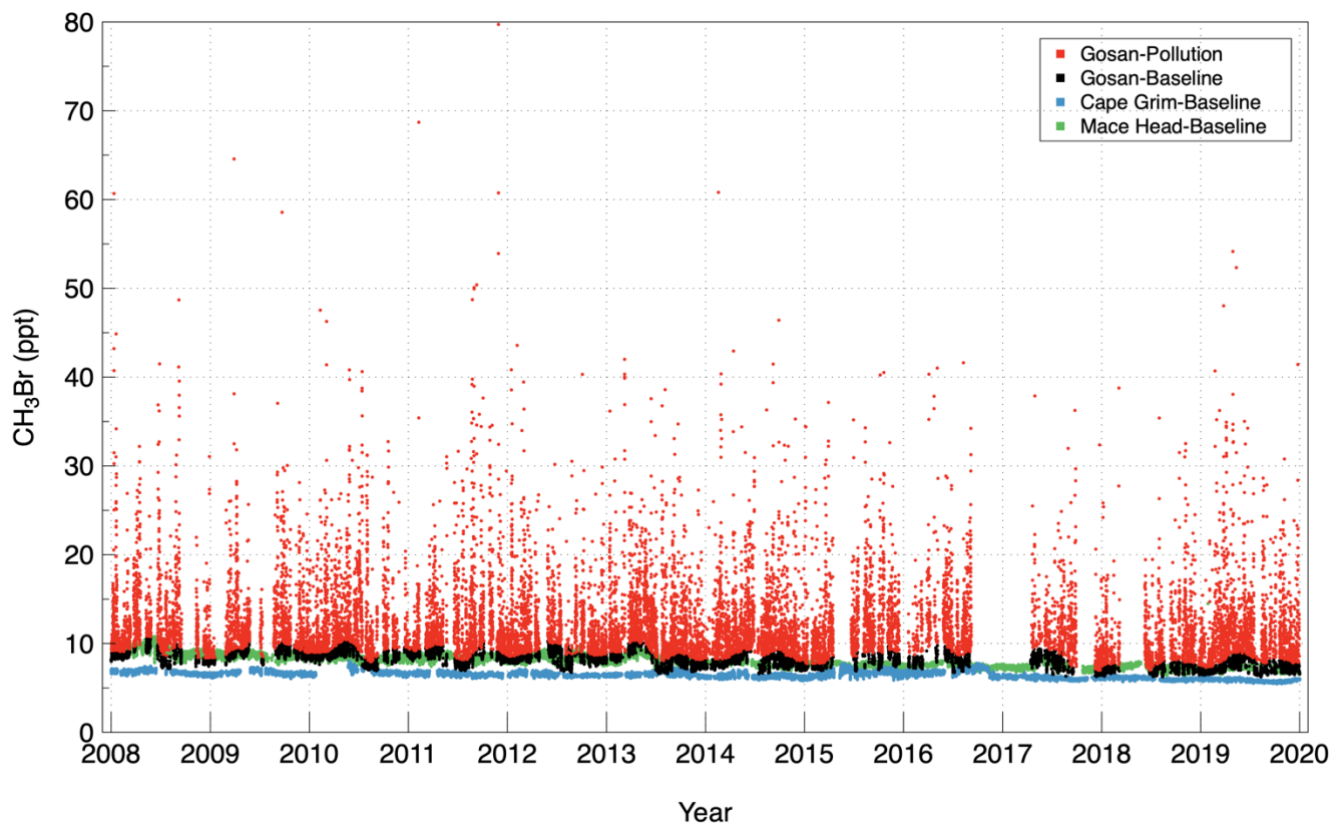
635 Figure 2: Mole fractions of \text{CH}_3\text{Br} in the atmosphere at Gosan for the period 2008–2019. The baseline data (black) are selected using a statistical method (O’Doherty et al., 2001); the polluted data (red) are elevated above the baseline data. The baseline data from Mace Head, Ireland (green) and Cape Grim, Australia (blue) over the same period are shown as mid-latitude references for the Northern and Southern Hemisphere, respectively.
