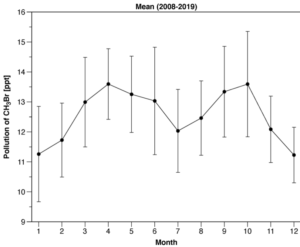
100 Figure S5: Monthly mean of polluted concentrations of CH 3 Br at Gosan from 2008 to 2019. Error bars represent the standard deviation of each month.
