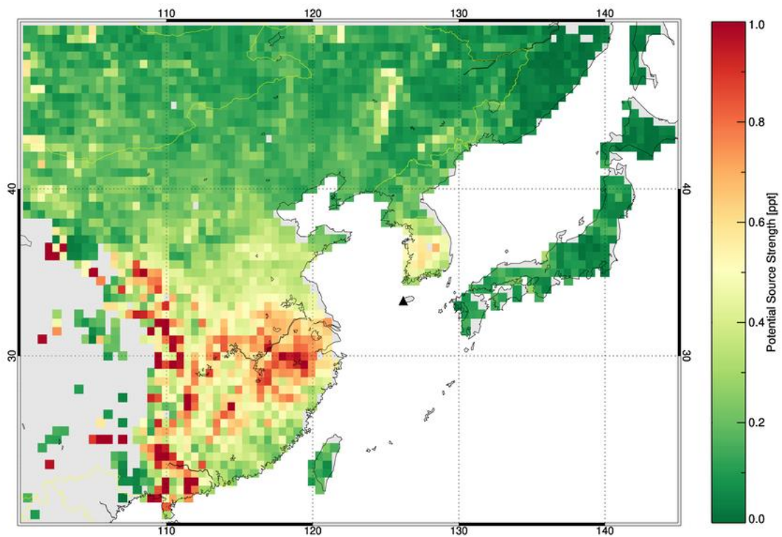
105 Figure S6: Potential source regions derived from back-trajectory analyses of SO 2 F 2 pollution data at Gosan from 2008 to 2019. The location of Gosan station is represented as a black triangle.
