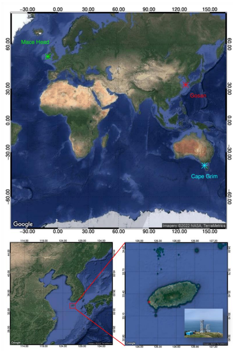
Figure 1: Gosan station (33.3° N, 126.9° E, 72 m a.s.l.) on Jeju island, Korea (red asterisk). Air samples are taken at 17 m (~100 m a.s.l.) from a tower next to the coastal cliff. The geographic locations of Ireland's Mace Head (53.3°N, 9.9°W) and Australia's Cape Grim (40.7°S, 144.7°E), representative the remote background monitoring station in Northern and Southern Hemispheres, are indicated by green and blue asterisk, respectively. (Map data: © Google Earth)
