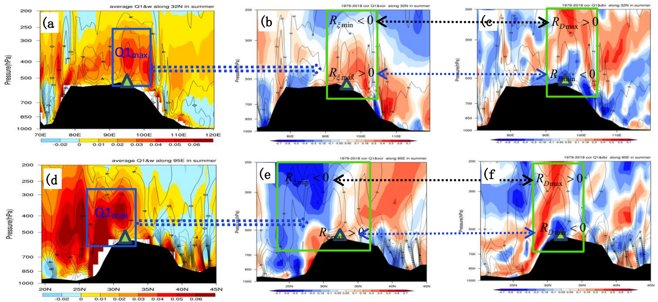
Figure 4. The vertical sections of vertical motion (contours, in unit: 10^{-2}\text{Pa}\cdot\text{s}^{-1} ) and average Q1 (shaded, in unit: 10^{-3}\text{w/kg} ) (a,d) ; vertical motion (contours, in unit: 10^{-2}\text{Pa}\cdot\text{s}^{-1} ) and correlation coefficients (shaded) between Q1 and the vorticity (b,e) as well as the correlation coefficients between Q1 and the divergence (c,f) separately in the core region of the AWT, in which, a, b, c is along 32^\circ\text{N} , and d, e, f is along 95^\circ\text{E} . The green triangle is the AWT.
